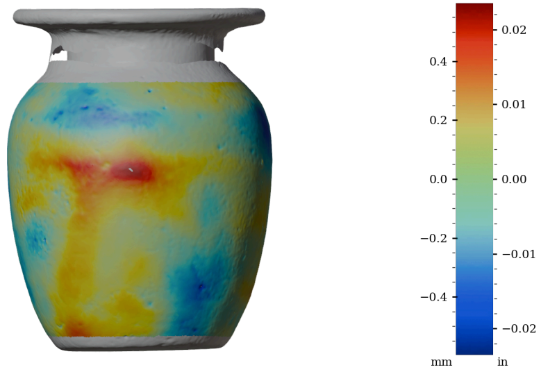
Figure 47: Surface variability heatmap of HV005, rotated 180°
