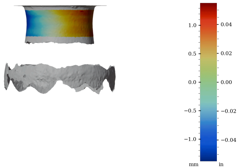
Figure 52: Surface variability heatmap of HV005, rotated 270°
