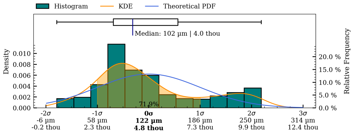
Figure 42: Coaxiality residual plots of exterior surface, HV005.
