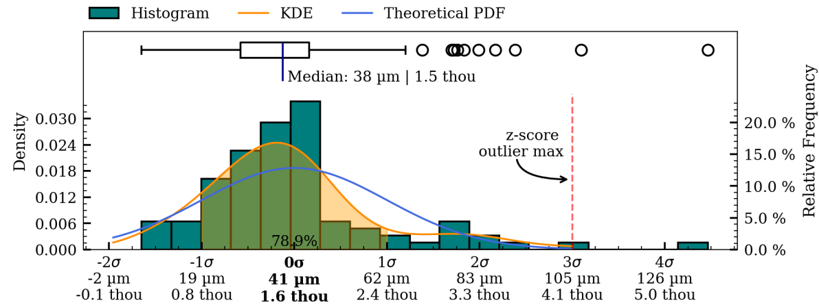
Figure 43: Coaxiality residual plots of interior surface, HV005.
