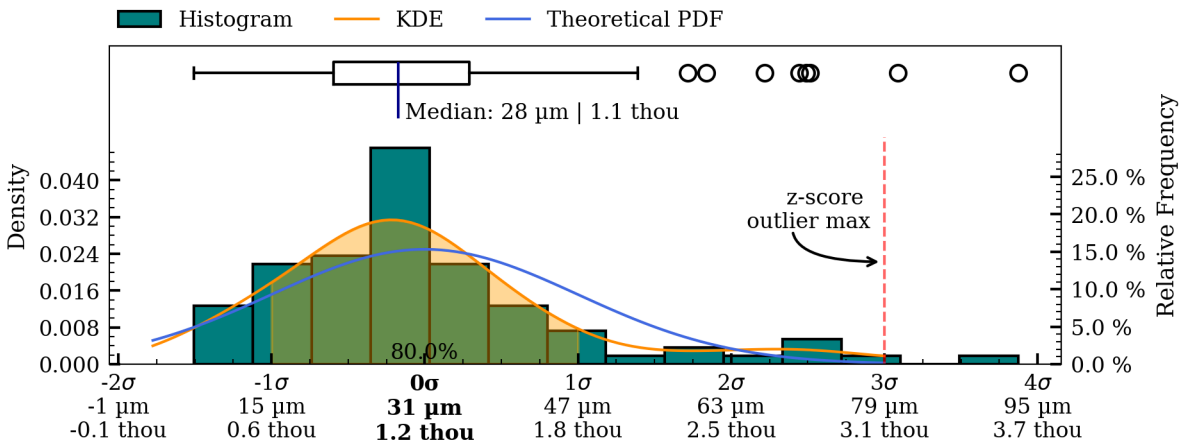
Figure 44: Coaxiality residual plots of interior_separate surface, HV005.
