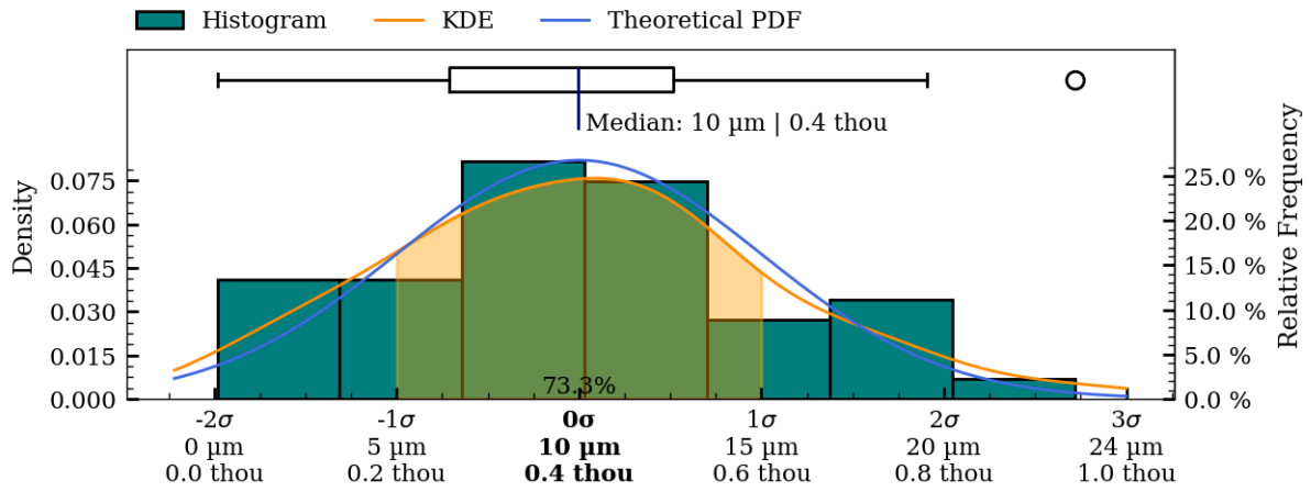
Figure 43: Coaxiality residual plots of interior surface, IV009.
