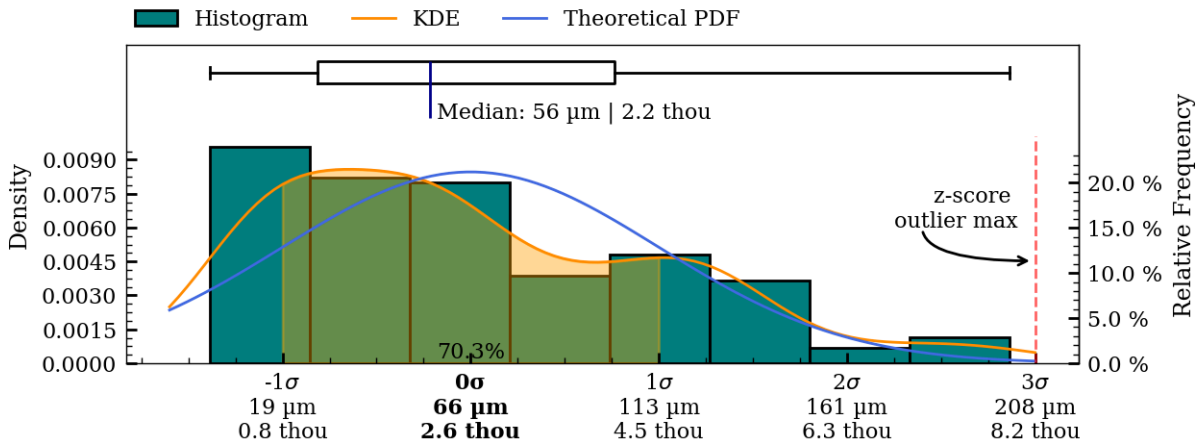
Figure 42: Coaxiality residual plots of exterior surface, IV009.
