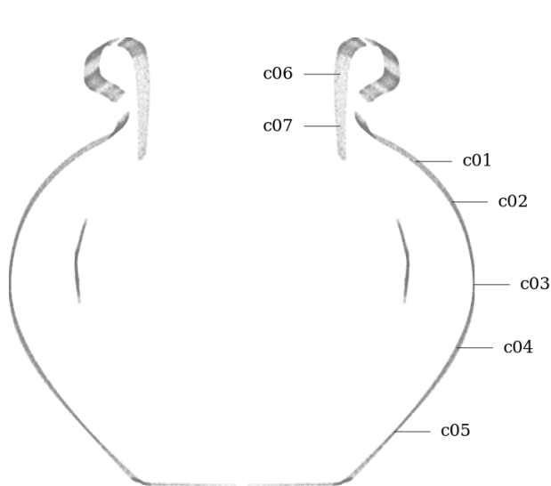
Figure 31: Circularity measurement sample locations, full mesh aligned to exterior surface
