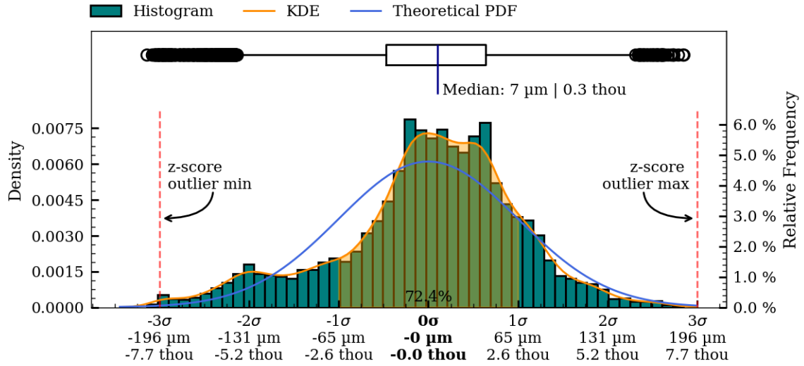
Figure 59: Interior separately aligned surface variability boxplot, kds and histogram.
