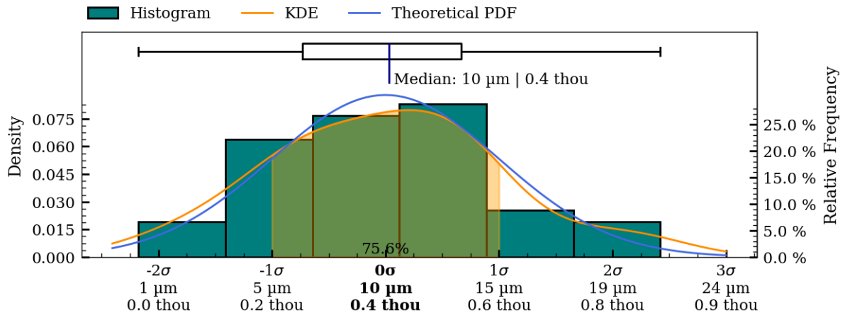
Figure 44: Coaxiality residual plots of interior_separate surface, IV009.
