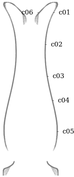
Figure 4: Circularity measurement sample locations, full mesh aligned with exterior surface
