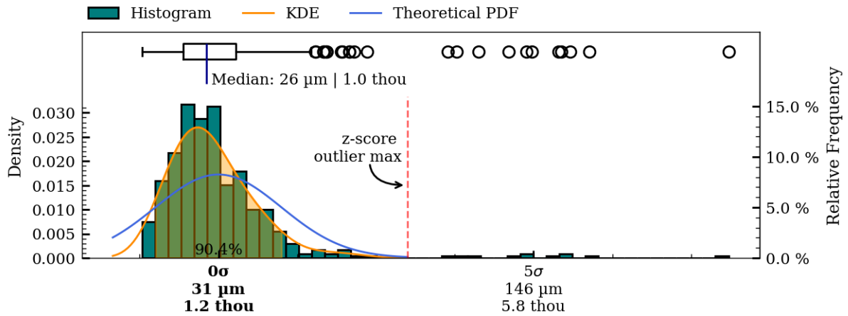
Figure 38: Coaxiality residual plots of exterior surface, IV012.
