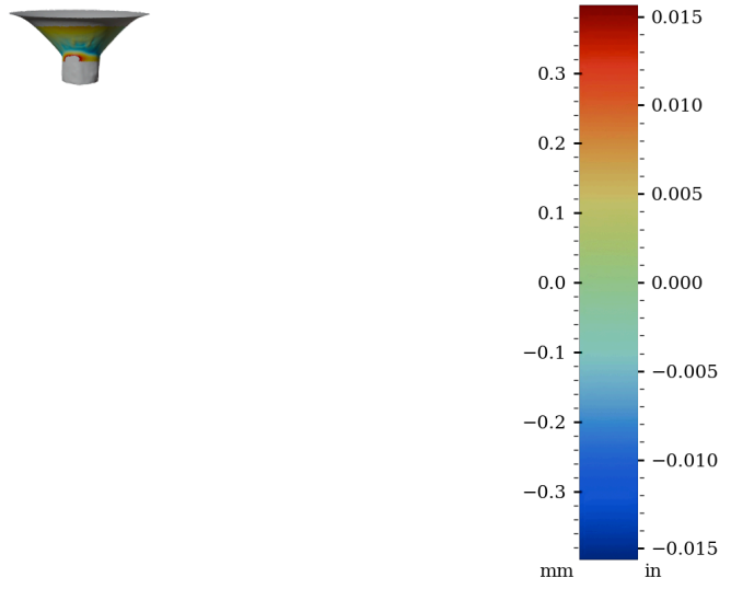
Figure 51: Surface variability heatmap of IV012, rotated 180°
