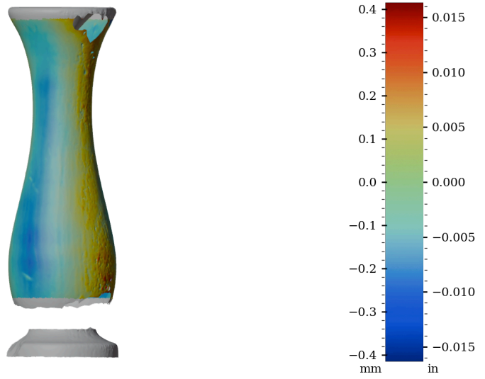
Figure 44: Surface variability heatmap of IV012, rotated 270°
