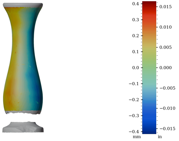
Figure 43: Surface variability heatmap of IV012, rotated 180°
