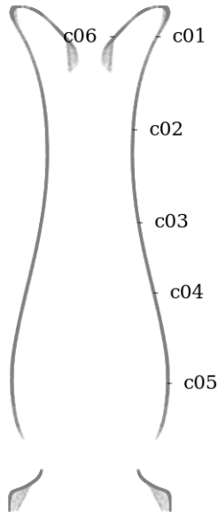
Figure 72: Circularity measurement sample locations, full mesh aligned to exterior surface
