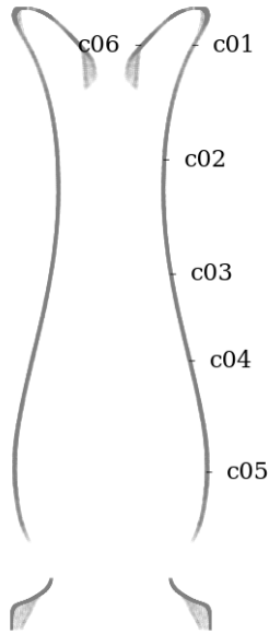
Figure 74: Circularity measurement sample locations, full mesh aligned to exterior surface
