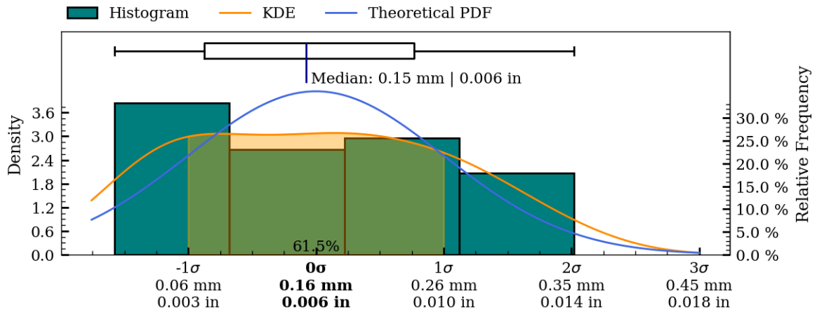
Figure 39: Coaxiality residual plots of interior surface, IV012.
