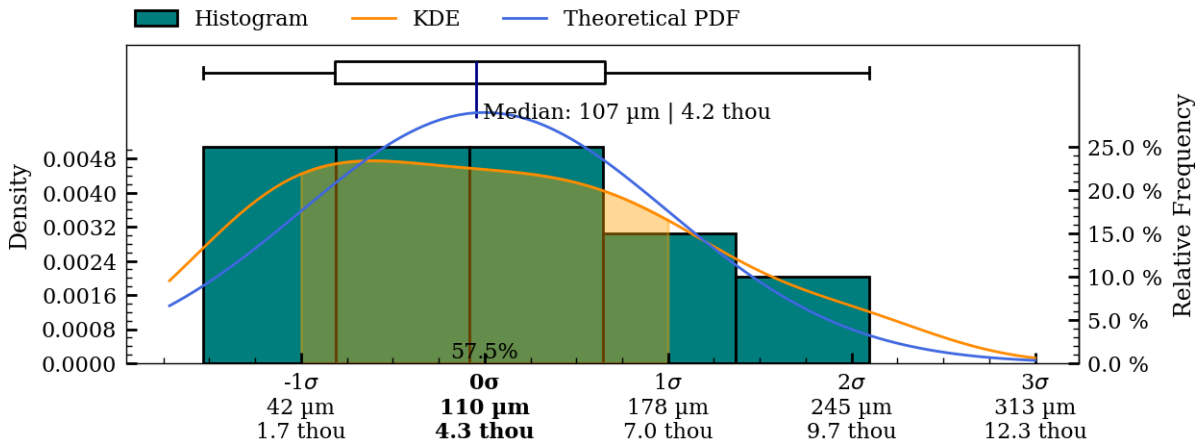
Figure 40: Coaxiality residual plots of interior_separate surface, IV012.
