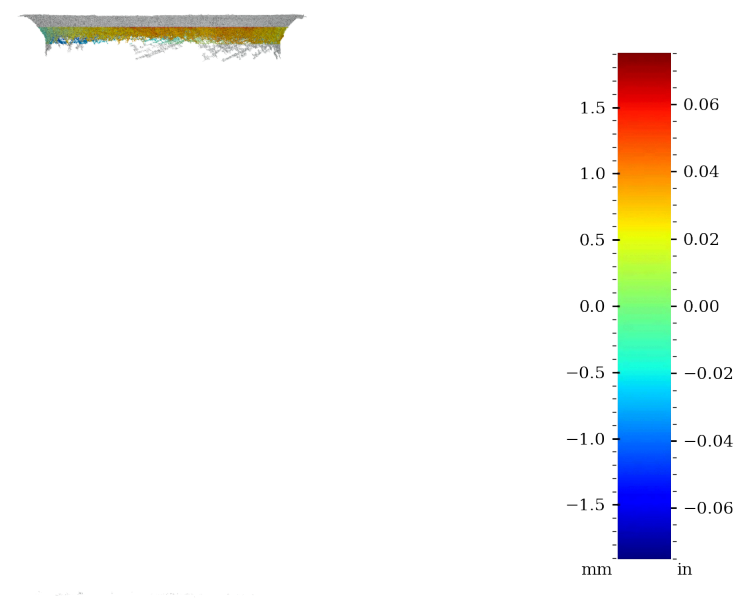
Figure 45: Surface variability heatmap of MV001, front view
