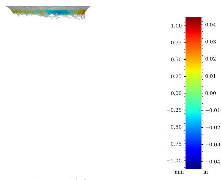
Figure 50: Surface variability heatmap of MV001, rotated 90°
