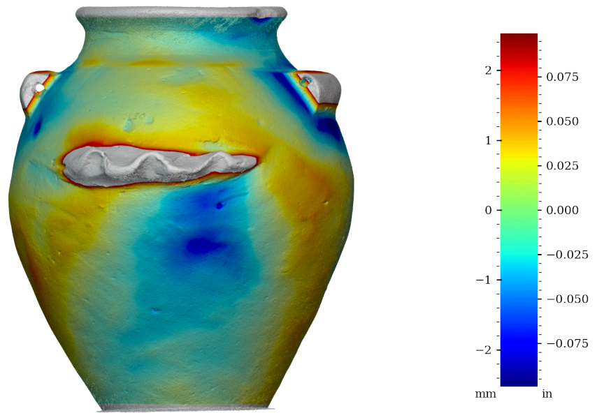
Figure 43: Surface variability heatmap of MV001, rotated 180°
