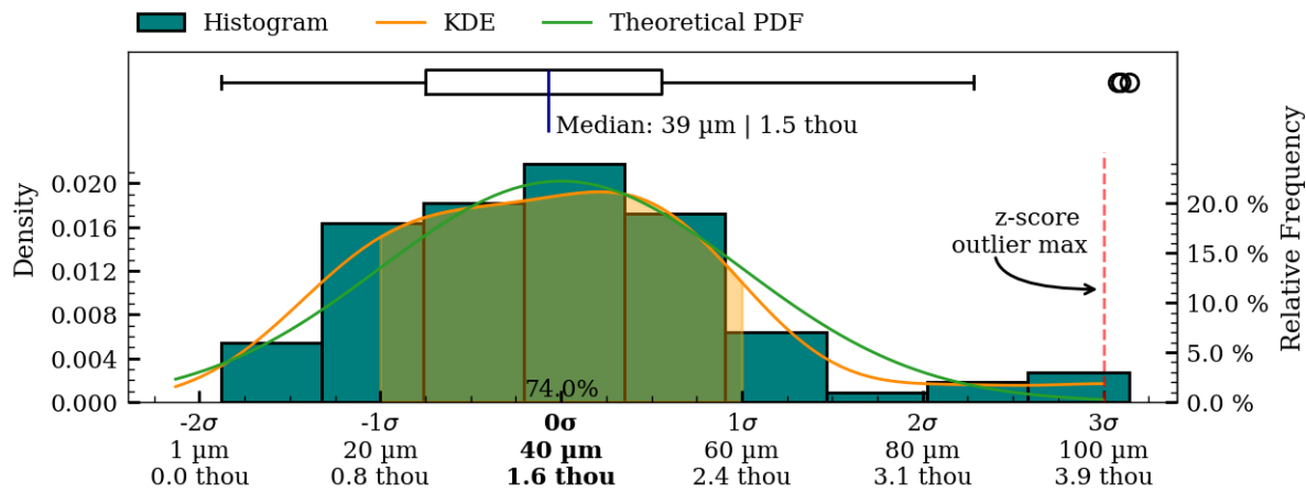
Figure 40: Coaxiality residual plots of interior_separate surface, MV001.
