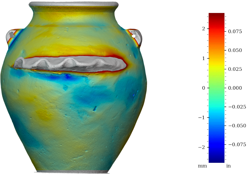
Figure 41: Surface variability heatmap of MV001, front view
