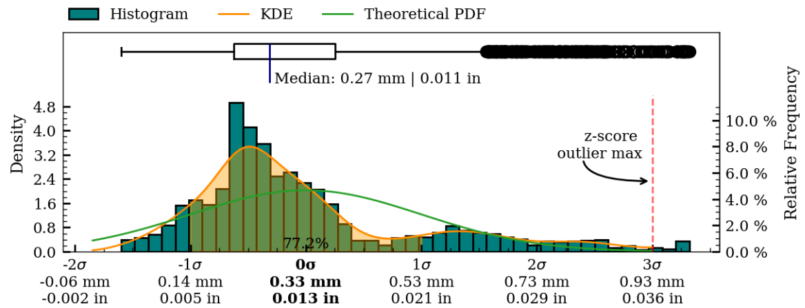
Figure 38: Coaxiality residual plots of exterior surface, MV001.
