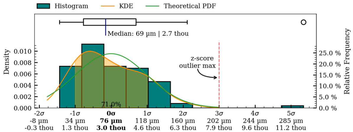
Figure 39: Coaxiality residual plots of interior surface, MV001.
