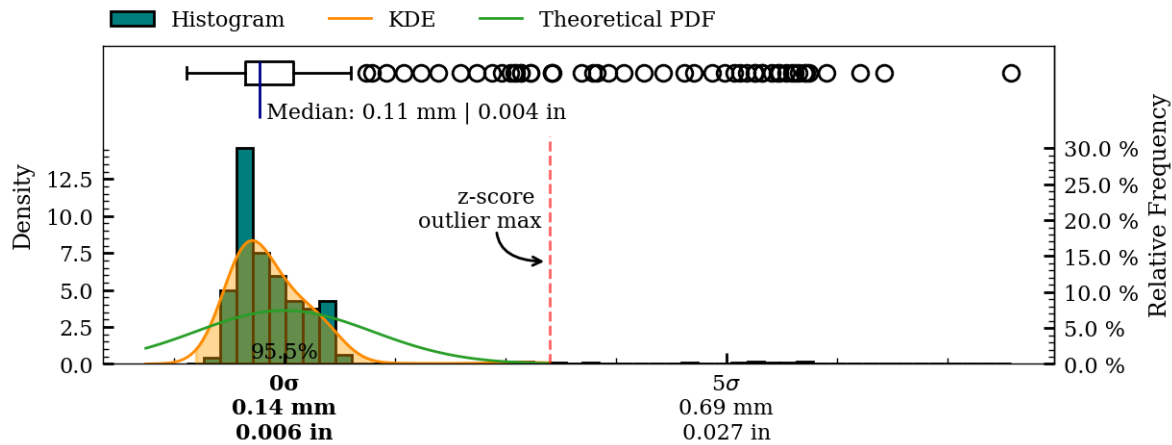
Figure 29: Coaxiality residual plots of exterior surface, MV003.
