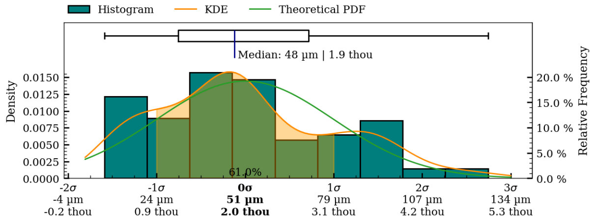
Figure 30: Coaxiality residual plots of interior surface, MV003.
