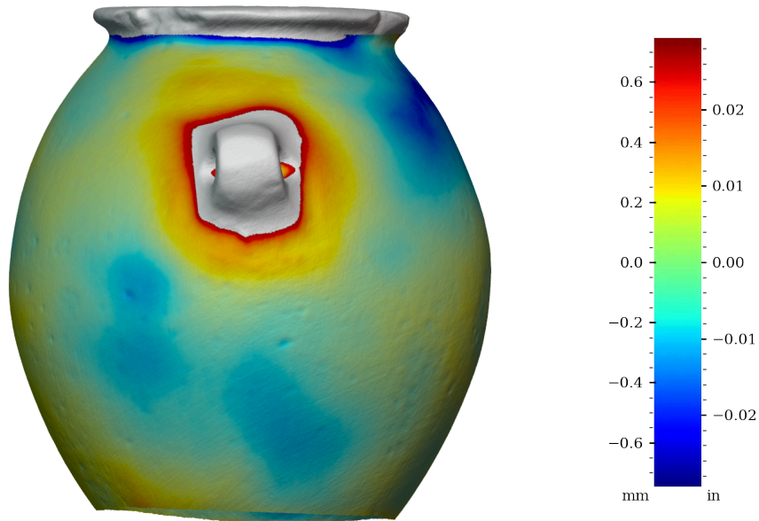
Figure 32: Surface variability heatmap of MV003, rotated 90°
