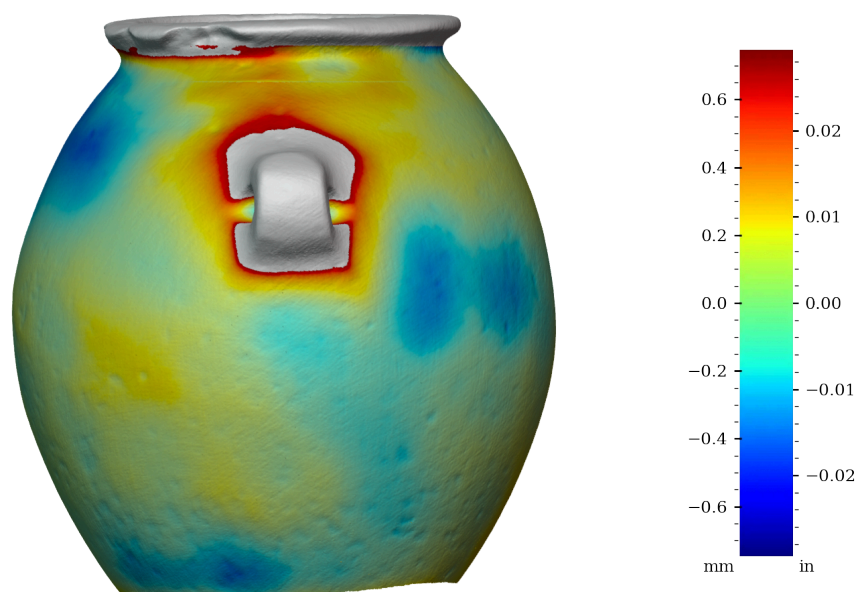
Figure 34: Surface variability heatmap of MV003, rotated 270°
