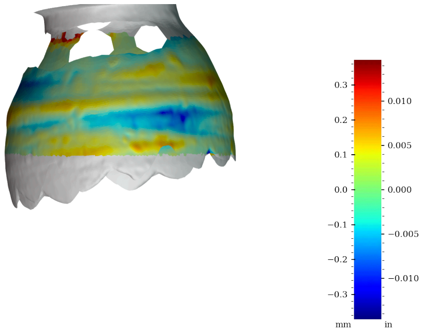
Figure 55: Surface variability heatmap of MV004b, rotated 180°
