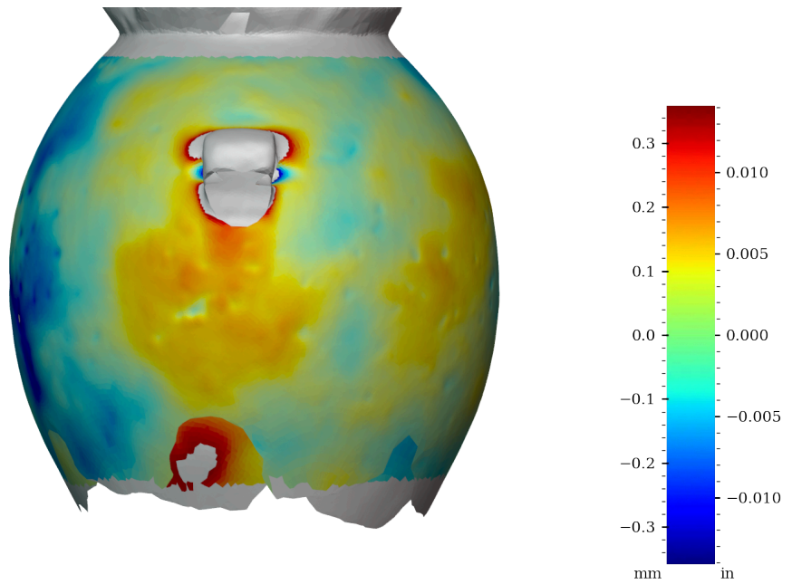
Figure 48: Surface variability heatmap of MV004b, rotated 270°
