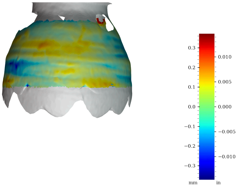
Figure 56: Surface variability heatmap of MV004b, rotated 270°
