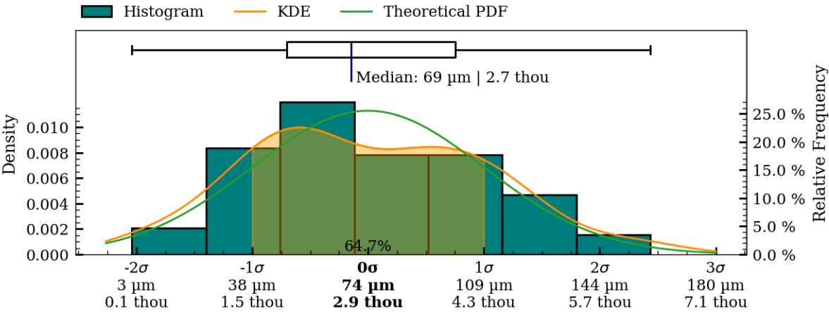
Figure 43: Coaxiality residual plots of interior surface, MV004b.
