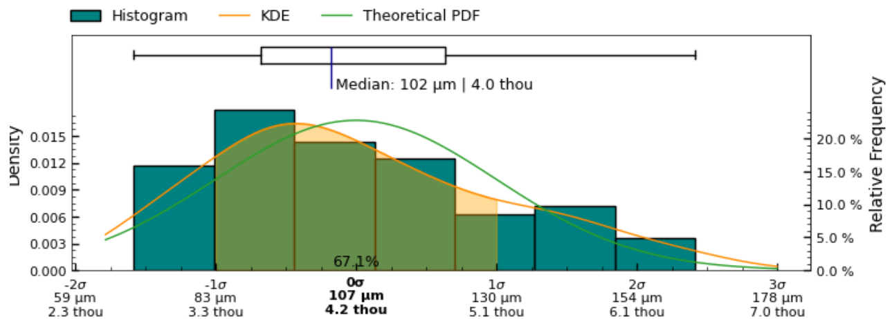
Figure 29: Root Mean Squared Deviation measurement distribution across measured slices of interior separately aligned surface
