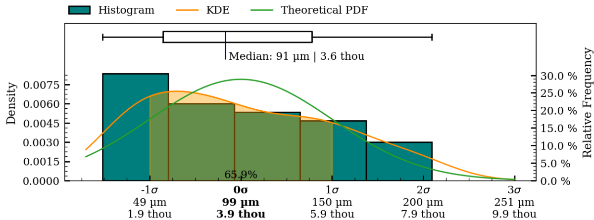
Figure 44: Coaxiality residual plots of interior_separate surface, MV004b.
