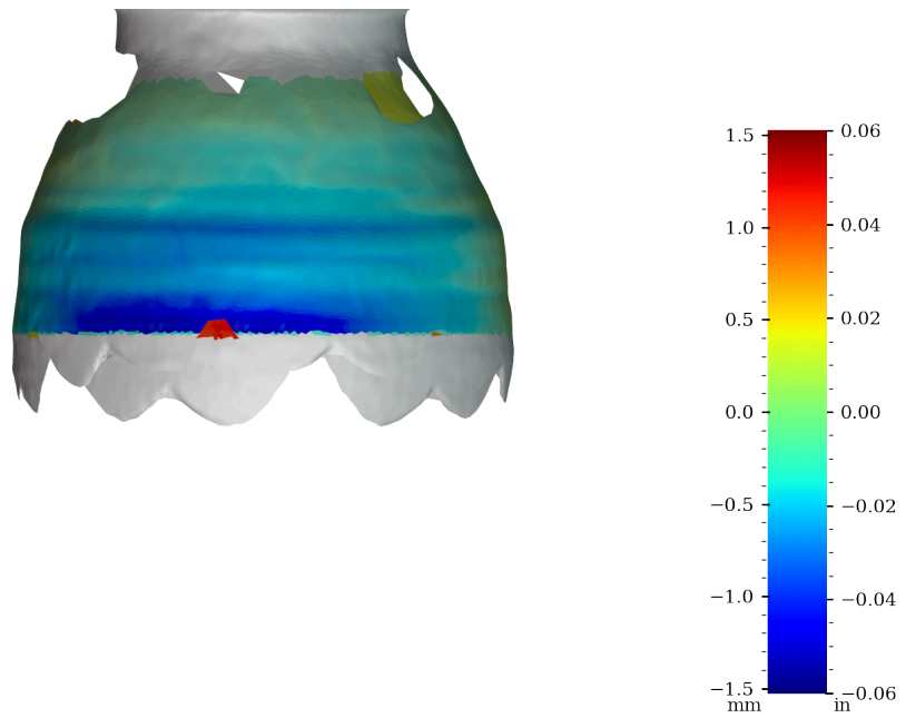
Figure 52: Surface variability heatmap of MV004b, rotated 270°
