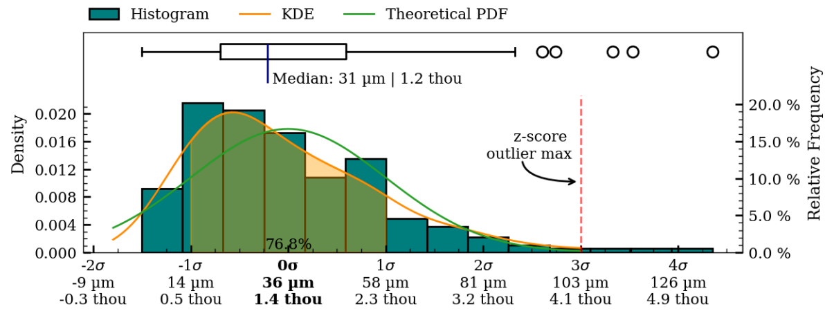
Figure 42: Coaxiality residual plots of exterior surface, MV004b.
