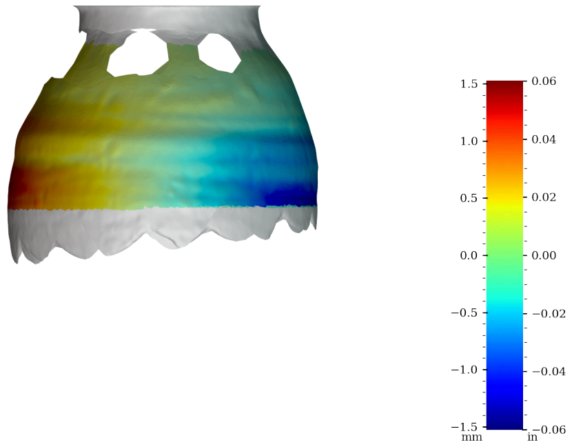
Figure 51: Surface variability heatmap of MV004b, rotated 180°
