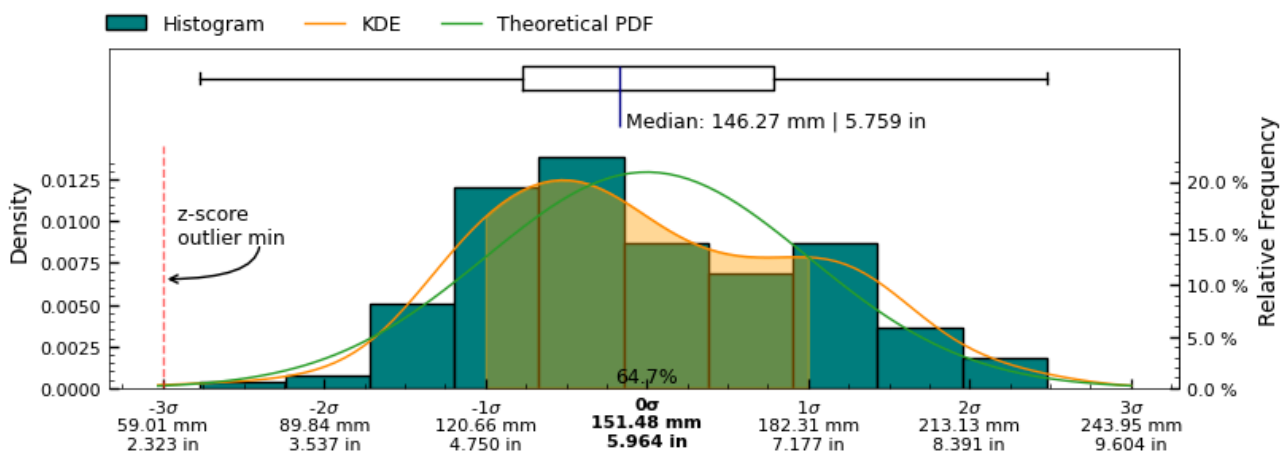
Figure 20: Median absolute deviation measurement distribution across measured slices of interior surface
