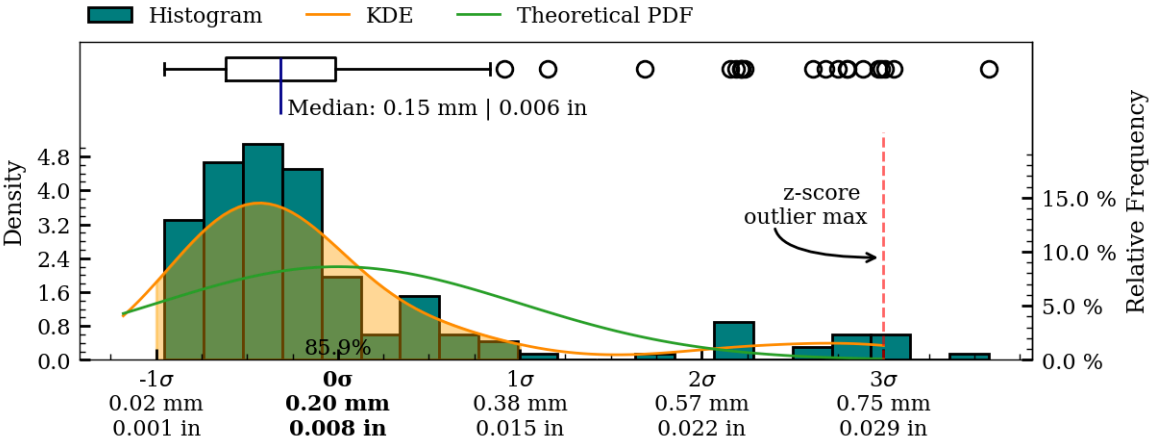
Figure 30: Coaxiality residual plots of interior surface, MV008.
