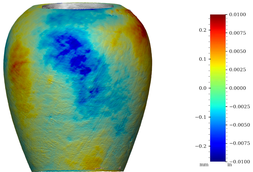
Figure 34: Surface variability heatmap of MV008, rotated 270°
