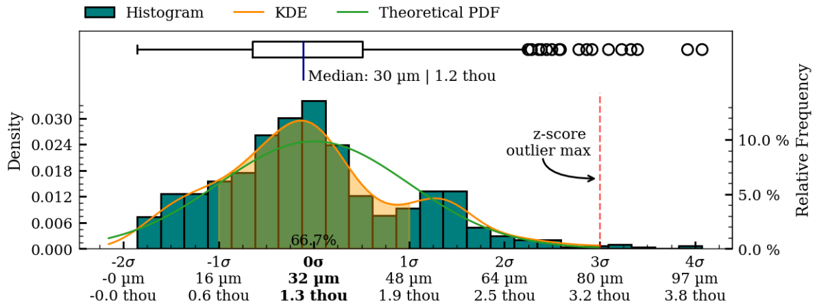
Figure 29: Coaxiality residual plots of exterior surface, MV008.
