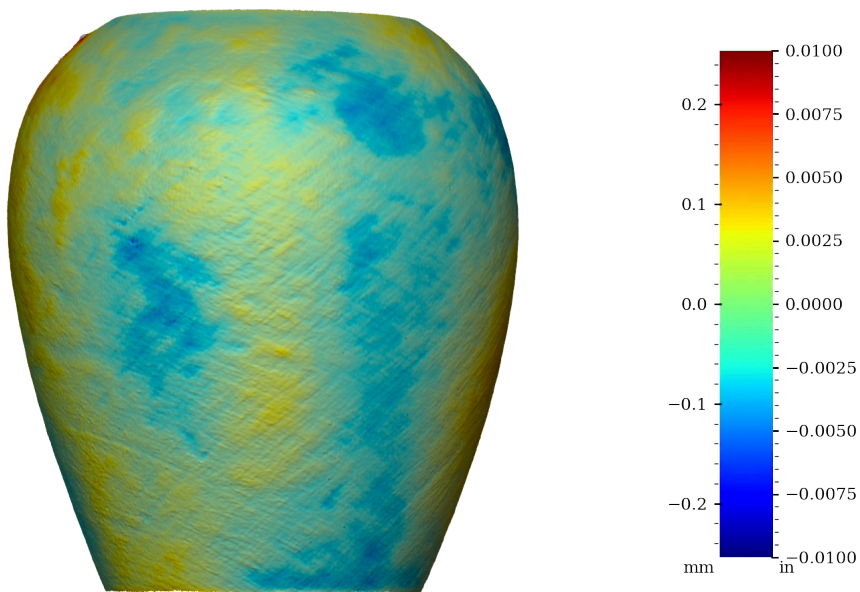
Figure 32: Surface variability heatmap of MV008, rotated 90°
