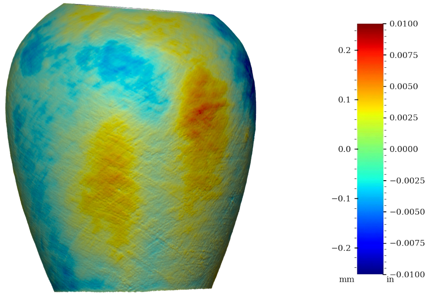
Figure 33: Surface variability heatmap of MV008, rotated 180°
