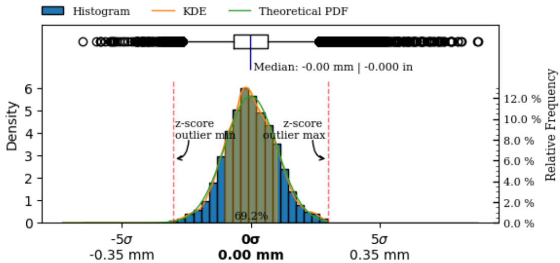
Figure 37: Exterior surface variability boxplot, kds and histogram.
