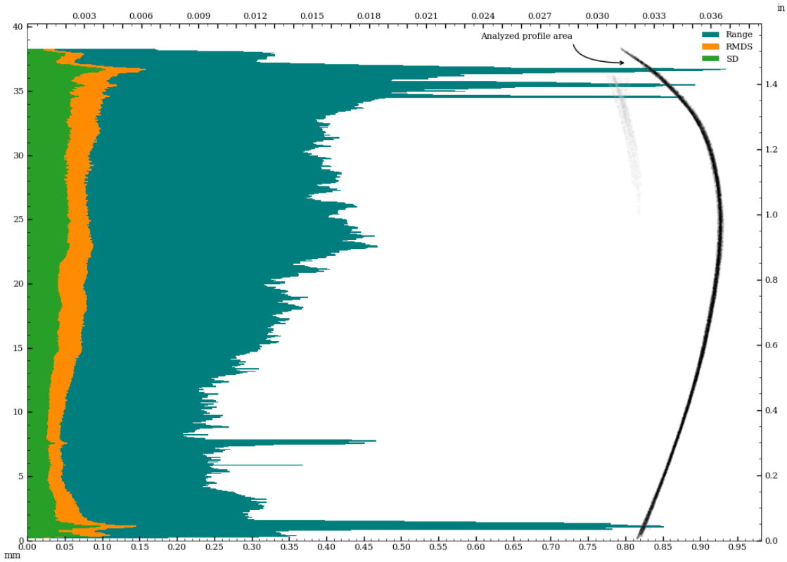
Figure 42: Circularity of exterior surface - in z-plane.
