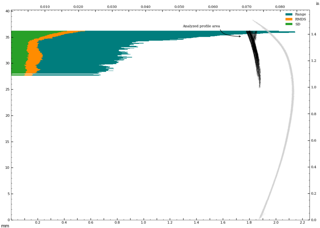
Figure 46: Circularity of interior surface - in z-plane.
