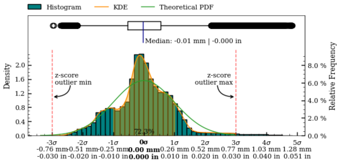
Figure 38: Interior surface variability boxplot, kds and histogram.
