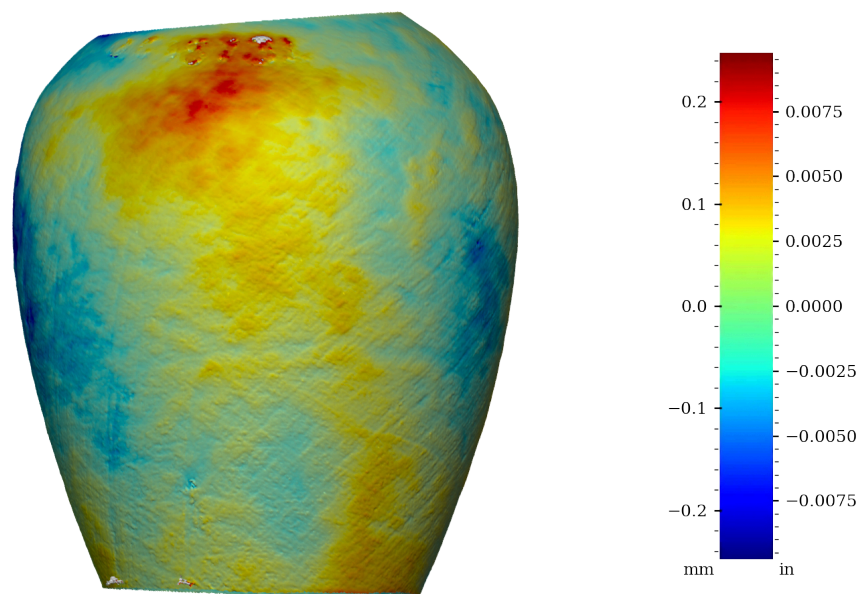
Figure 29: Surface variability heatmap of MV008, front view
