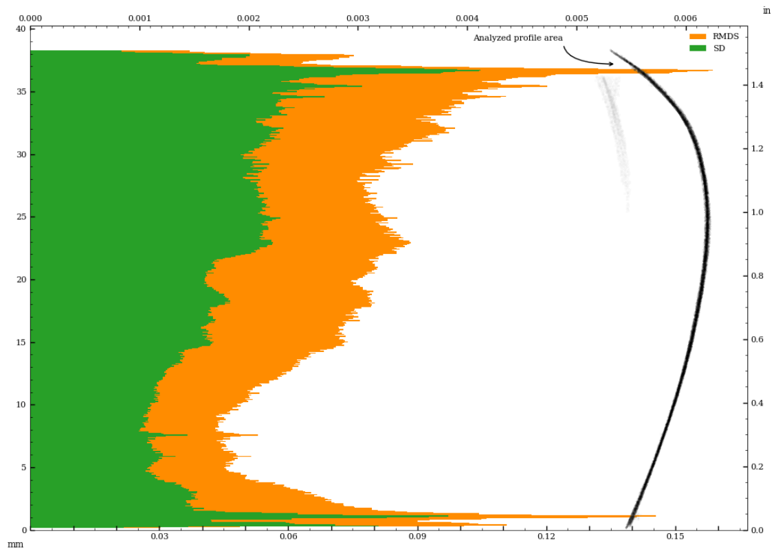
Figure 44: Vessel circularity of exterior surface, in z-plane, standard deviation and median absolute deviation.
