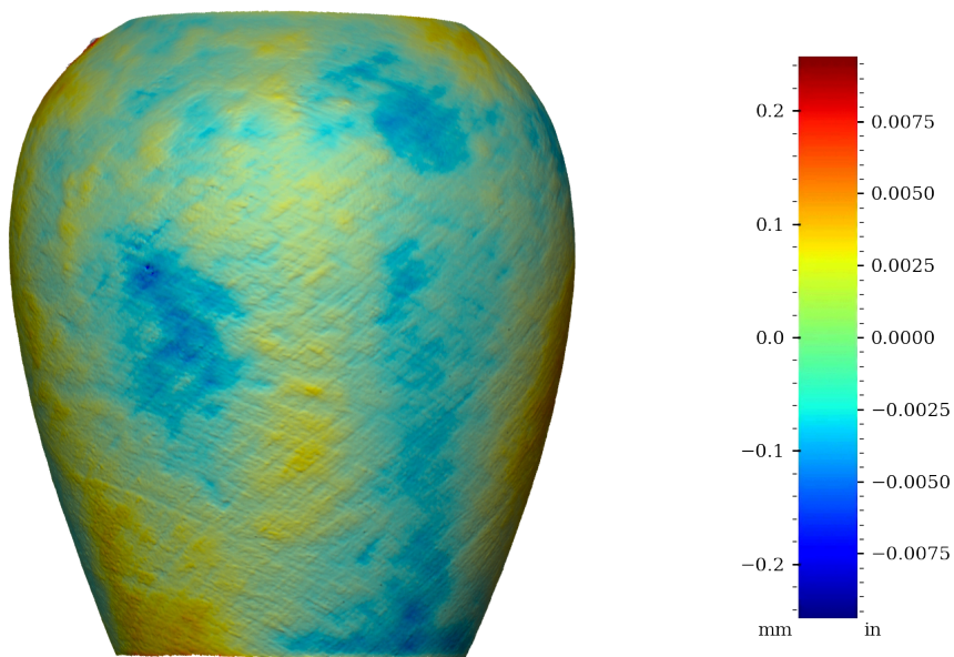
Figure 30: Surface variability heatmap of MV008, rotated 90°
