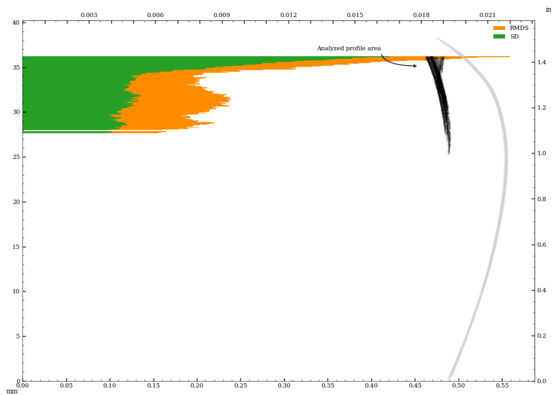
Figure 48: Vessel circularity of interior surface, in z-plane, standard deviation and median absolute deviation.
