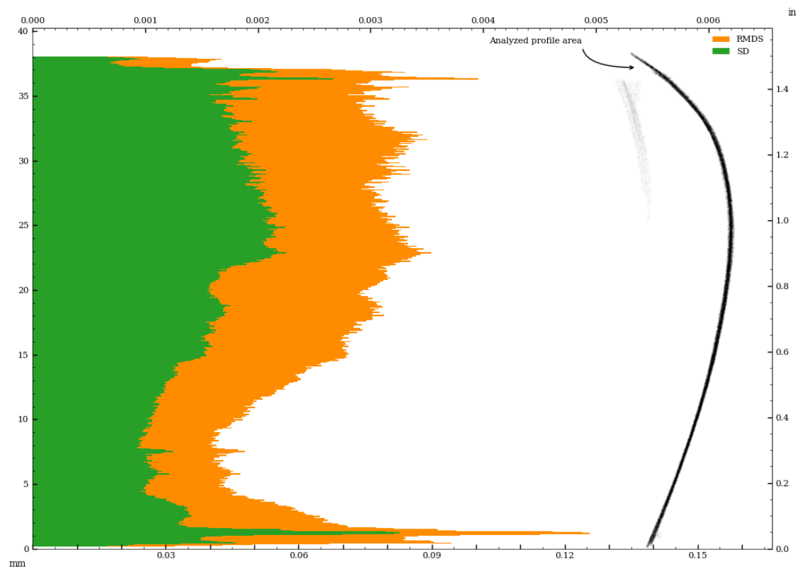
Figure 43: Vessel circularity of exterior surface, perpendicular to surface curvature, standard deviation and median absolute deviation.
