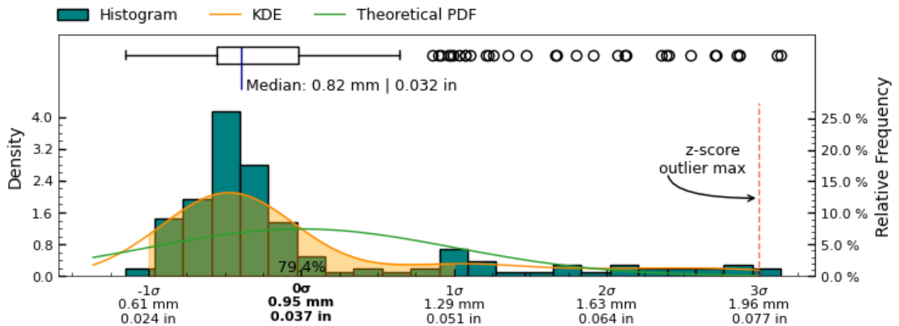
Figure 17: Range measurement distribution across measured slices of interior surface
