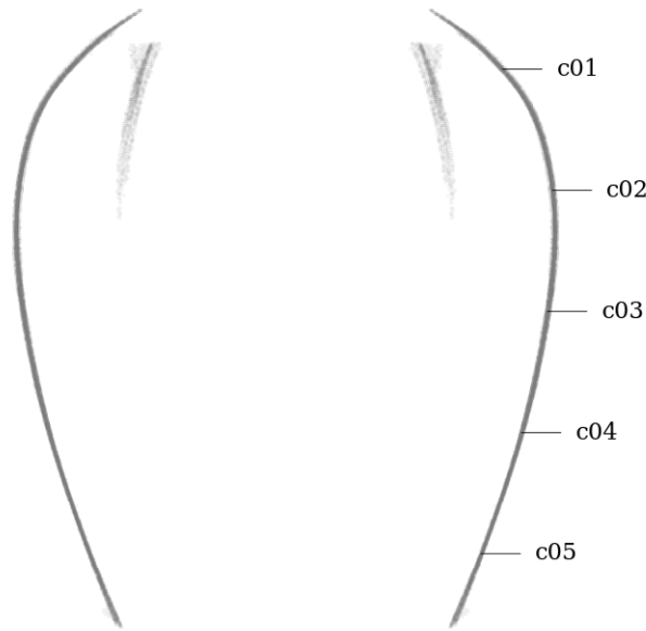
Figure 39: Circularity measurement sample locations, full mesh aligned to exterior surface
