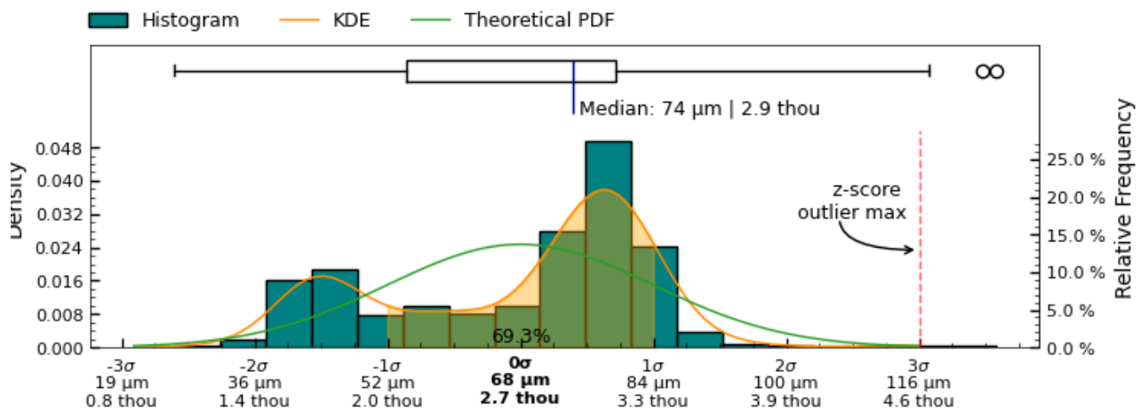
Figure 14: Root Mean Squared Deviation measurement distribution across measured slices of exterior surface
