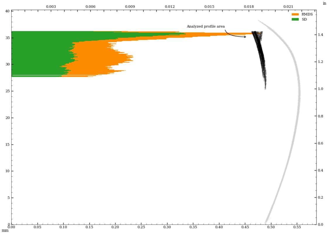
Figure 47: Vessel circularity of interior surface, perpendicular to surface curvature, standard deviation and median absolute deviation.
