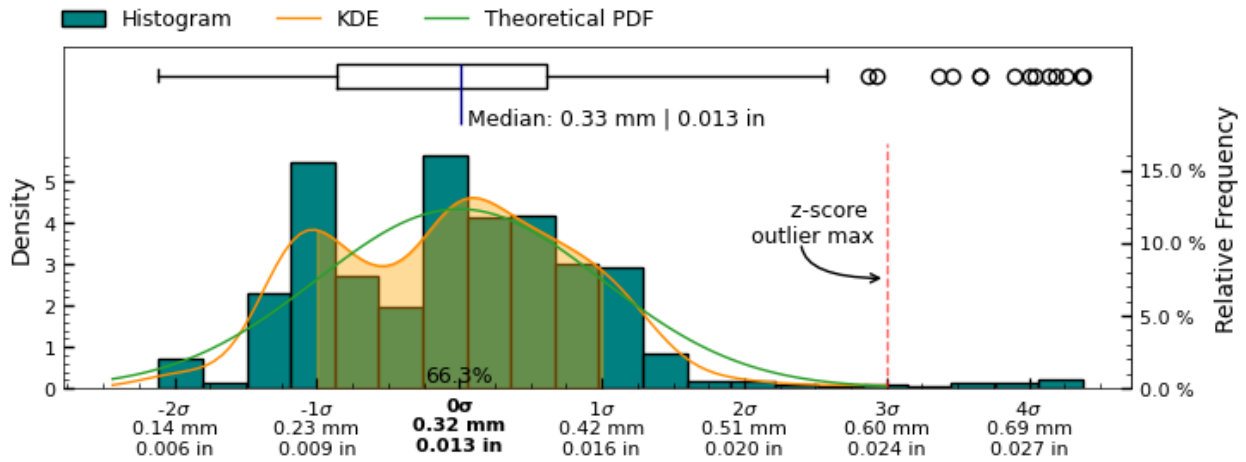
Figure 12: Range measurement distribution across measured slices of exterior surface
