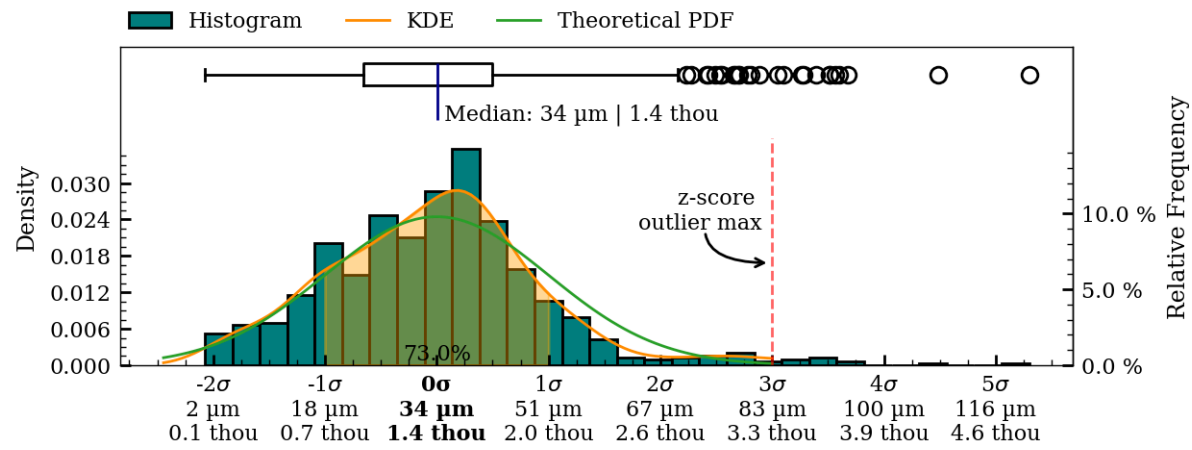
Figure 27: Coaxiality residual plots of exterior surface, MV008.
