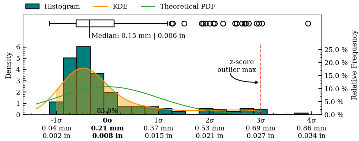
Figure 28: Coaxiality residual plots of interior surface, MV008.
