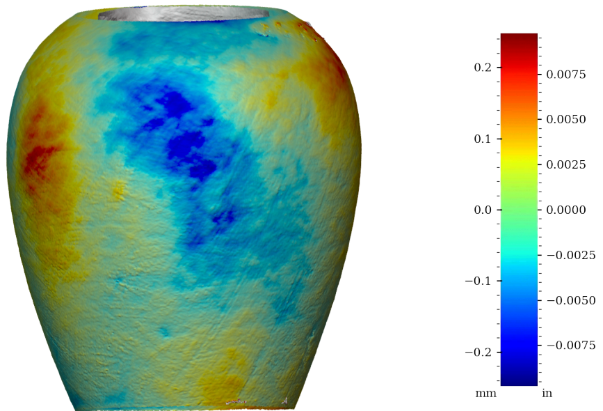
Figure 32: Surface variability heatmap of MV008, rotated 270°
