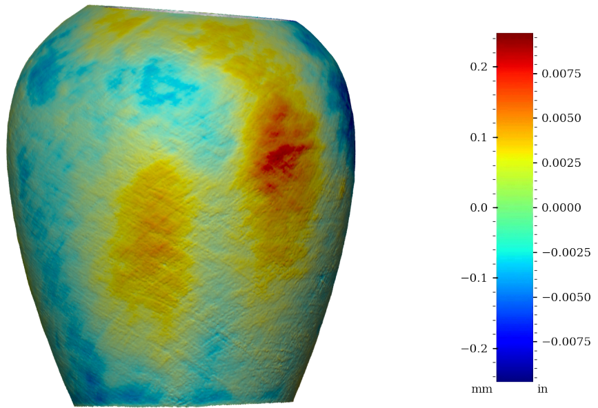
Figure 31: Surface variability heatmap of MV008, rotated 180°
