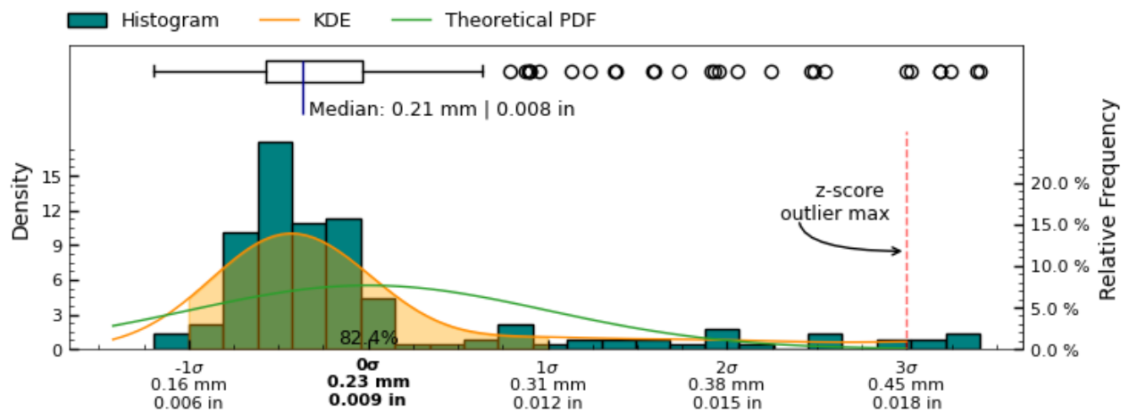
Figure 19: Root Mean Squared Deviation measurement distribution across measured slices of interior surface
