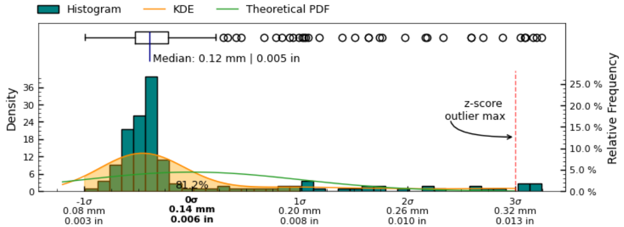
Figure 18: Standard Deviation measurement distribution across measured slices of “ + interior + ” surface
