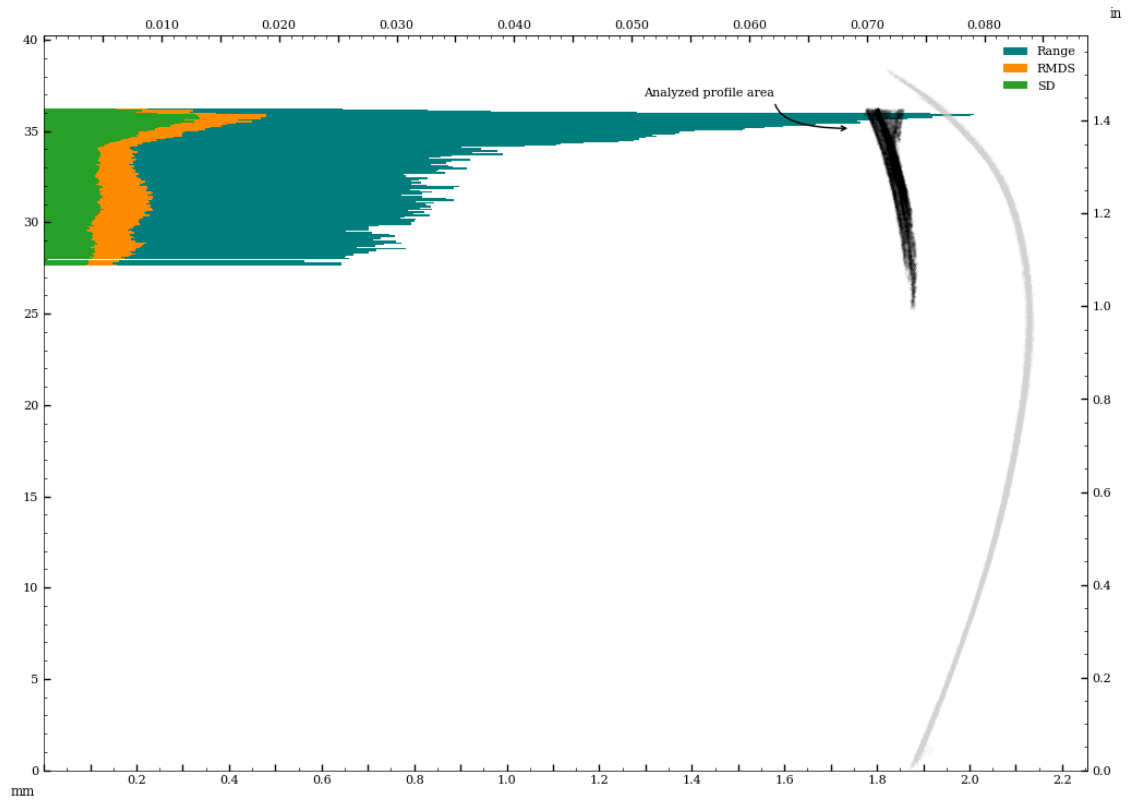
Figure 45: Circularity of interior surface - perpendicular to surface curvature.
