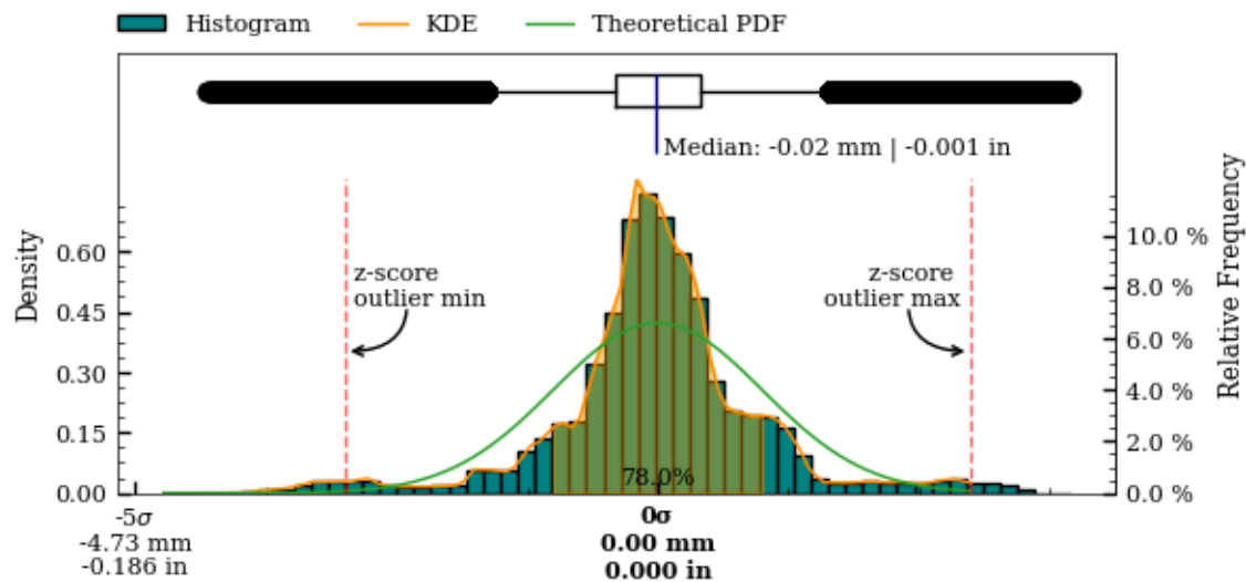
Figure 41: Exterior surface variability boxplot, kds and histogram.
