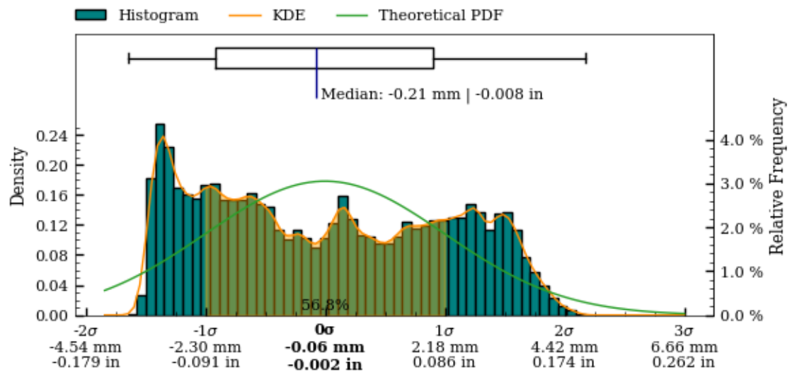
Figure 42: Interior surface variability boxplot, kds and histogram.
