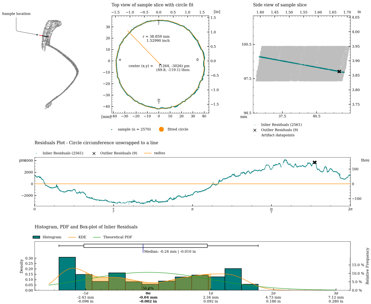
Figure 30: Detailed plot of concentricity measurement for c07.
