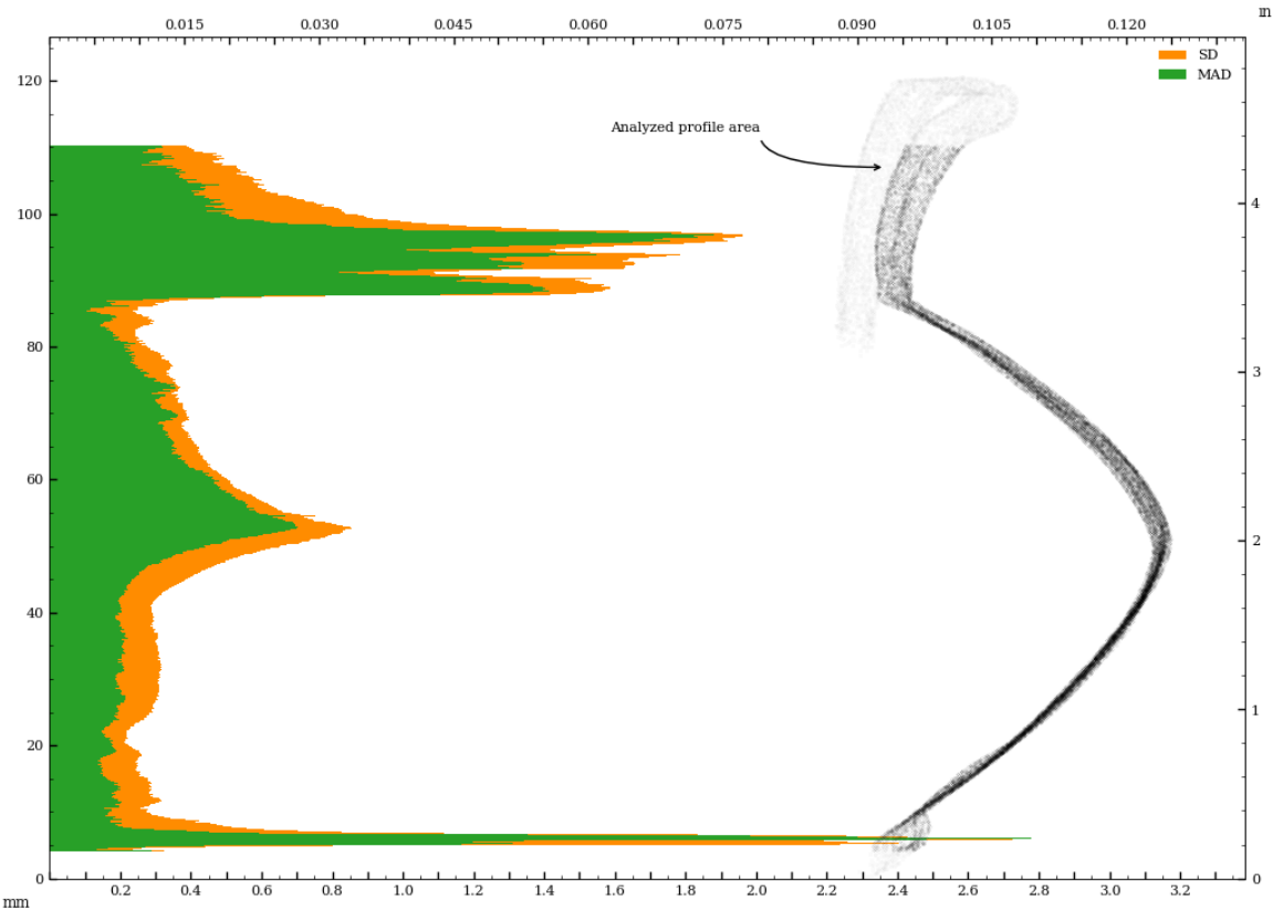
Figure 45: Circularity analysis of exterior samples perpendicular to surface curvature
