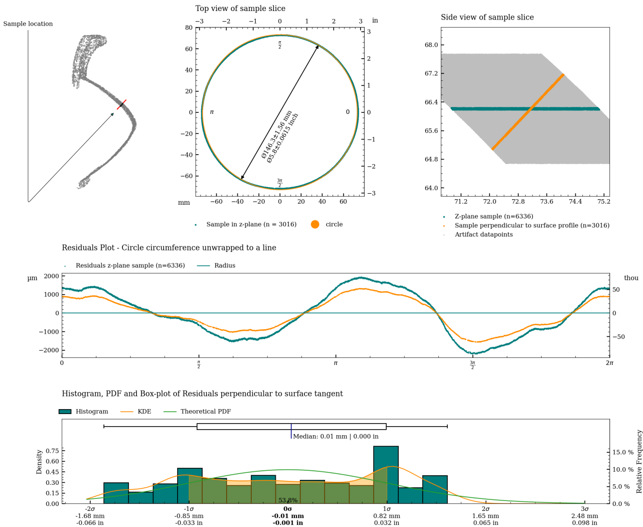
Figure 7: Charts with statistics for the measurement of c03.
