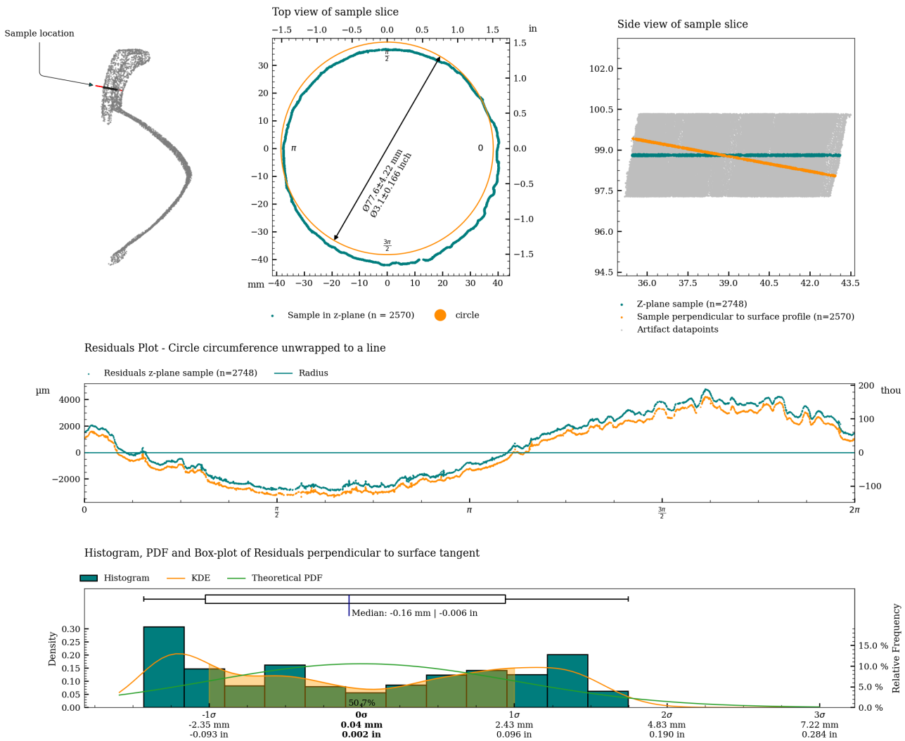
Figure 11: Charts with statistics for the measurement of c07.
