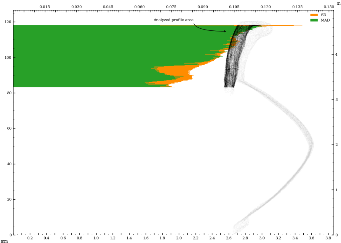
Figure 50: Circularity analysis of interior surface - in z-plane
