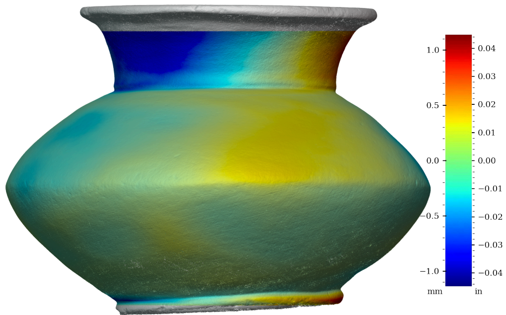
Figure 36: Surface variability heatmap of MV010, rotated 270°
