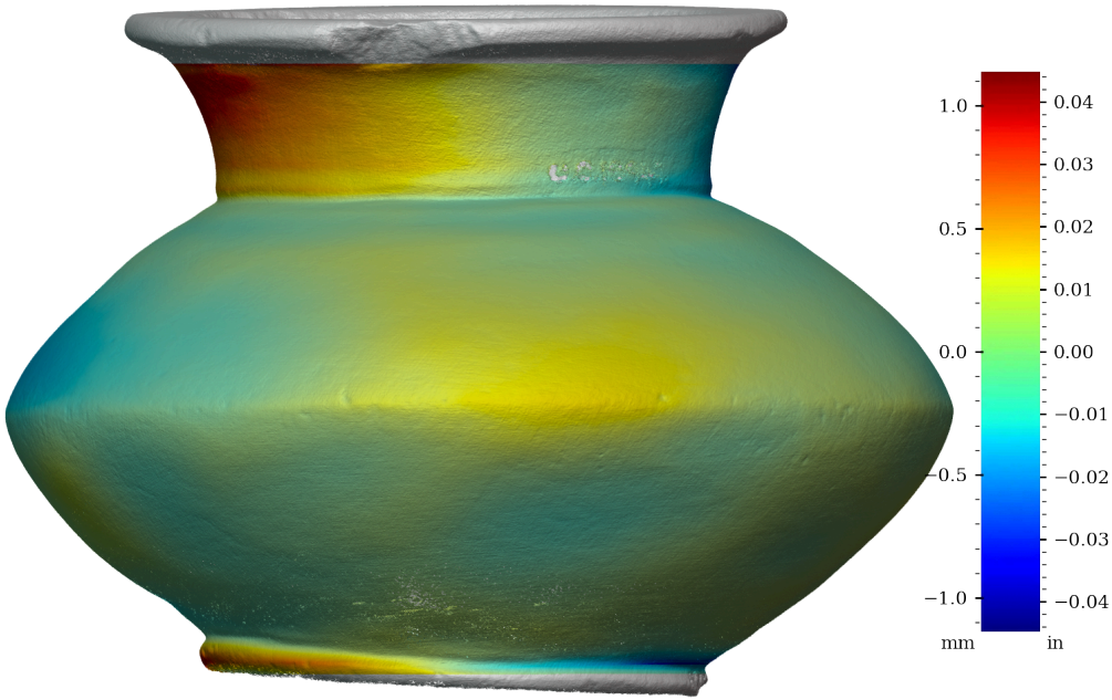
Figure 34: Surface variability heatmap of MV010, rotated 90°
