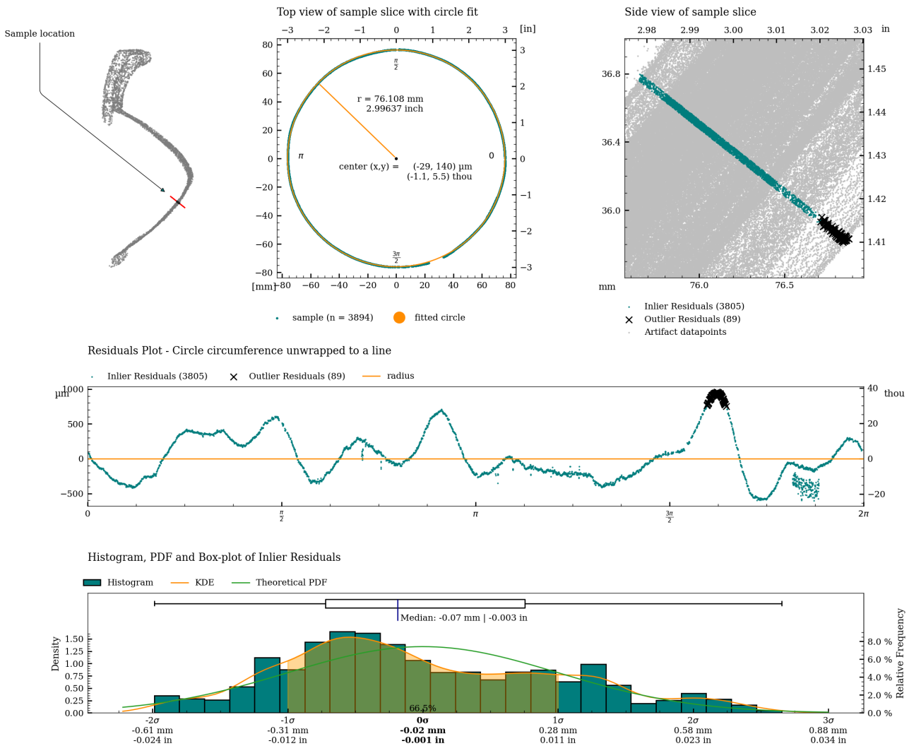
Figure 28: Detailed plot of concentricity measurement for c05.
