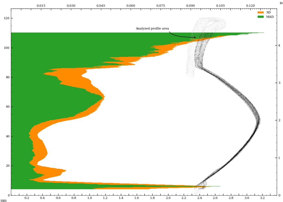
Figure 46: Circularity analysis of exterior surface - in z-plane
