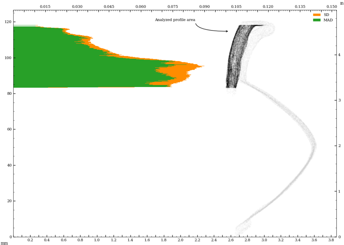
Figure 49: Circularity analysis of interior samples perpendicular to surface curvature
