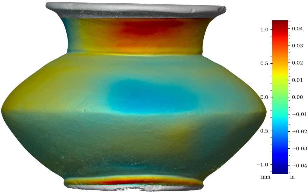
Figure 33: Surface variability heatmap of MV010, front view
