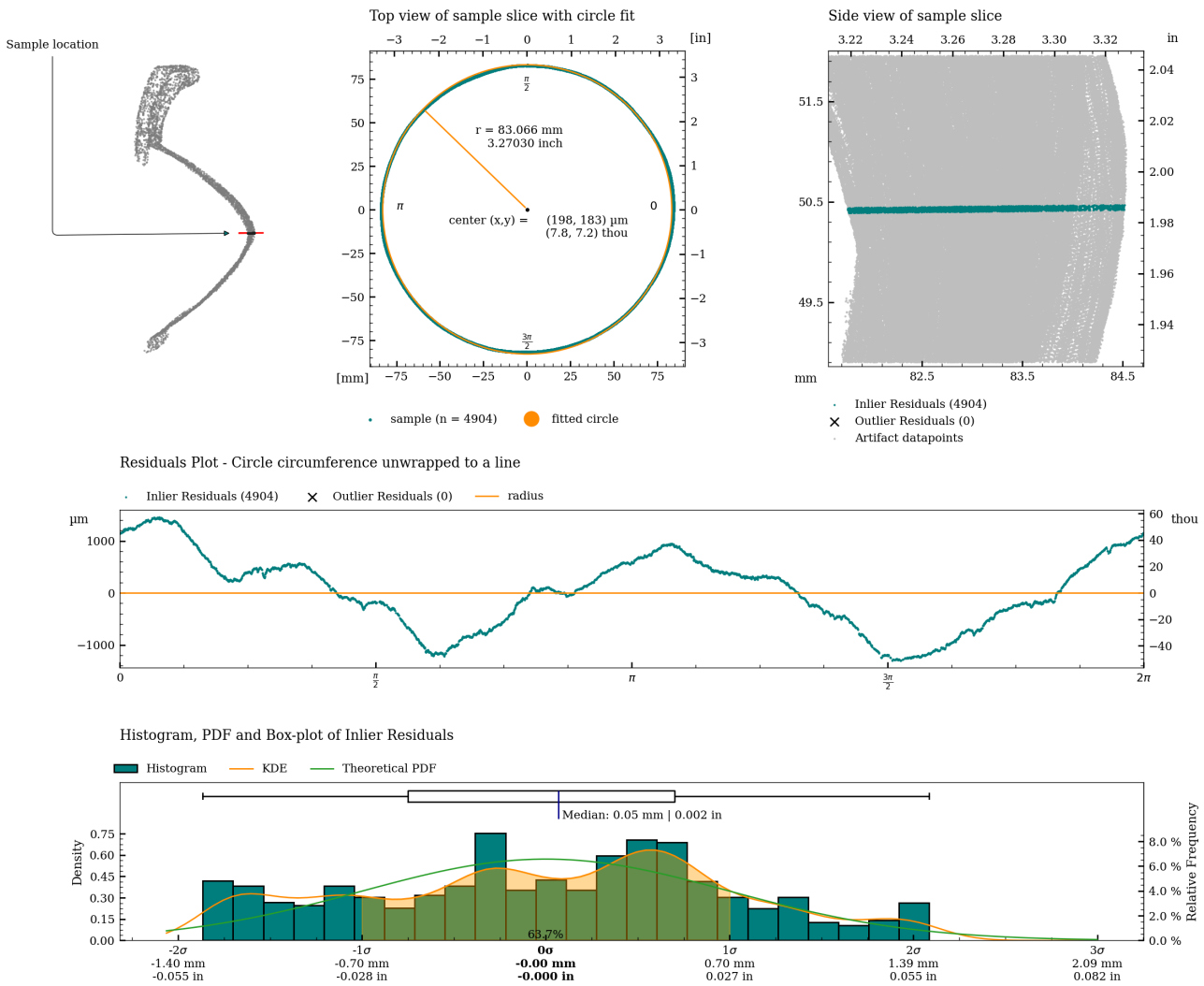
Figure 27: Detailed plot of concentricity measurement for c04.
