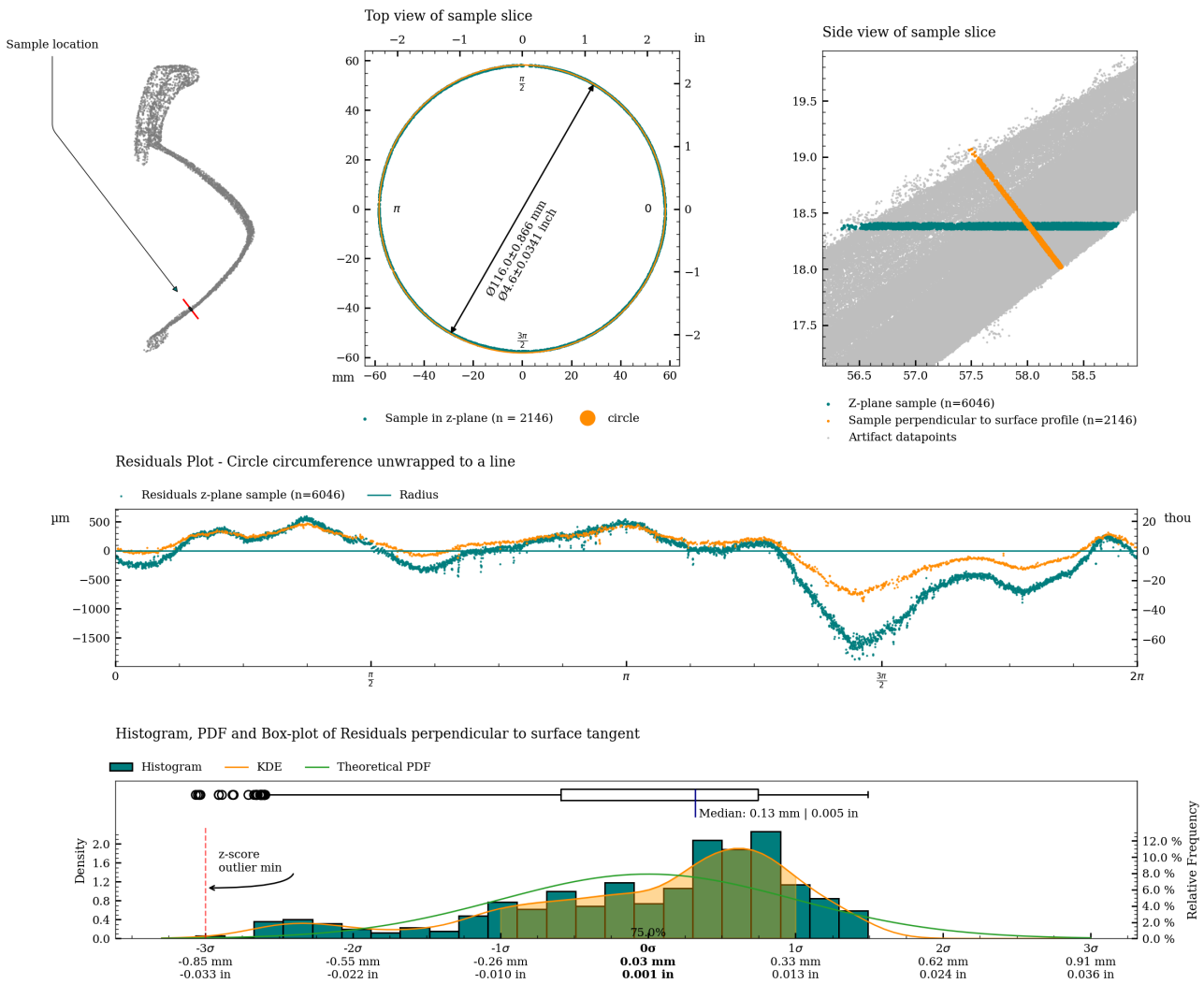
Figure 10: Charts with statistics for the measurement of c06.
