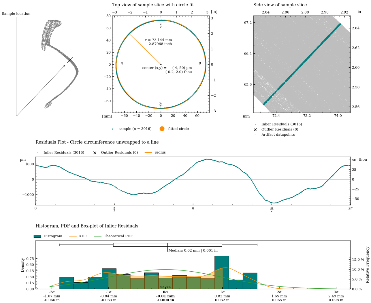
Figure 26: Detailed plot of concentricity measurement for c03.
