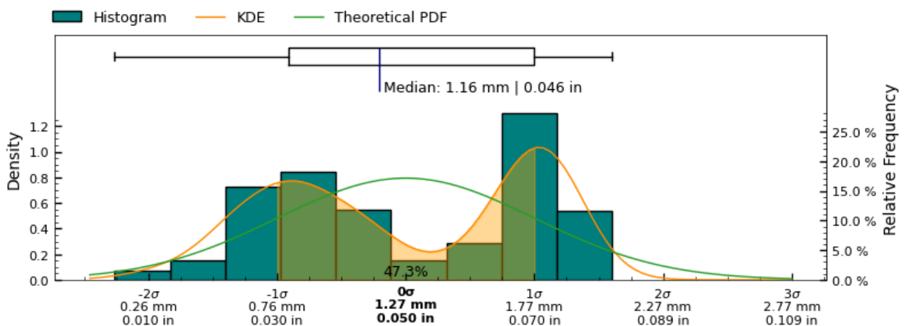
Figure 21: Median absolute deviation measurement distribution across measured slices of interior surface
