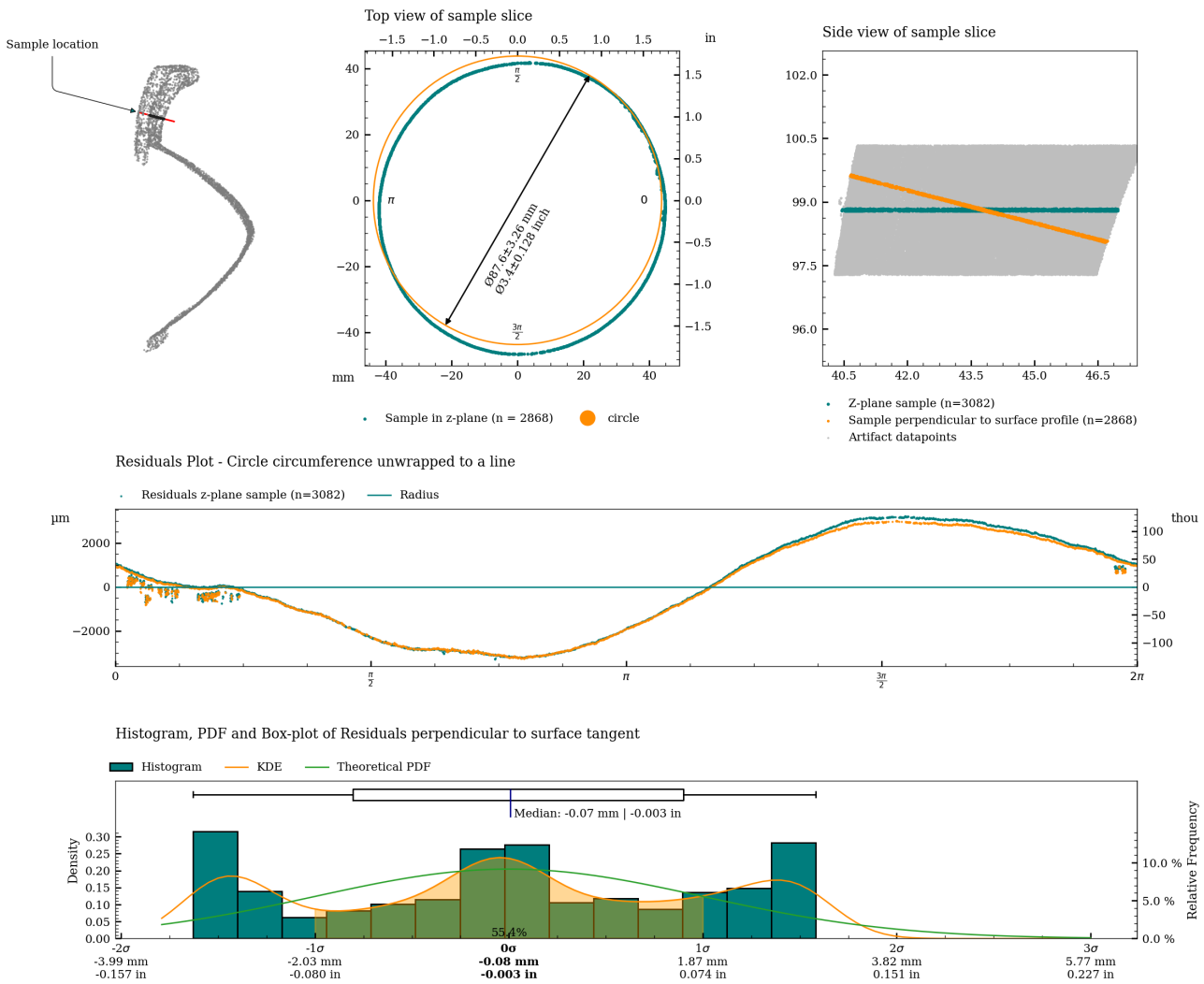
Figure 5: Charts with statistics for the measurement of c01.
