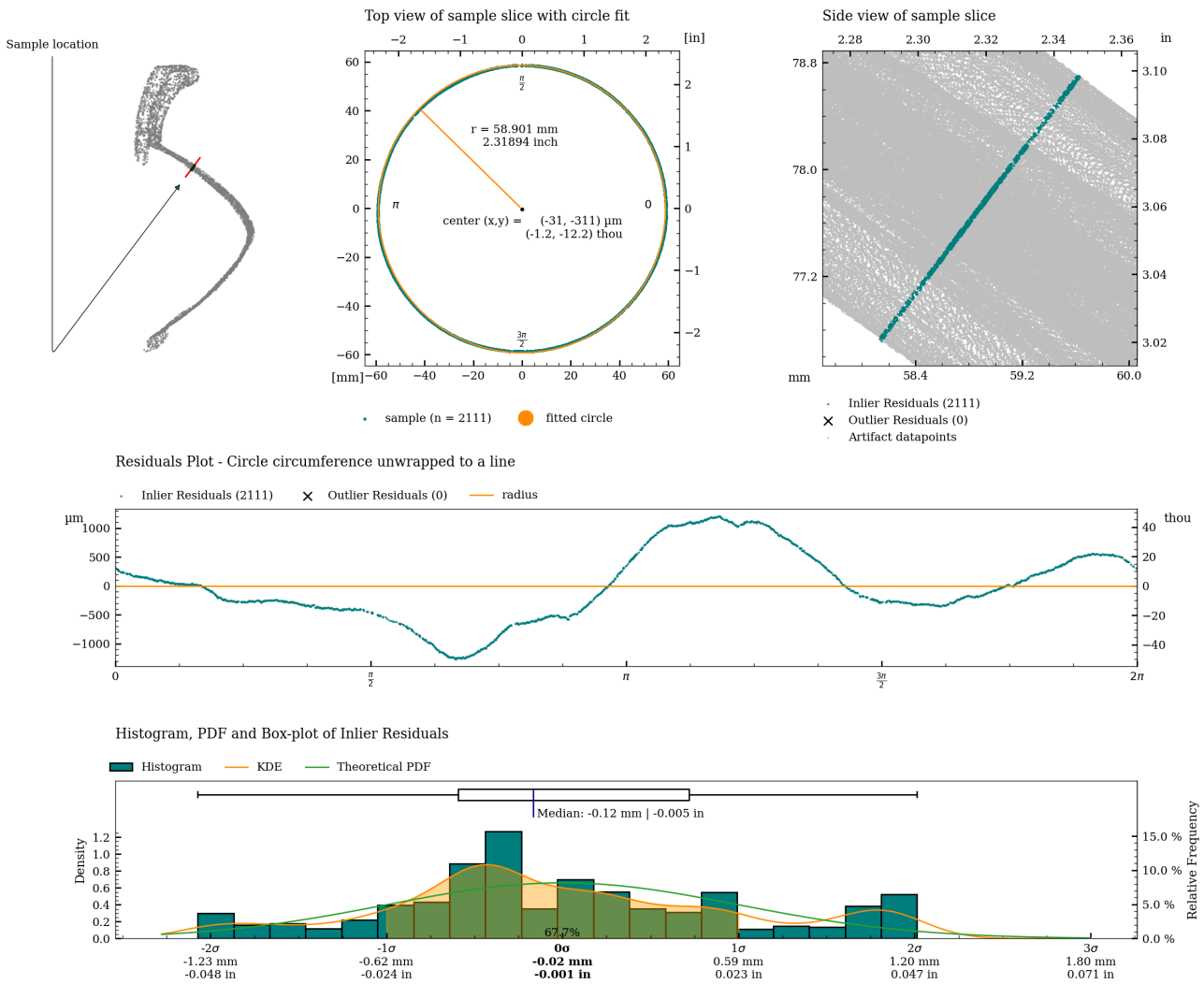
Figure 25: Detailed plot of concentricity measurement for c02.
