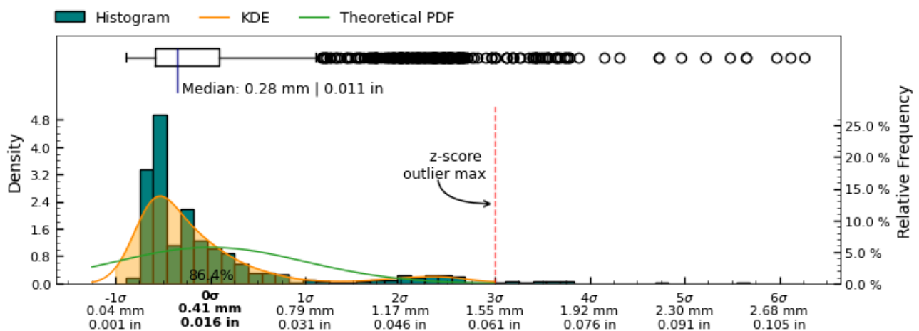
Figure 16: Median absolute deviation measurement distribution across measured slices of exterior surface
