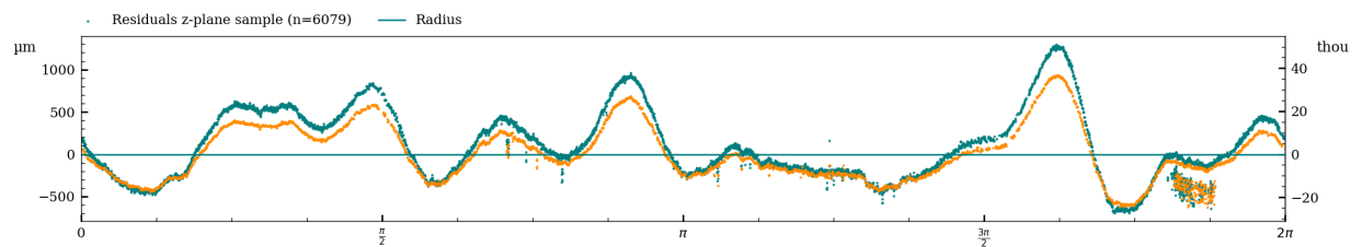
Residuals Plot - Circle circumference unwrapped to a line
