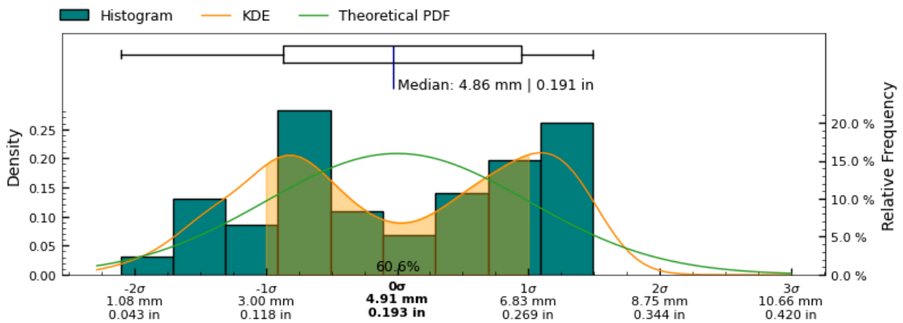
Figure 19: Range measurement distribution across measured slices of interior surface
