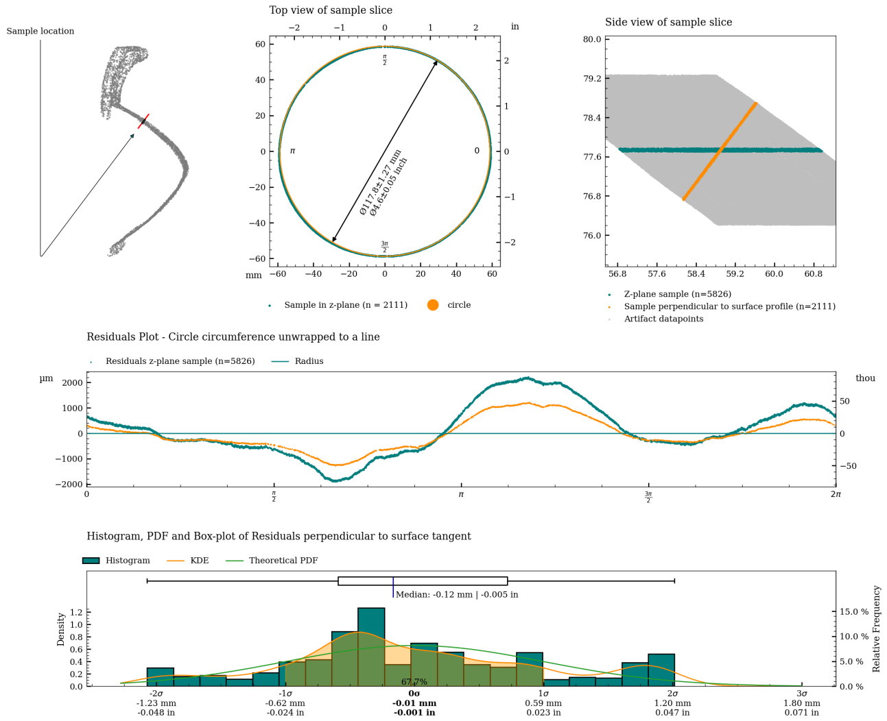
Figure 6: Charts with statistics for the measurement of c02.
