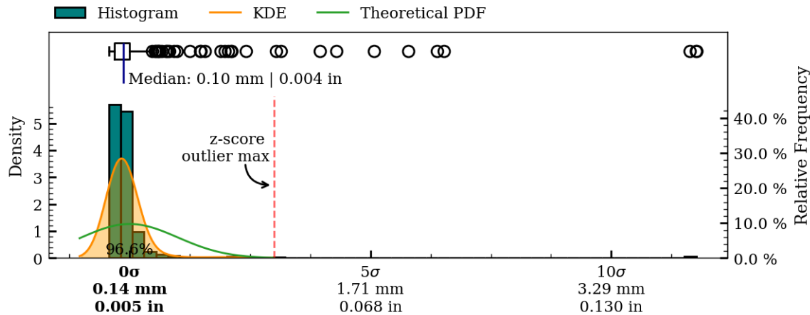
Figure 32: Coaxiality residual plots of interior surface, MV010.
