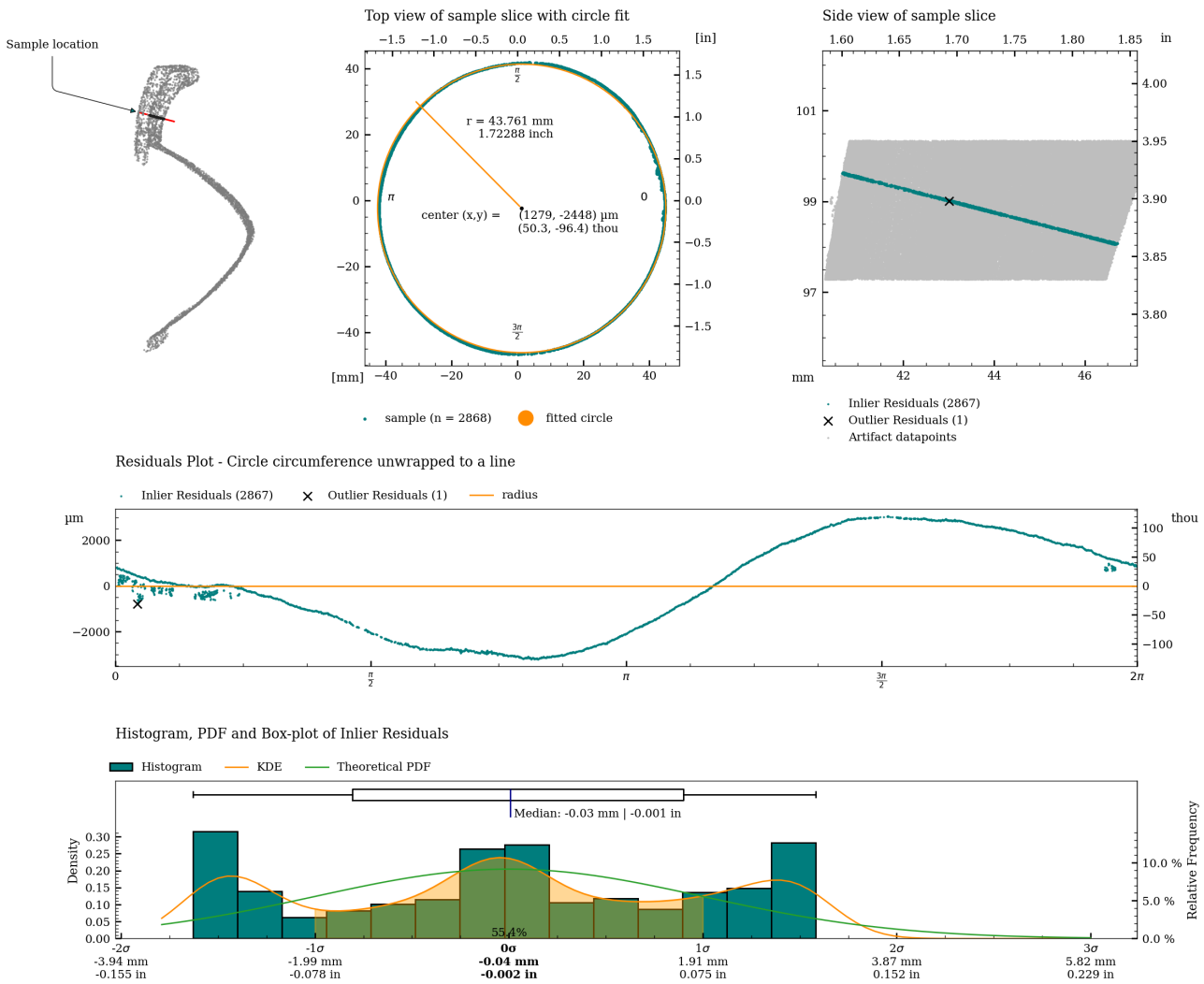
Figure 24: Detailed plot of concentricity measurement for c01.
