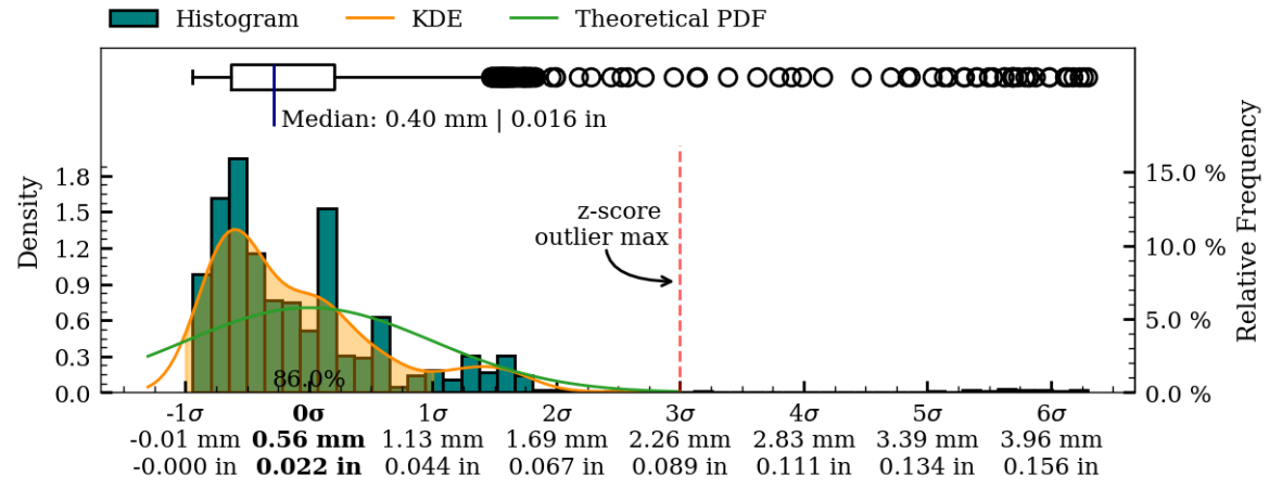
Figure 31: Coaxiality residual plots of exterior surface, MV010.
