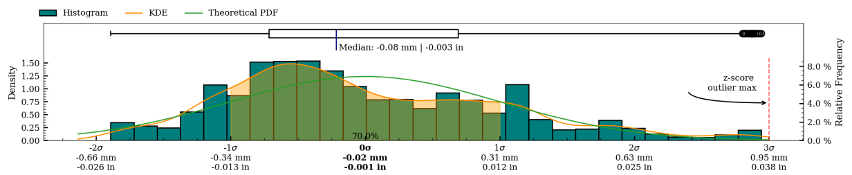
Figure 9: Charts with statistics for the measurement of c05.
