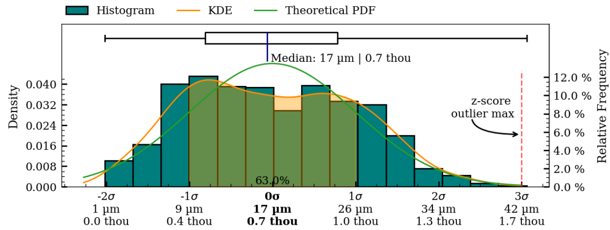
Figure 30: Coaxiality residual plots of interior surface, MV012.
