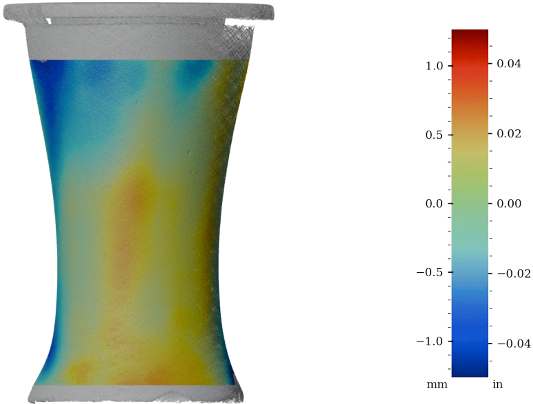
Figure 32: Surface variability heatmap of MV012, rotated 90°
