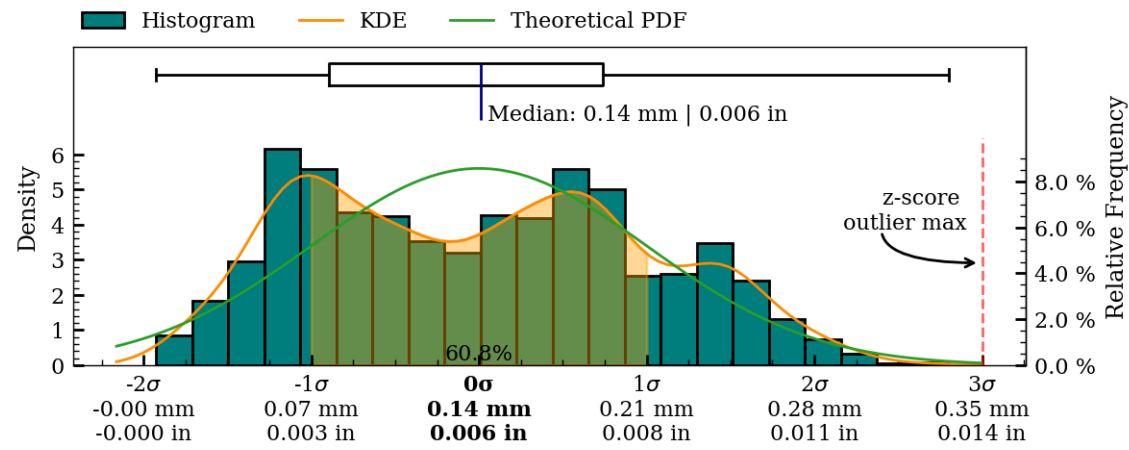
Figure 29: Coaxiality residual plots of exterior surface, MV012.
