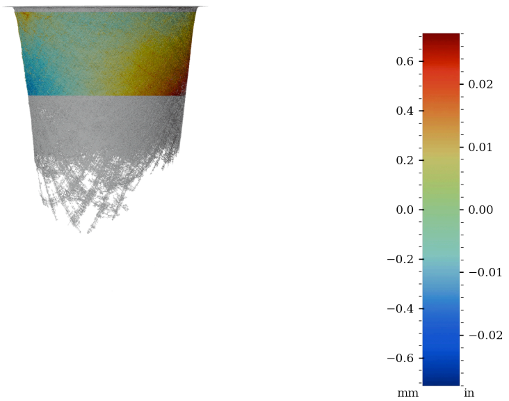
Figure 38: Surface variability heatmap of MV012, rotated 270°
