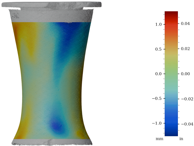
Figure 31: Surface variability heatmap of MV012, front view
