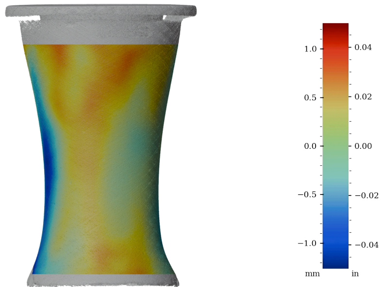
Figure 34: Surface variability heatmap of MV012, rotated 270°
