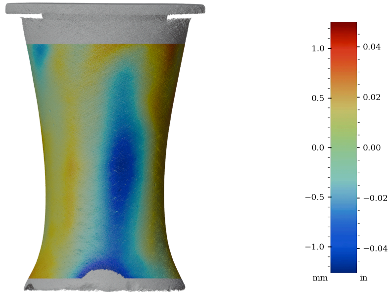
Figure 33: Surface variability heatmap of MV012, rotated 180°
