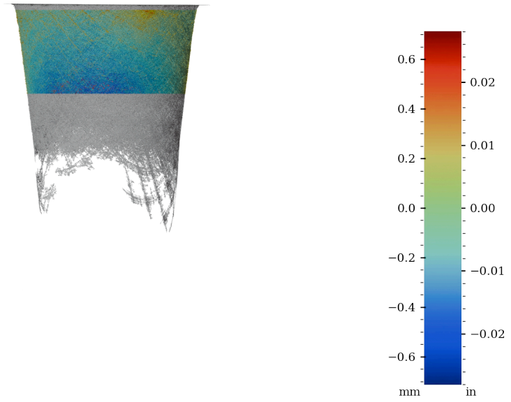
Figure 37: Surface variability heatmap of MV012, rotated 180°
