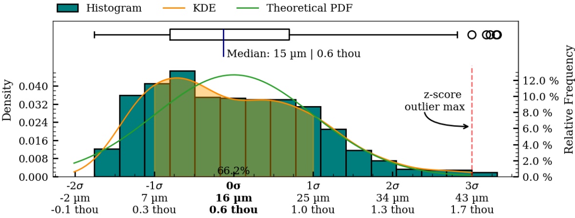
Figure 39: Coaxiality residual plots of interior surface, MV012.
