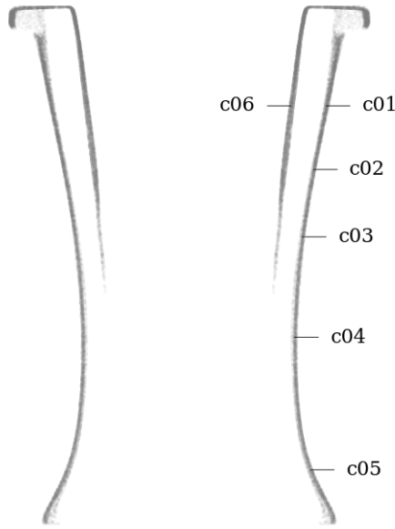
Figure 58: Circularity measurement sample locations, full mesh aligned to exterior surface
