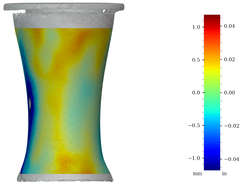
Figure 44: Surface variability heatmap of MV012, rotated 270°
