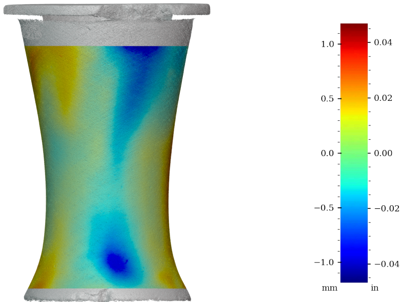
Figure 41: Surface variability heatmap of MV012, front view
