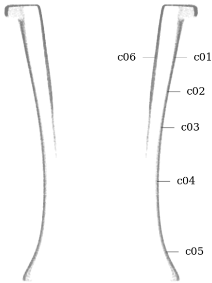
Figure 29: Circularity measurement sample locations, full mesh aligned to exterior surface
