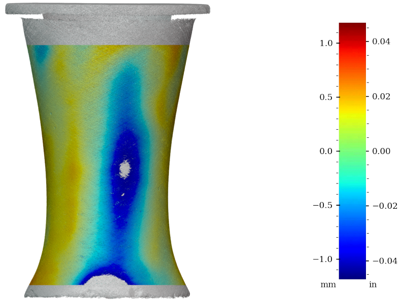
Figure 43: Surface variability heatmap of MV012, rotated 180°
