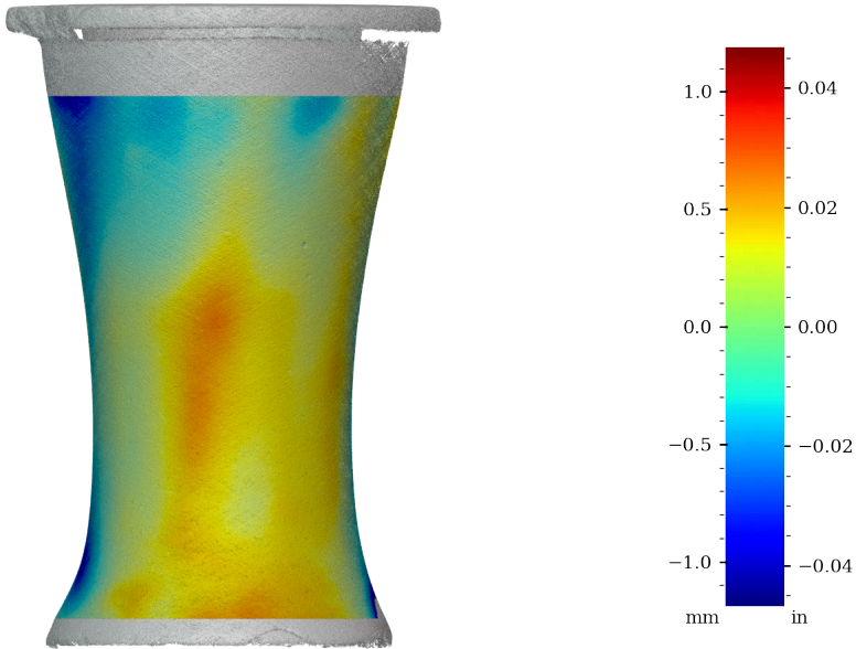
Figure 42: Surface variability heatmap of MV012, rotated 90°
