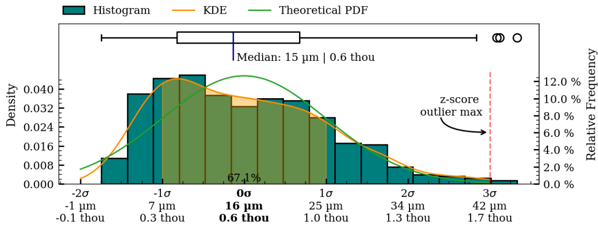
Figure 40: Coaxiality residual plots of interior_separate surface, MV012.
