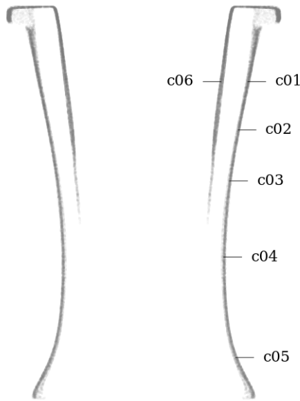
Figure 56: Circularity measurement sample locations, full mesh aligned to exterior surface
