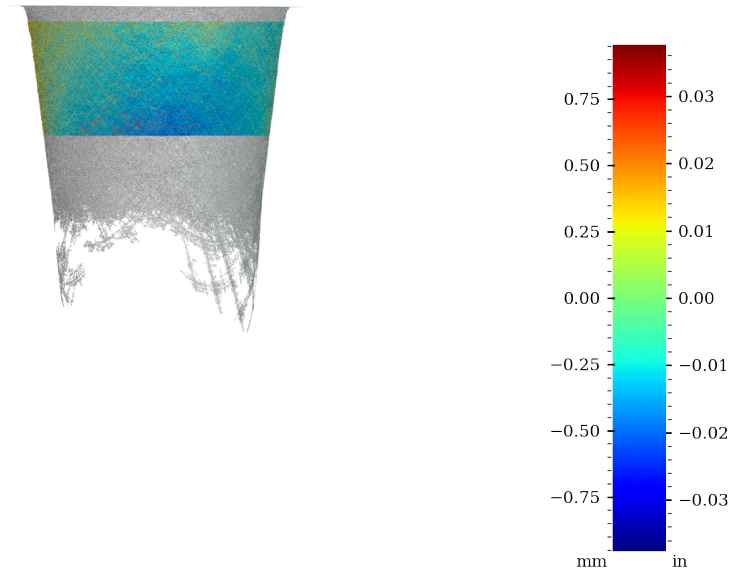
Figure 47: Surface variability heatmap of MV012, rotated 180°
