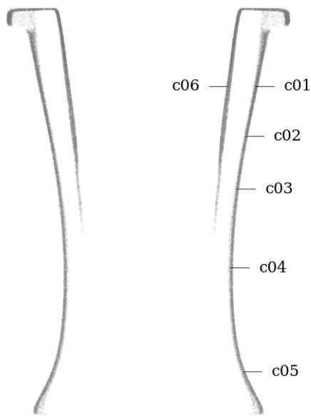
Figure 74: Circularity measurement sample locations, full mesh aligned to exterior surface
