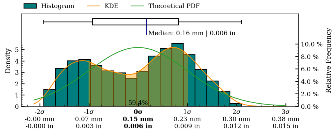
Figure 38: Coaxiality residual plots of exterior surface, MV012.
