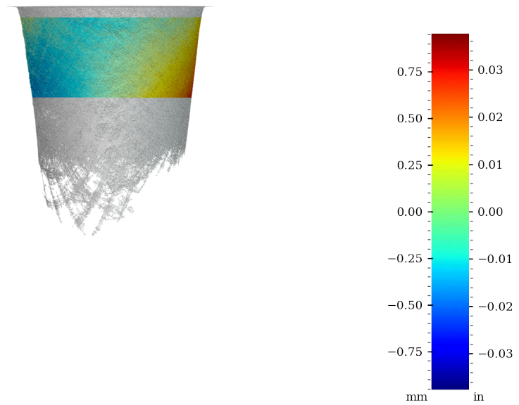
Figure 48: Surface variability heatmap of MV012, rotated 270°
