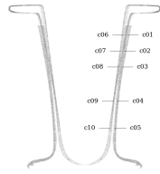
Figure 72: Circularity measurement sample locations, full mesh aligned to exterior surface
