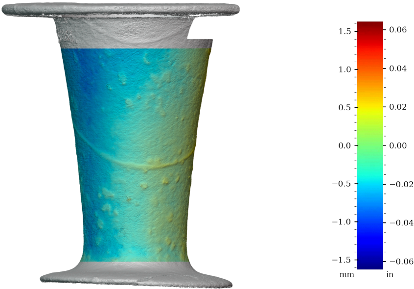
Figure 57: Surface variability heatmap of MV013, front view
