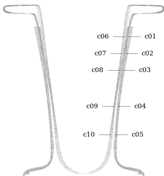
Figure 90: Circularity measurement sample locations, full mesh aligned to exterior surface
