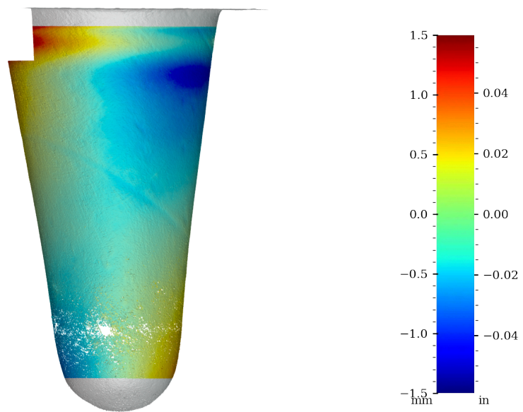
Figure 64: Surface variability heatmap of MV013, rotated 270°
