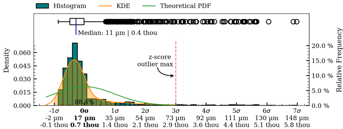
Figure 56: Coaxiality residual plots of interior_separate surface, MV013.
