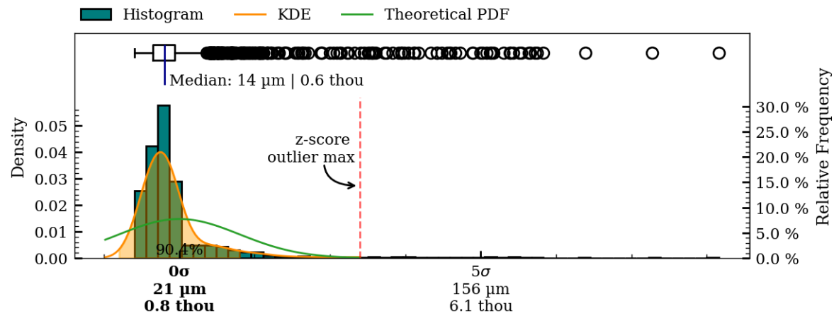
Figure 55: Coaxiality residual plots of interior surface, MV013.
