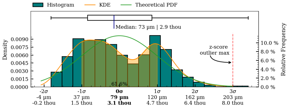
Figure 54: Coaxiality residual plots of exterior surface, MV013.
