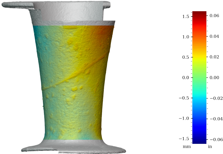
Figure 58: Surface variability heatmap of MV013, rotated 90°
