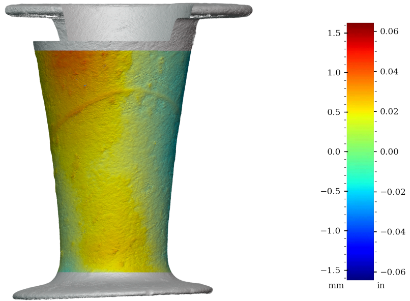
Figure 59: Surface variability heatmap of MV013, rotated 180°
