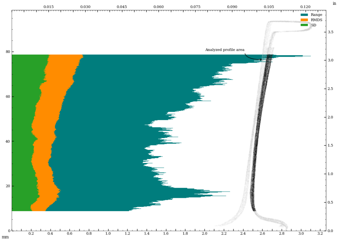
Figure 77: Circularity of exterior surface - in z-plane.
