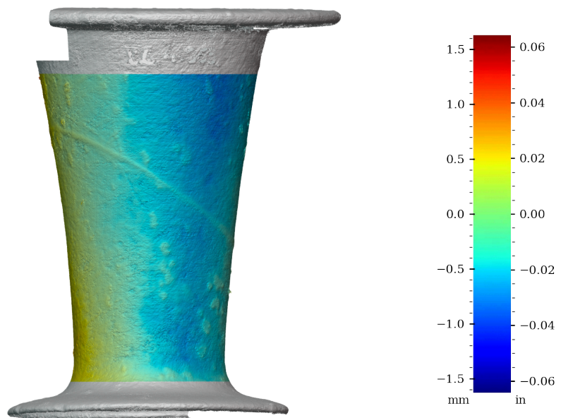
Figure 60: Surface variability heatmap of MV013, rotated 270°
