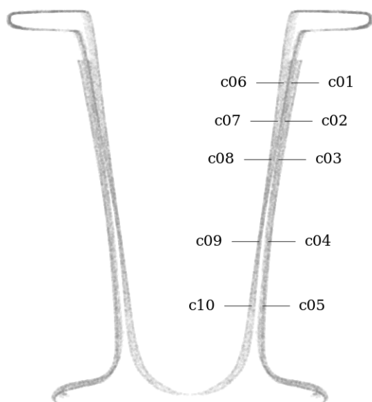
Figure 37: Circularity measurement sample locations, full mesh aligned to exterior surface
