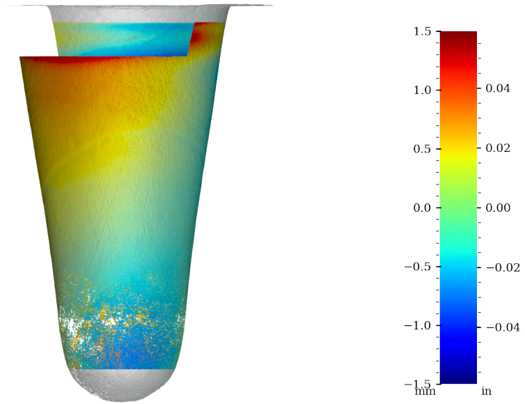
Figure 63: Surface variability heatmap of MV013, rotated 180°
