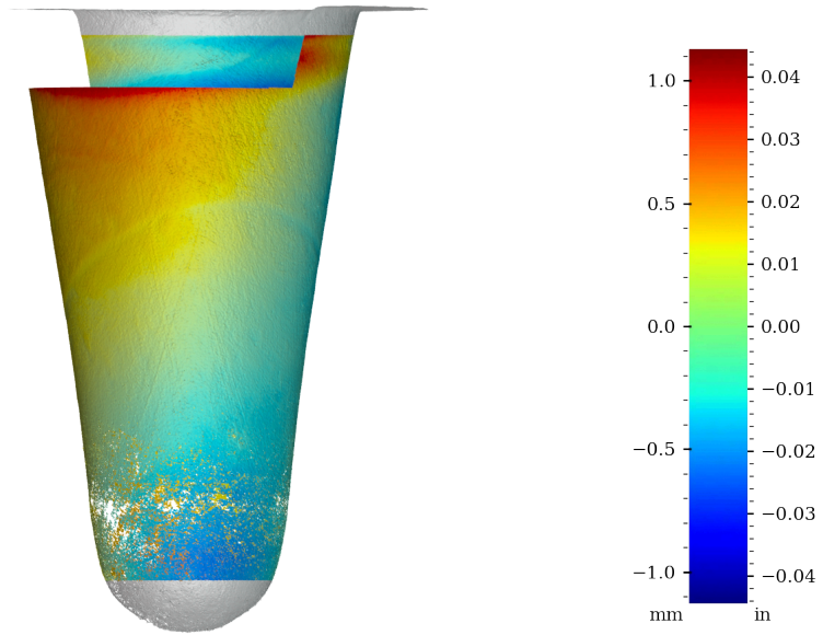
Figure 67: Surface variability heatmap of MV013, rotated 180°
