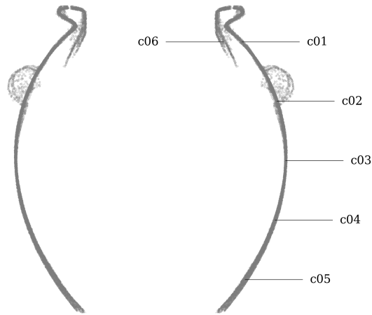
Figure 4: Circularity measurement sample location on MV015.
