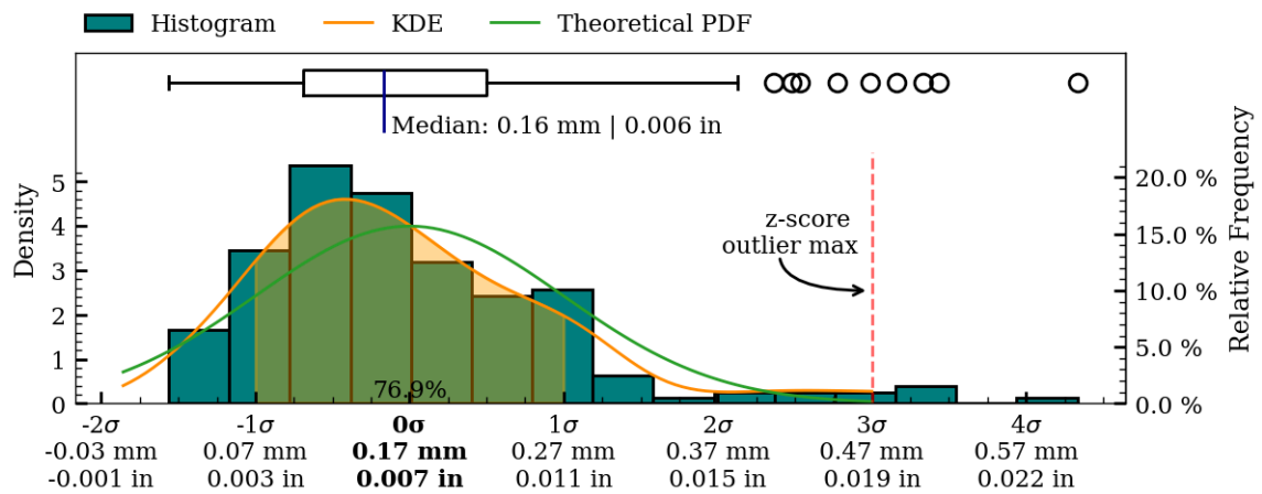
Figure 30: Coaxiality residual plots of interior surface, MV015.
