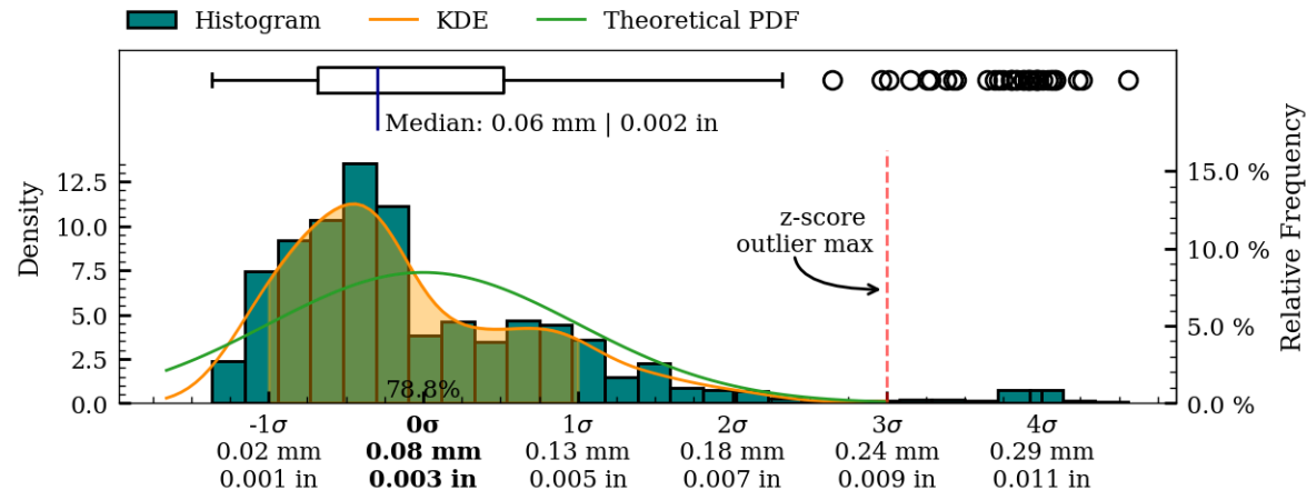
Figure 29: Coaxiality residual plots of exterior surface, MV015.
