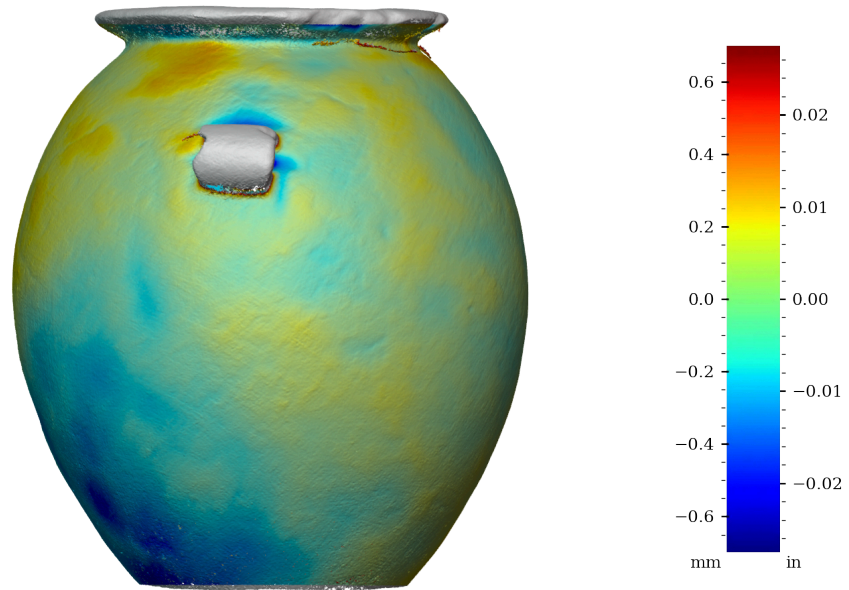
Figure 34: Surface variability heatmap of MV015, rotated 270°
