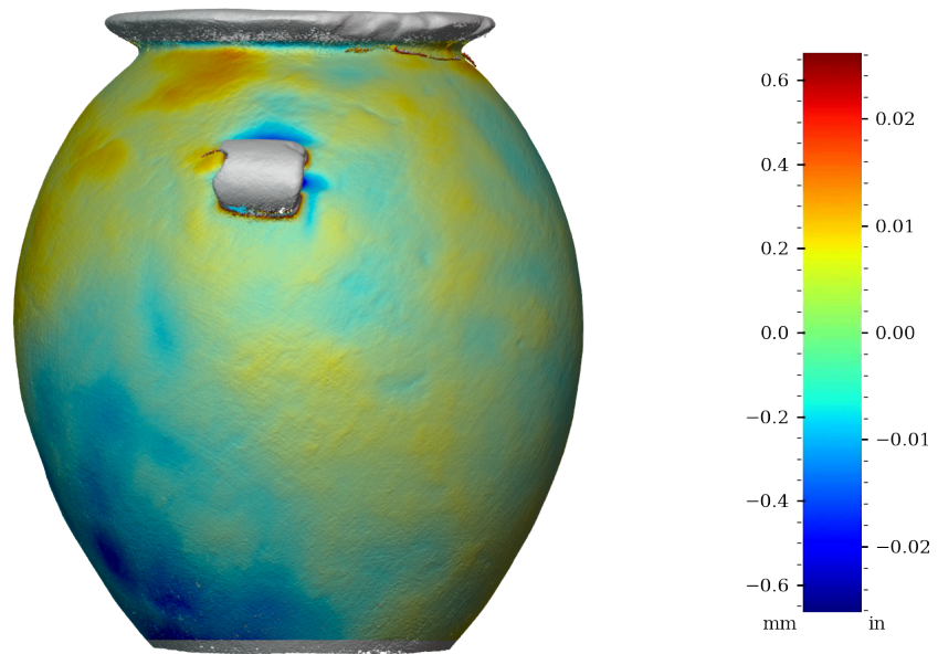
Figure 44: Surface variability heatmap of MV015, rotated 270°
