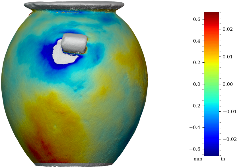
Figure 42: Surface variability heatmap of MV015, rotated 90°
