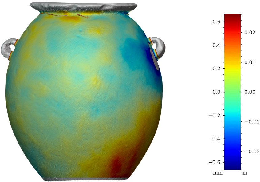
Figure 41: Surface variability heatmap of MV015, front view
