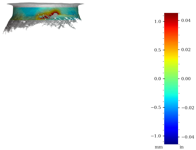
Figure 52: Surface variability heatmap of MV015, rotated 270°
