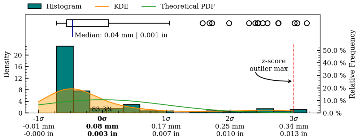
Figure 40: Coaxiality residual plots of interior_separate surface, MV015.
