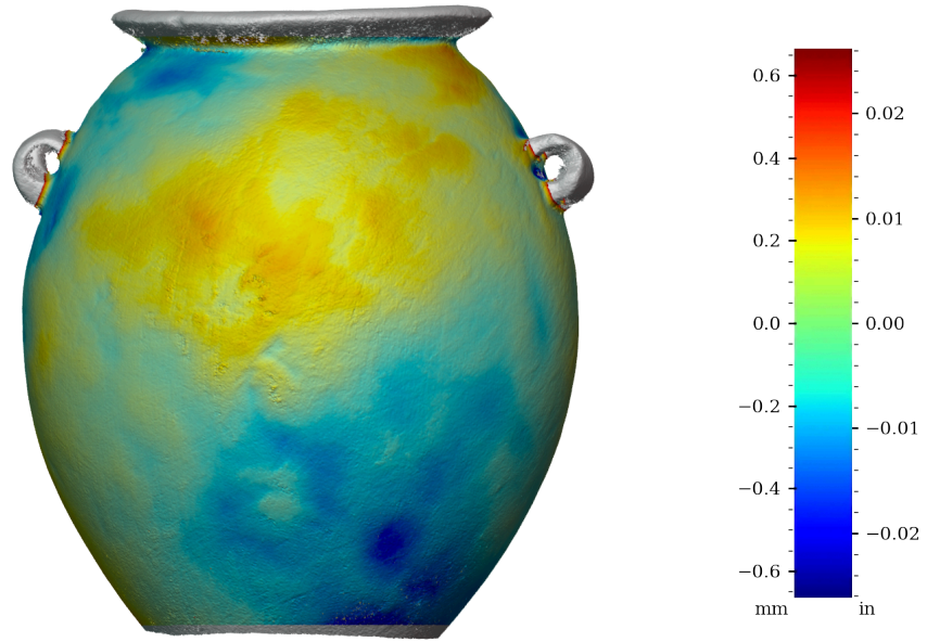
Figure 43: Surface variability heatmap of MV015, rotated 180°
