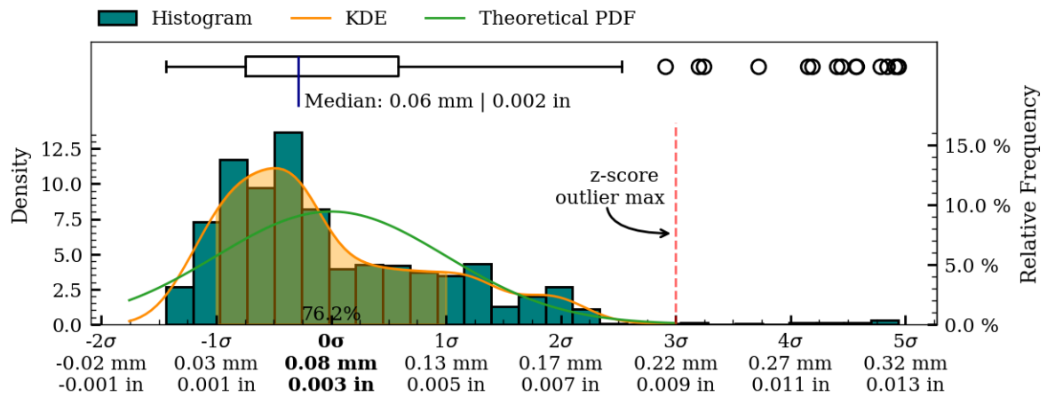
Figure 38: Coaxiality residual plots of exterior surface, MV015.
