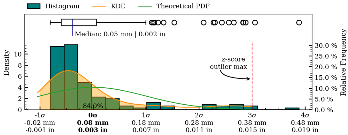
Figure 39: Coaxiality residual plots of interior surface, MV015.
