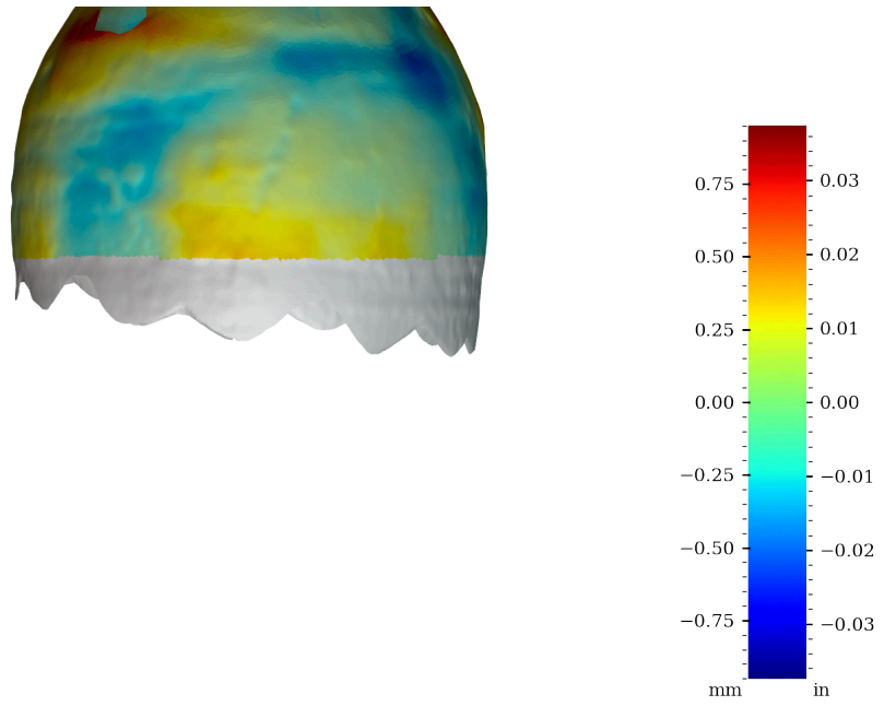
Figure 59: Surface variability heatmap of MV015b, rotated 180°
