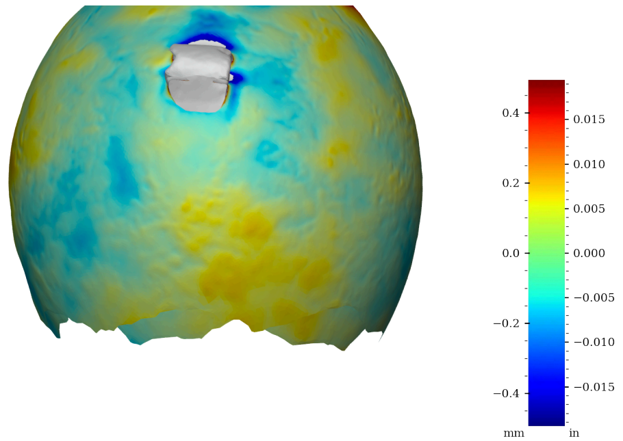
Figure 52: Surface variability heatmap of MV015b, rotated 270°
