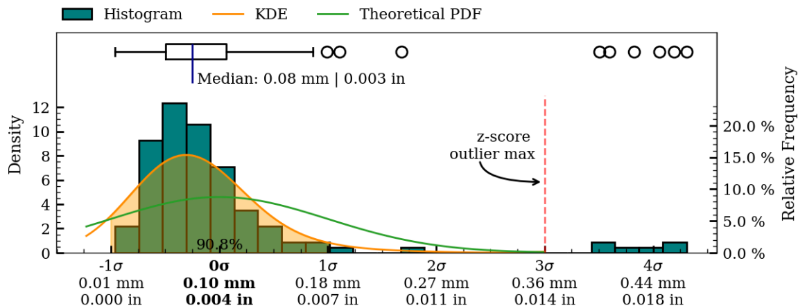
Figure 48: Coaxiality residual plots of interior_separate surface, MV015b.
