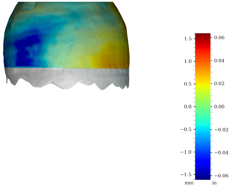
Figure 55: Surface variability heatmap of MV015b, rotated 180°
