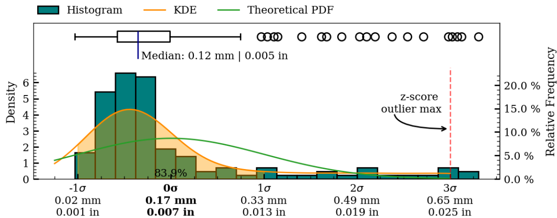
Figure 47: Coaxiality residual plots of interior surface, MV015b.
