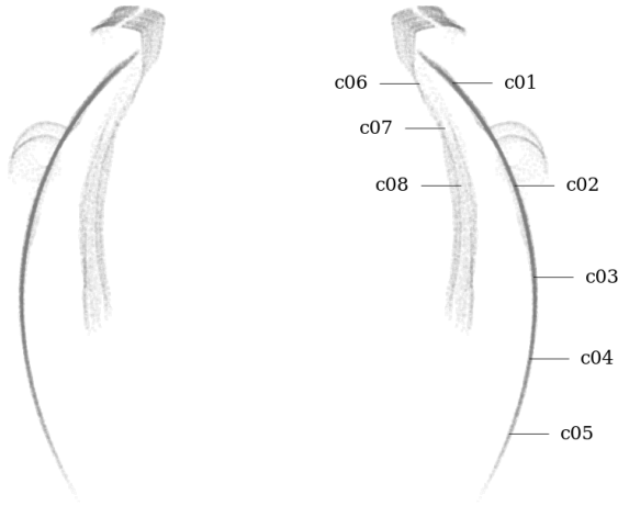
Figure 64: Circularity measurement sample locations, full mesh aligned to exterior surface
