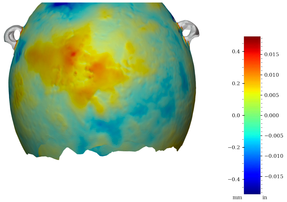
Figure 51: Surface variability heatmap of MV015b, rotated 180°
