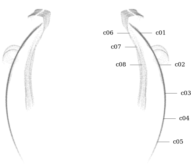
Figure 66: Circularity measurement sample locations, full mesh aligned to exterior surface
