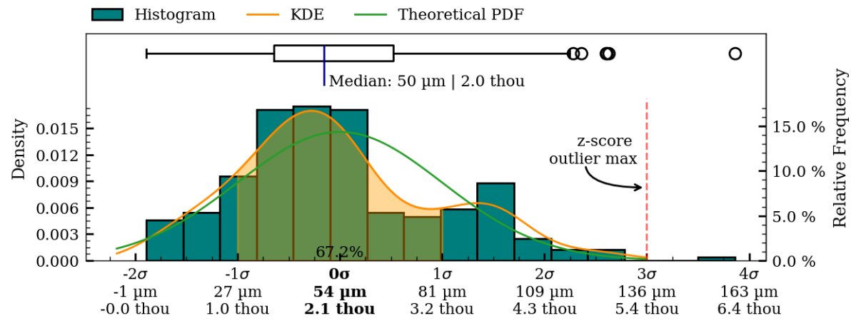
Figure 46: Coaxiality residual plots of exterior surface, MV015b.
