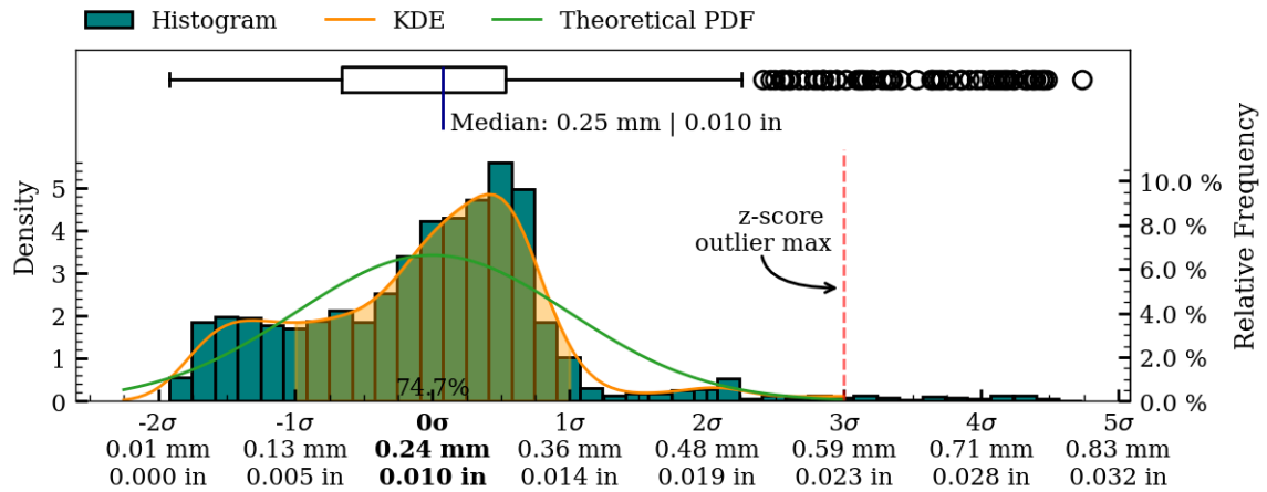
Figure 29: Coaxiality residual plots of exterior surface, MV016.
