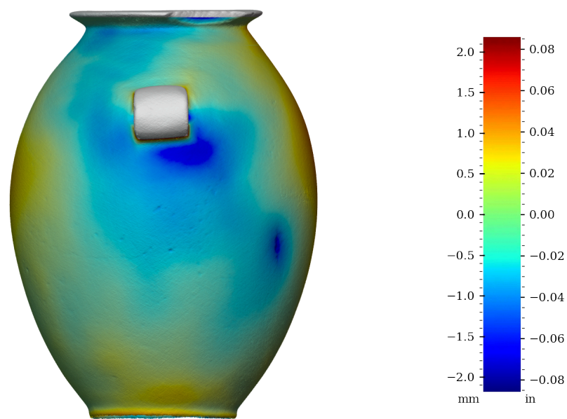
Figure 32: Surface variability heatmap of MV016, rotated 90°
