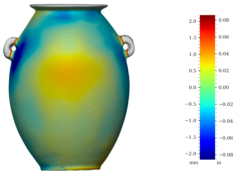
Figure 31: Surface variability heatmap of MV016, front view
