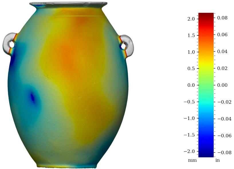
Figure 33: Surface variability heatmap of MV016, rotated 180°
