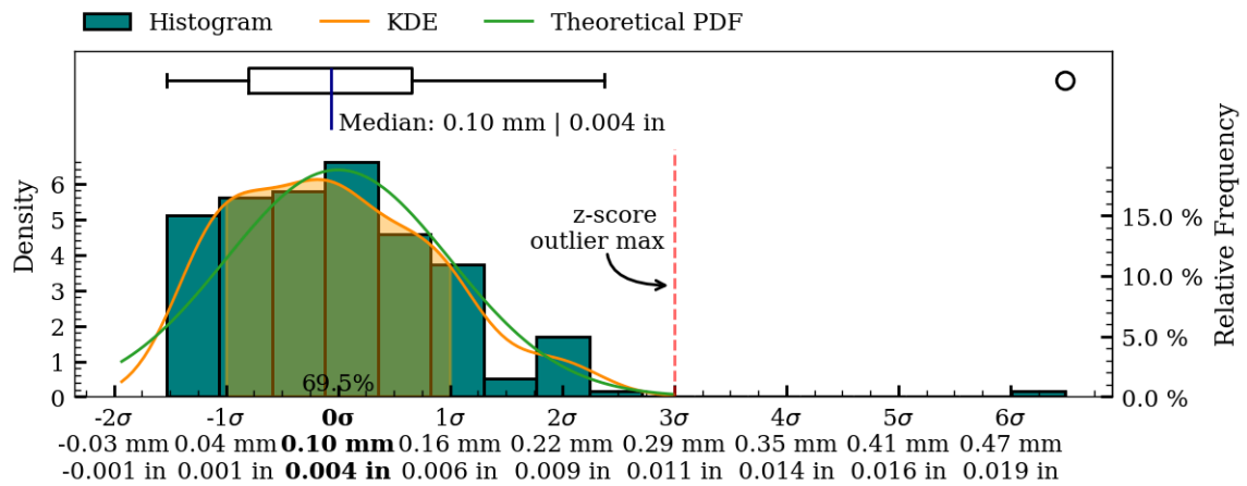
Figure 30: Coaxiality residual plots of interior surface, MV016.
