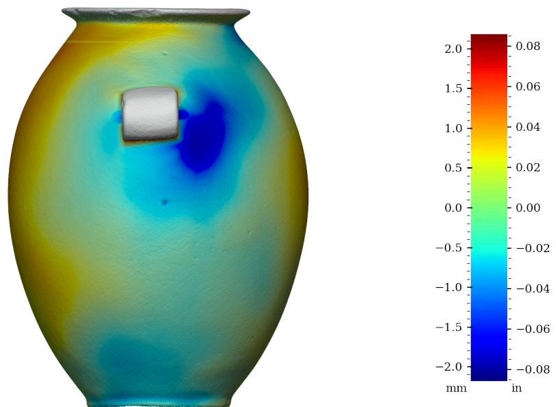
Figure 34: Surface variability heatmap of MV016, rotated 270°
