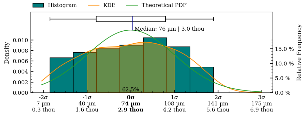
Figure 39: Coaxiality residual plots of interior surface, MV016.
