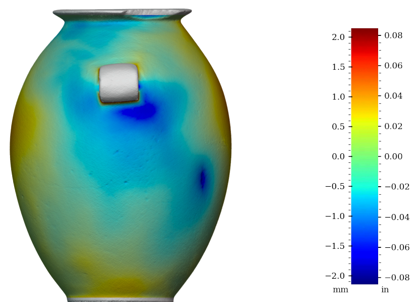
Figure 42: Surface variability heatmap of MV016, rotated 90°
