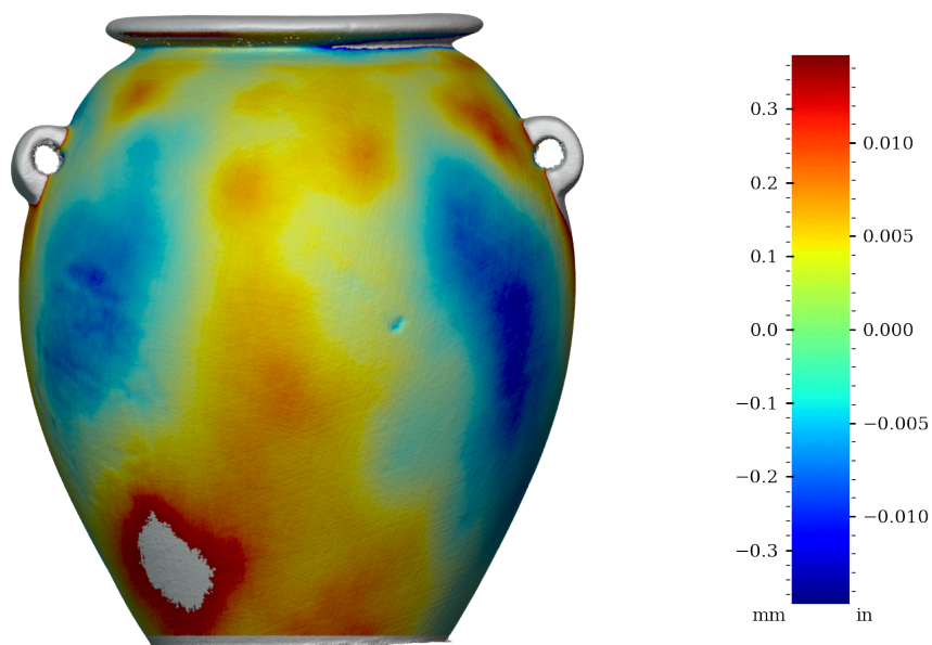
Figure 31: Surface variability heatmap of MV017, front view
