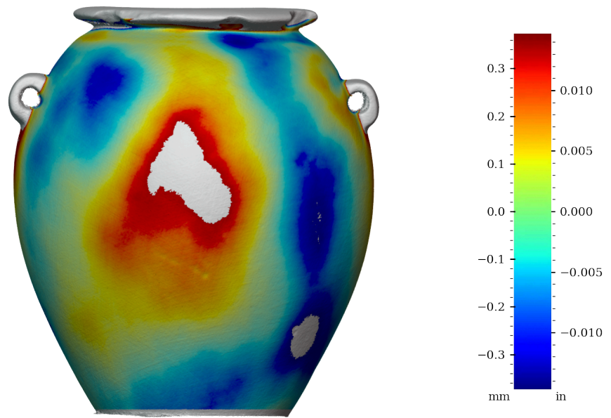
Figure 33: Surface variability heatmap of MV017, rotated 180°
