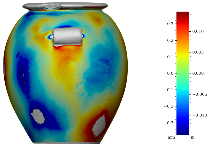
Figure 34: Surface variability heatmap of MV017, rotated 270°
