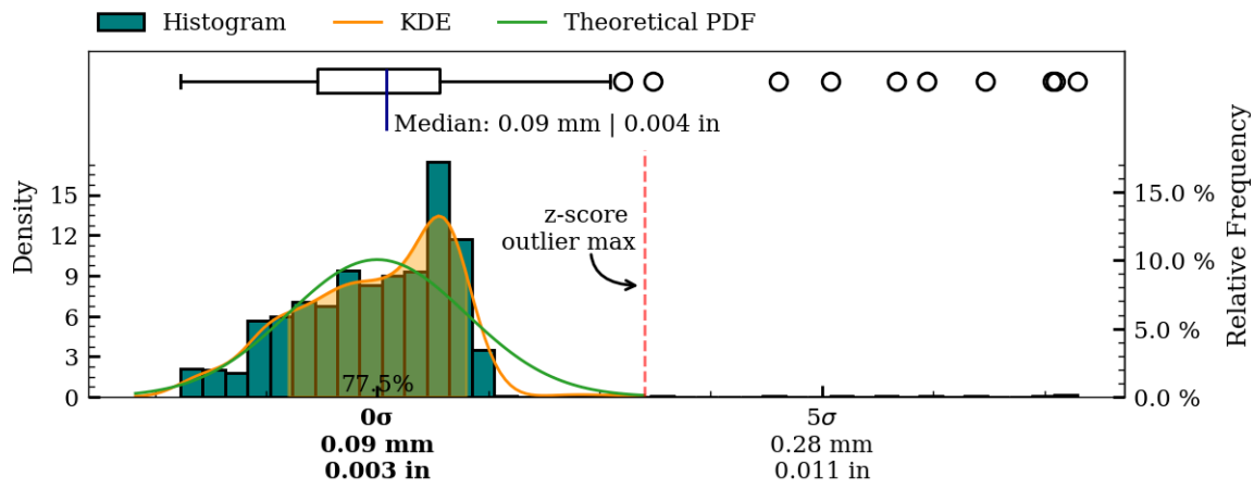
Figure 29: Coaxiality residual plots of exterior surface, MV017.
