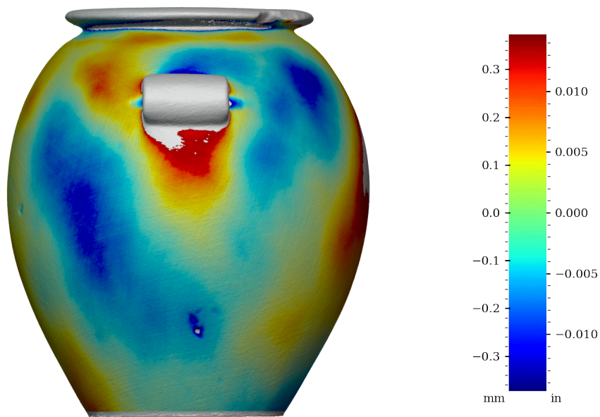
Figure 32: Surface variability heatmap of MV017, rotated 90°
