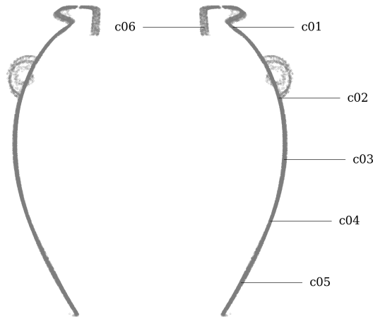
Figure 4: Circularity measurement sample location on MV017.
