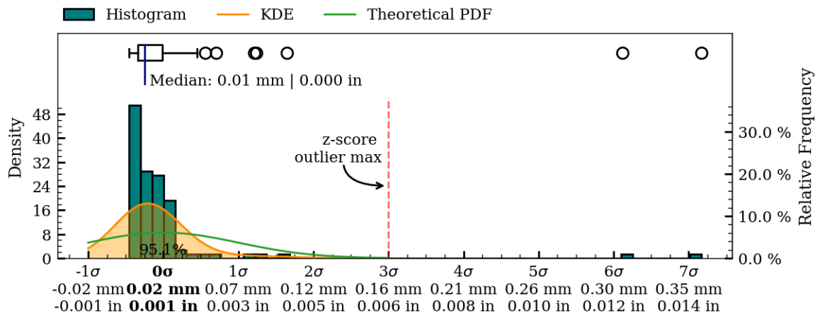
Figure 30: Coaxiality residual plots of interior surface, MV017.
