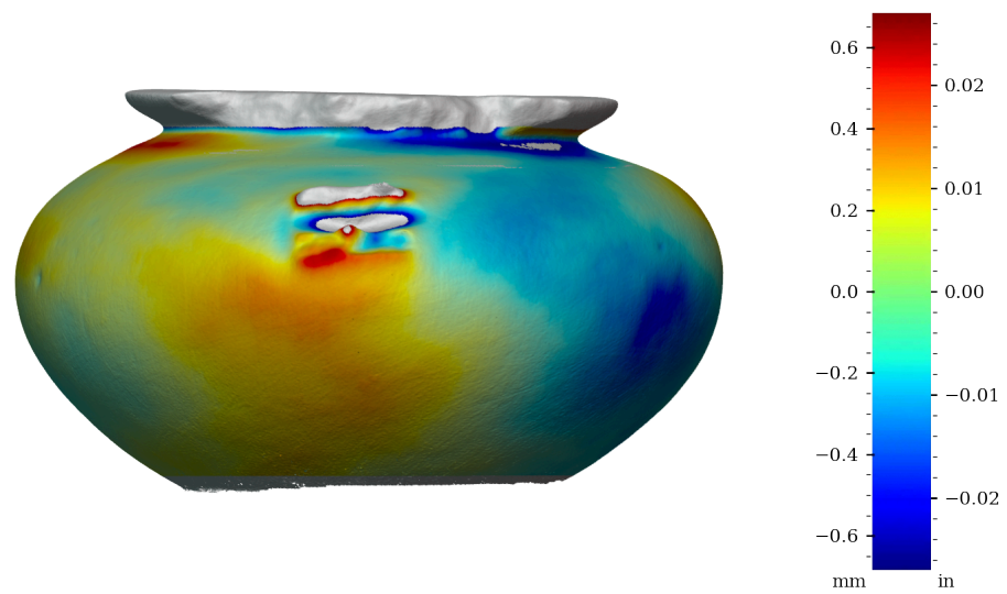
Figure 44: Surface variability heatmap of MV018, rotated 270°
