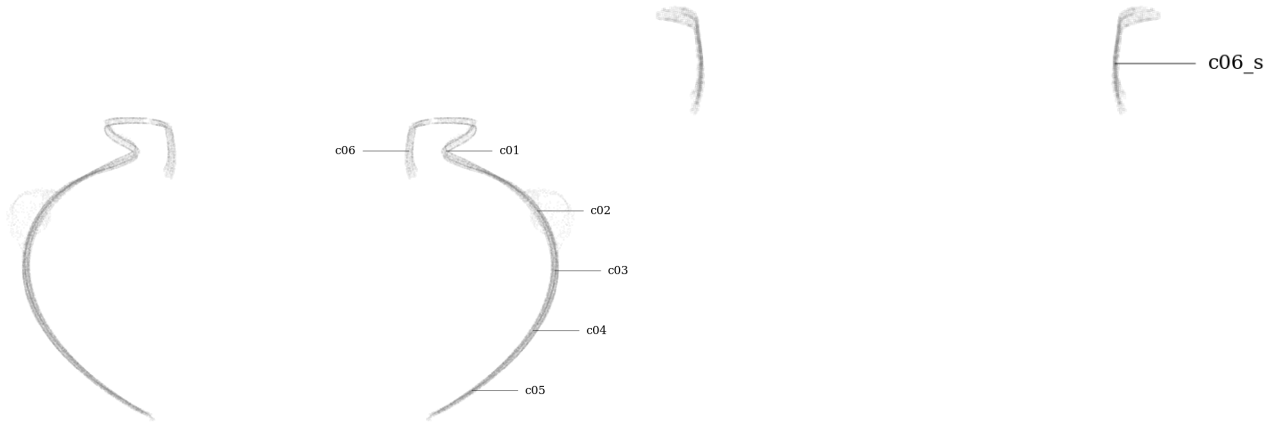
Figure 56: Circularity measurement sample locations, full mesh aligned to exterior surface
