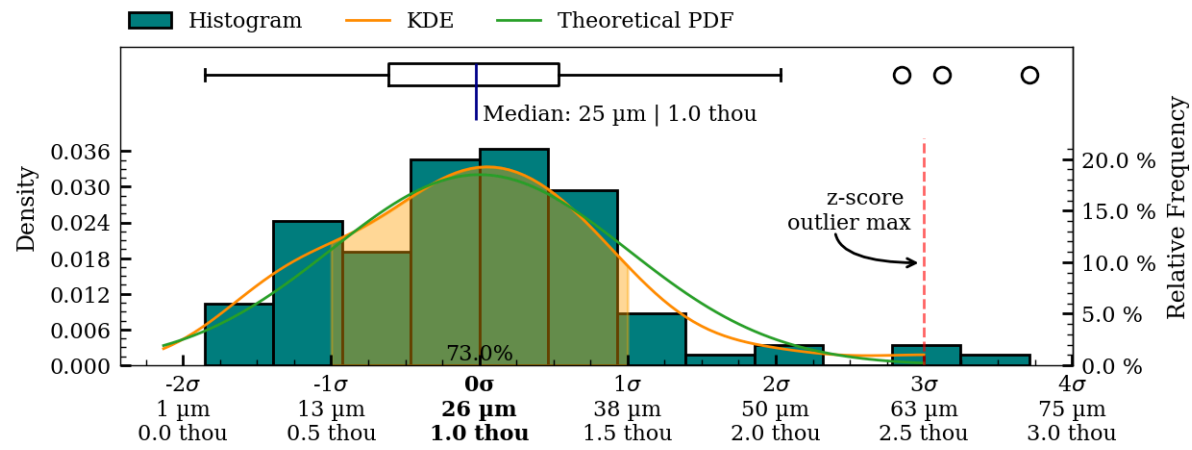
Figure 39: Coaxiality residual plots of interior surface, MV018.
