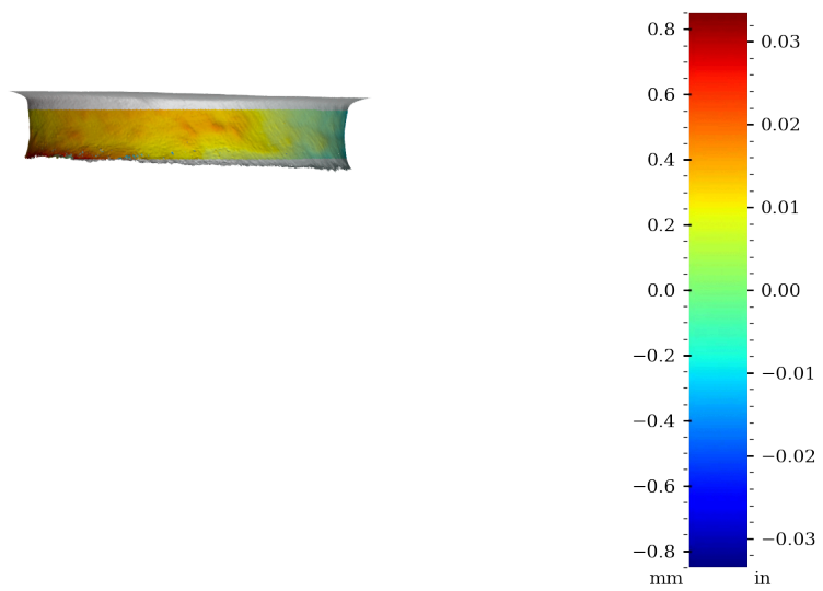
Figure 48: Surface variability heatmap of MV018, rotated 270°
