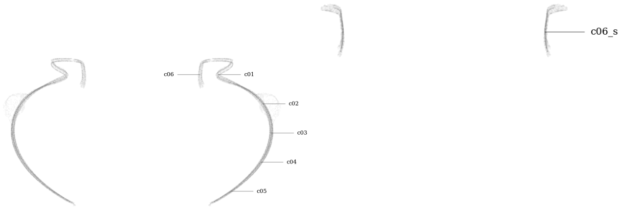
Figure 72: Circularity measurement sample locations, full mesh aligned to exterior surface
