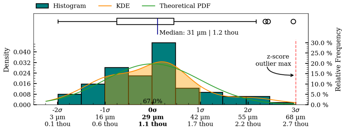
Figure 40: Coaxiality residual plots of interior_separate surface, MV018.
