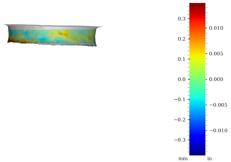
Figure 52: Surface variability heatmap of MV018, rotated 270°
