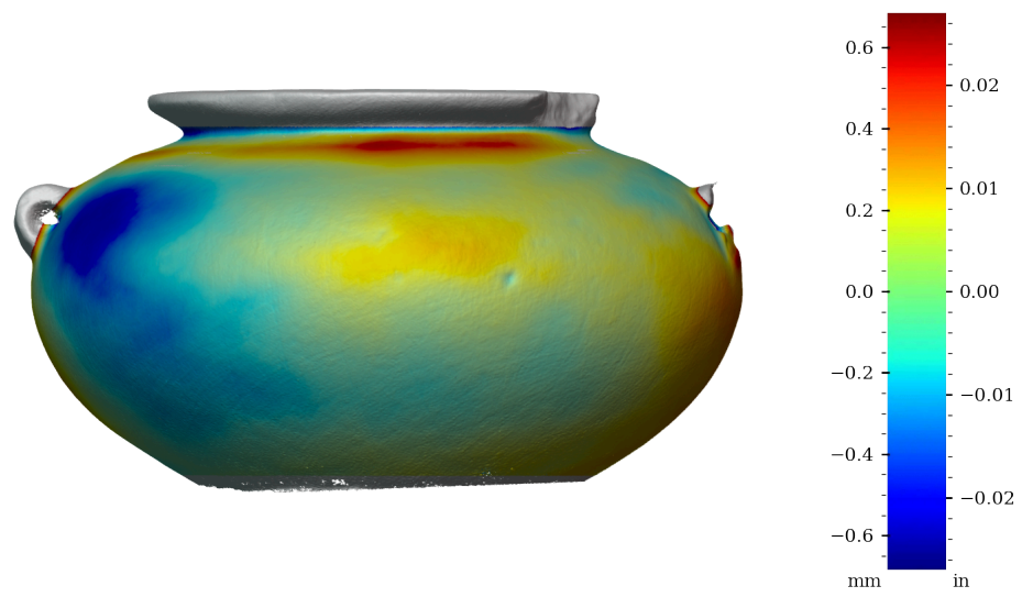
Figure 43: Surface variability heatmap of MV018, rotated 180°
