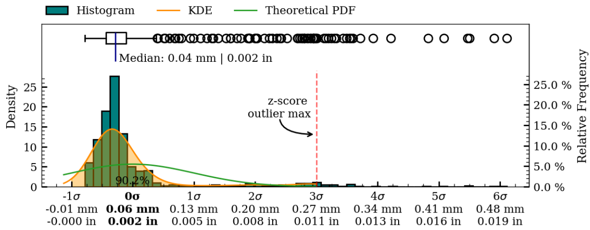
Figure 38: Coaxiality residual plots of exterior surface, MV018.
