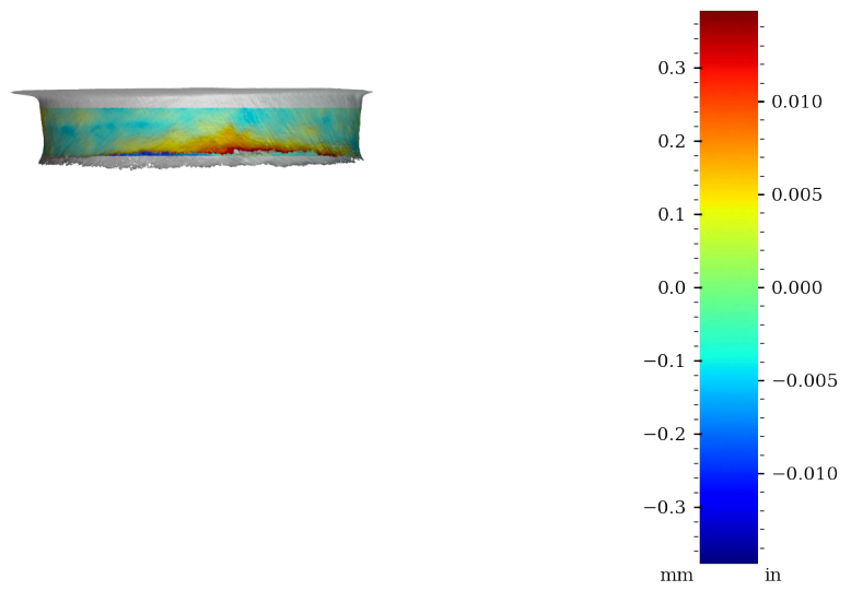
Figure 51: Surface variability heatmap of MV018, rotated 180°
