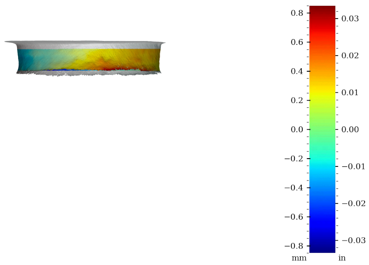
Figure 47: Surface variability heatmap of MV018, rotated 180°
