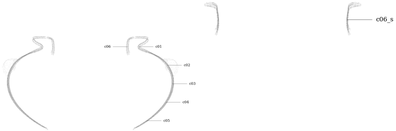
Figure 58: Circularity measurement sample locations, full mesh aligned to exterior surface
