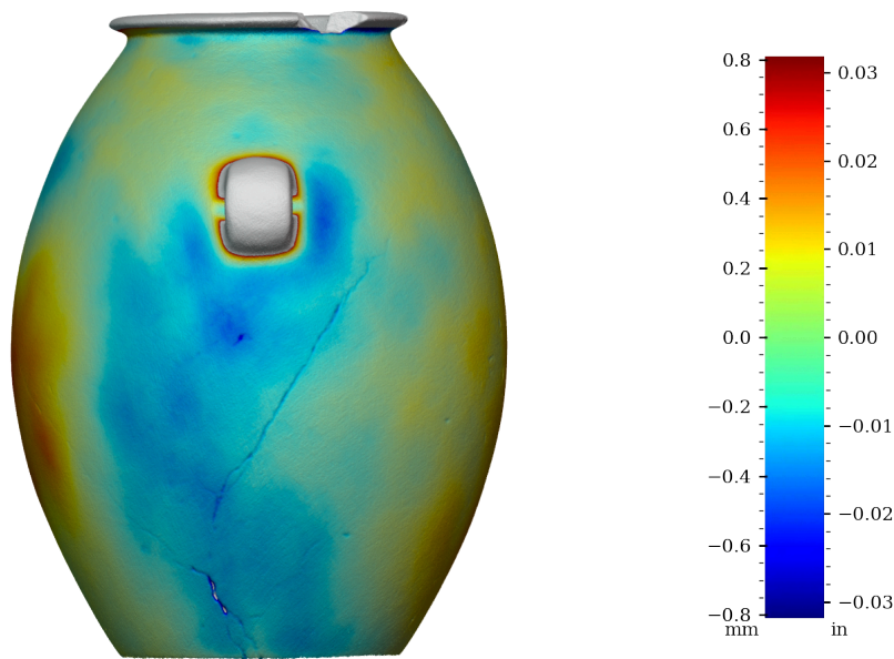
Figure 32: Surface variability heatmap of MV019, rotated 90°
