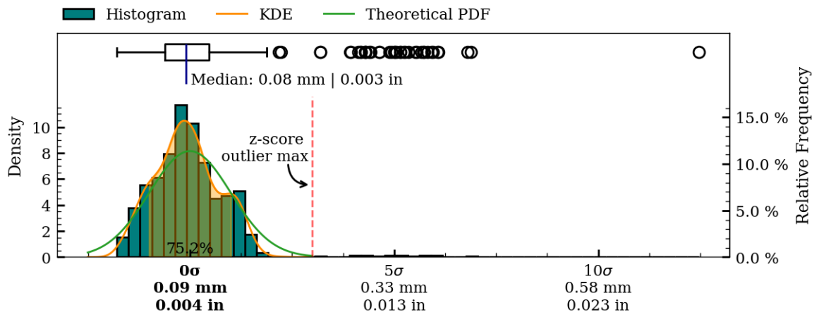
Figure 29: Coaxiality residual plots of exterior surface, MV019.
