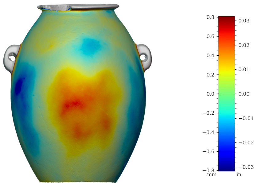
Figure 31: Surface variability heatmap of MV019, front view
