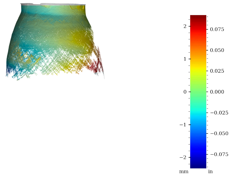
Figure 38: Surface variability heatmap of MV019, rotated 270°
