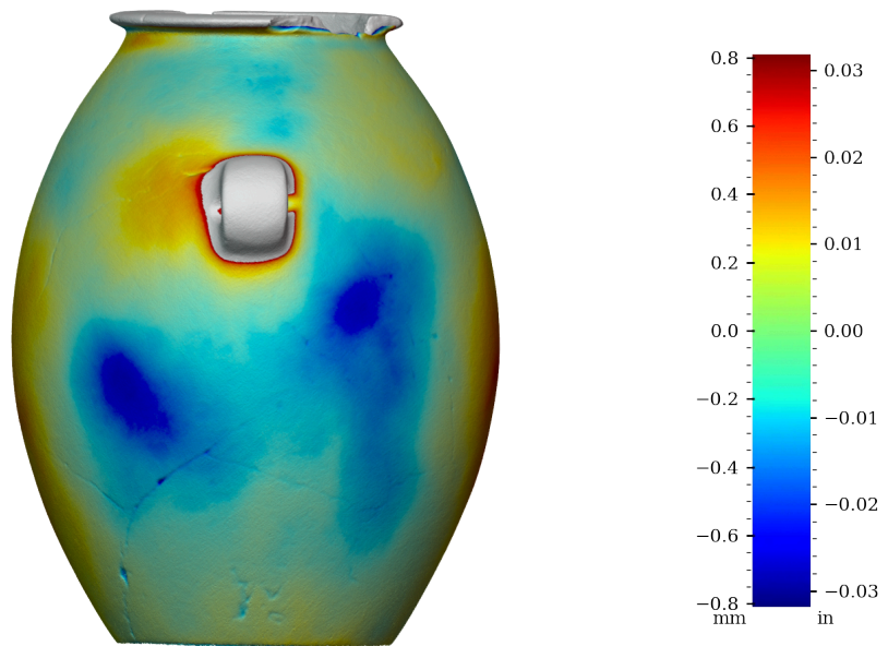
Figure 34: Surface variability heatmap of MV019, rotated 270°
