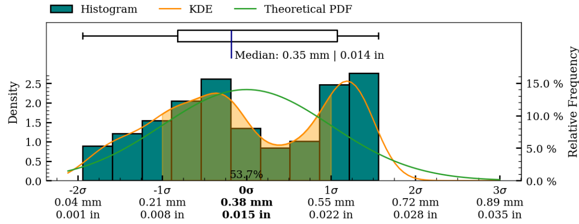
Figure 30: Coaxiality residual plots of interior surface, MV019.
