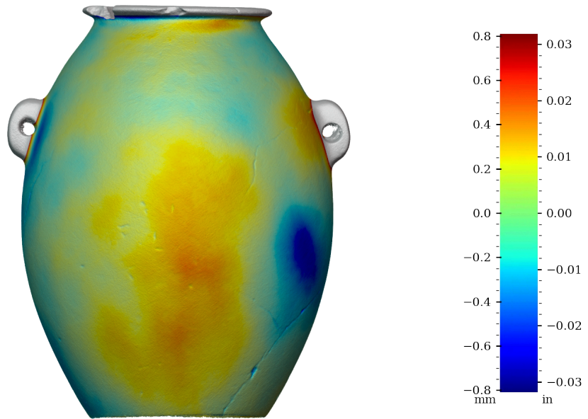
Figure 33: Surface variability heatmap of MV019, rotated 180°
