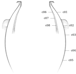
Figure 80: Circularity measurement sample locations, full mesh aligned to exterior surface
