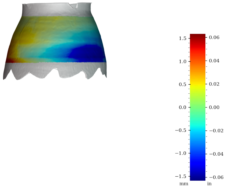
Figure 56: Surface variability heatmap of MV019b, rotated 270°
