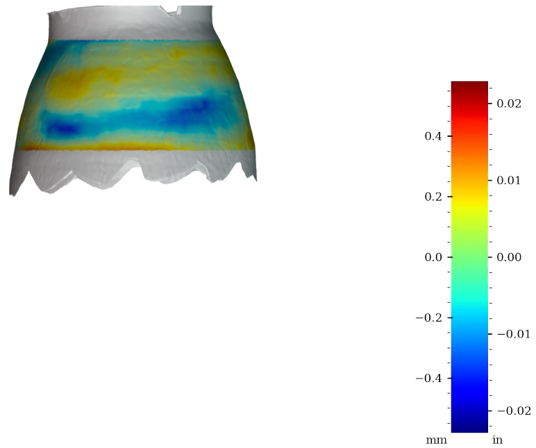
Figure 60: Surface variability heatmap of MV019b, rotated 270°
