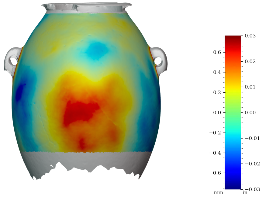
Figure 51: Surface variability heatmap of MV019b, rotated 180°
