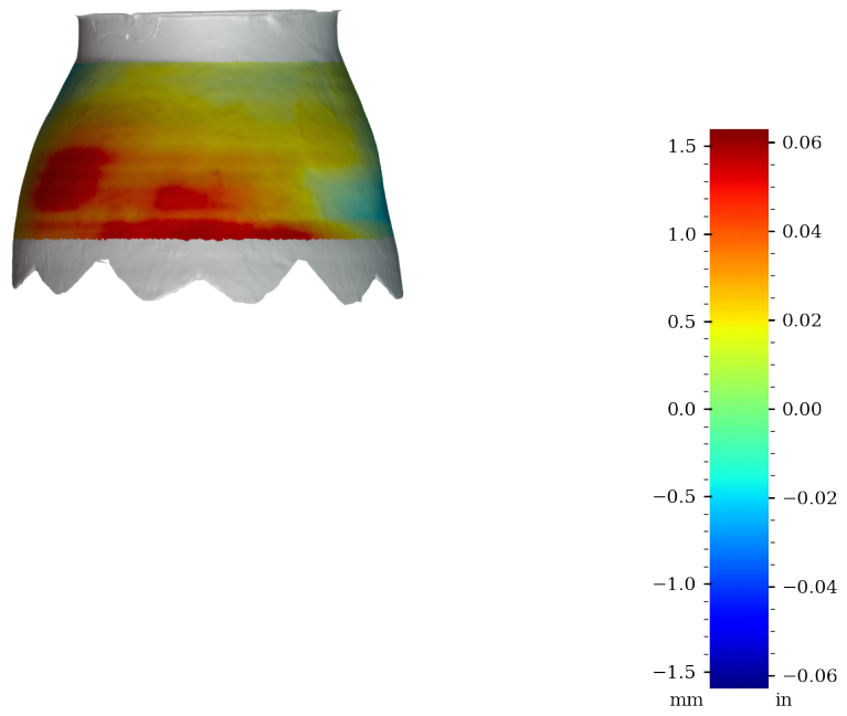
Figure 55: Surface variability heatmap of MV019b, rotated 180°
