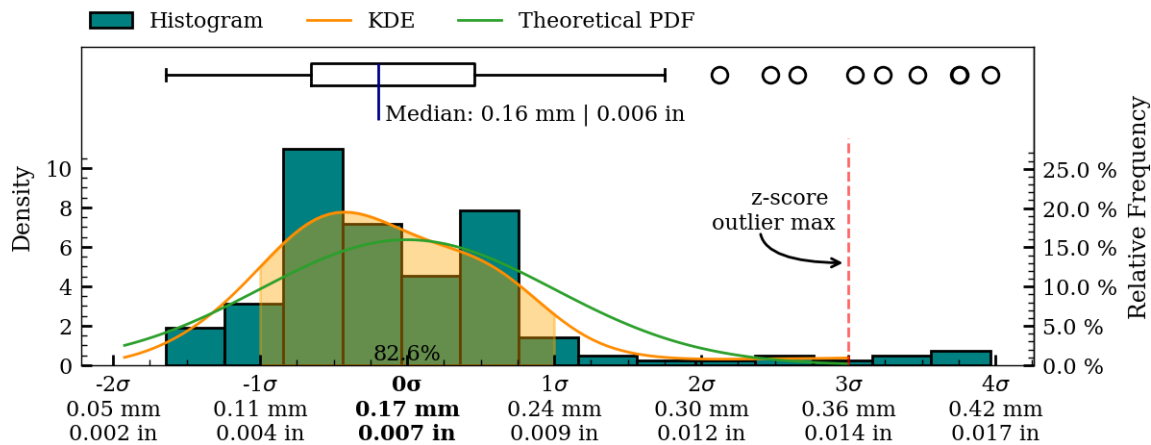
Figure 48: Coaxiality residual plots of interior_separate surface, MV019b.
