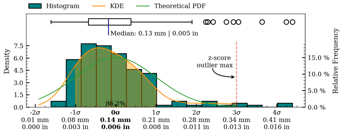
Figure 47: Coaxiality residual plots of interior surface, MV019b.
