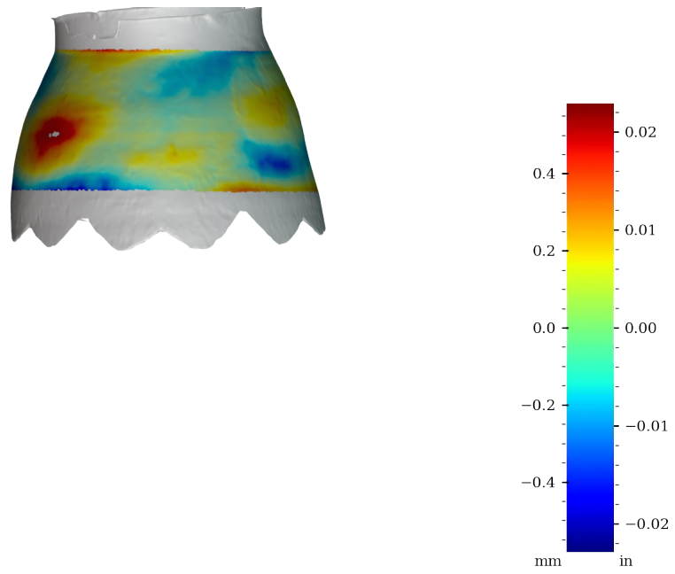
Figure 59: Surface variability heatmap of MV019b, rotated 180°
