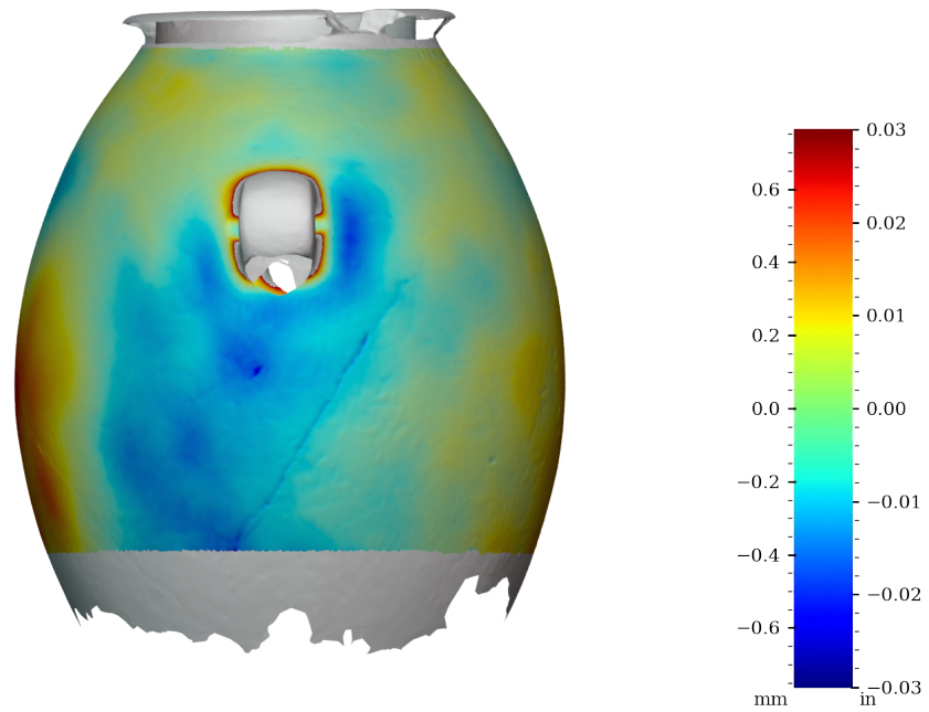
Figure 52: Surface variability heatmap of MV019b, rotated 270°
