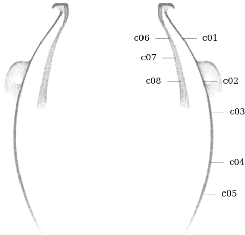
Figure 64: Circularity measurement sample locations, full mesh aligned to exterior surface
