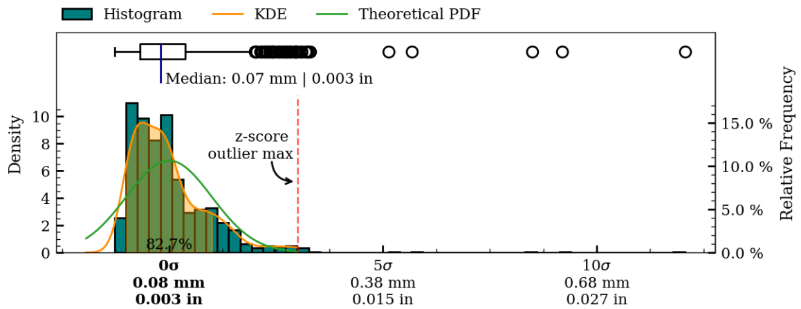
Figure 29: Coaxiality residual plots of exterior surface, MV020.
