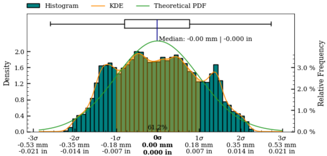
Figure 40: Interior surface variability boxplot, kds and histogram.
