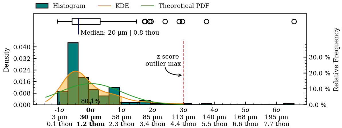
Figure 30: Coaxiality residual plots of interior surface, MV020.
