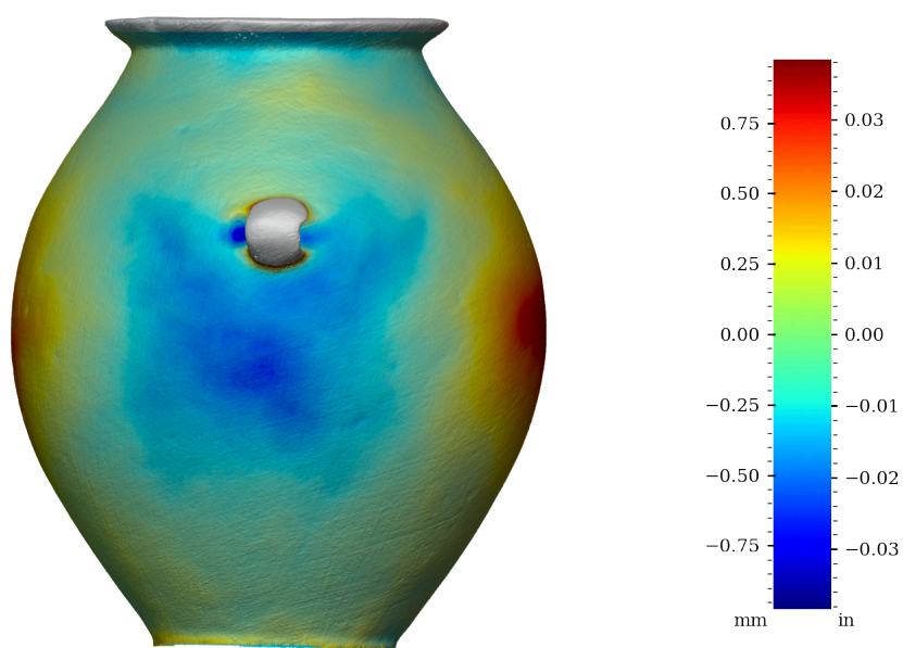
Figure 34: Surface variability heatmap of MV020, rotated 270°
