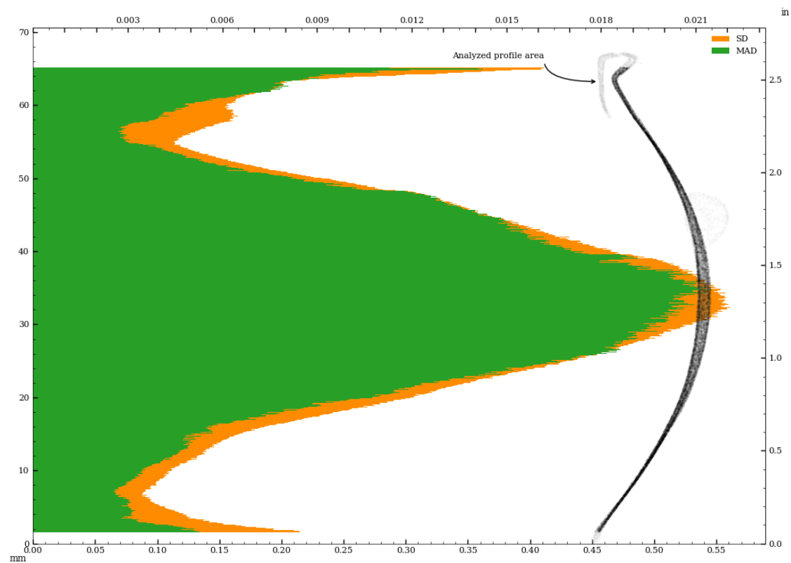
Figure 44: Circularity analysis of exterior surface - in z-plane
