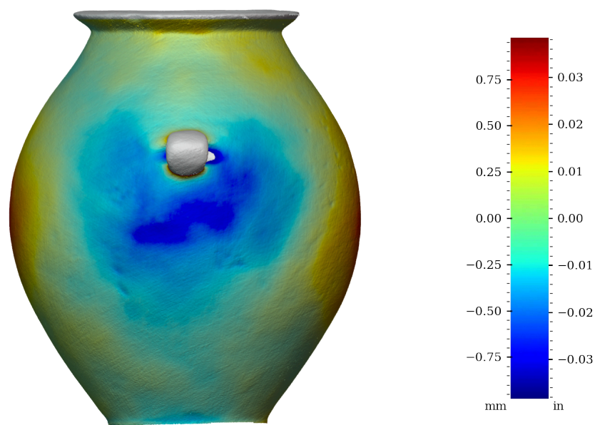
Figure 32: Surface variability heatmap of MV020, rotated 90°
