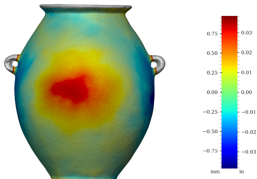
Figure 31: Surface variability heatmap of MV020, front view
