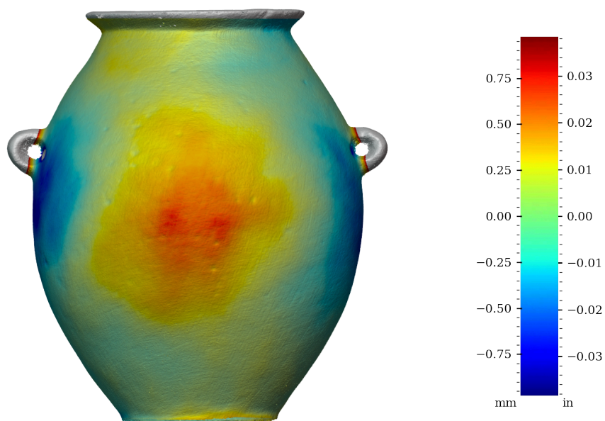
Figure 33: Surface variability heatmap of MV020, rotated 180°
