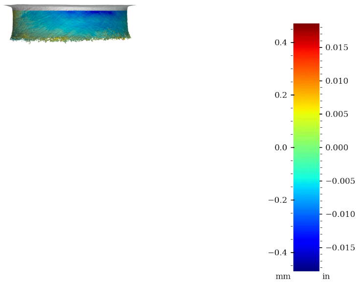
Figure 38: Surface variability heatmap of MV020, rotated 270°
