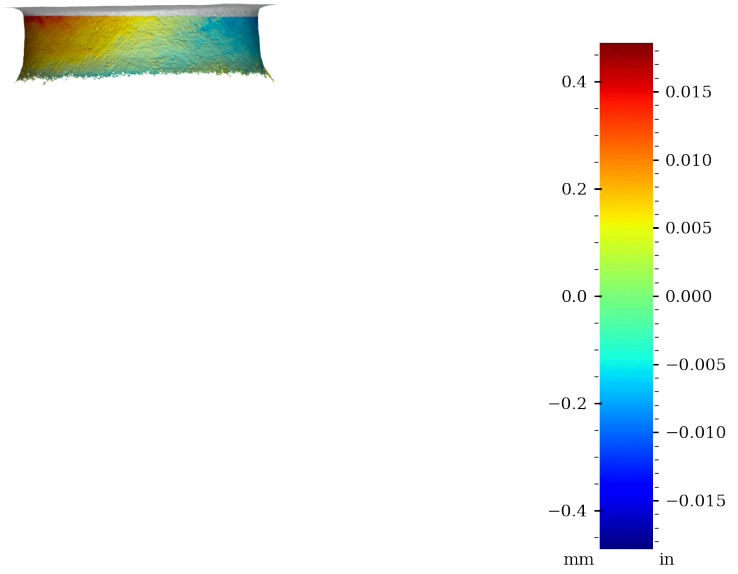
Figure 37: Surface variability heatmap of MV020, rotated 180°
