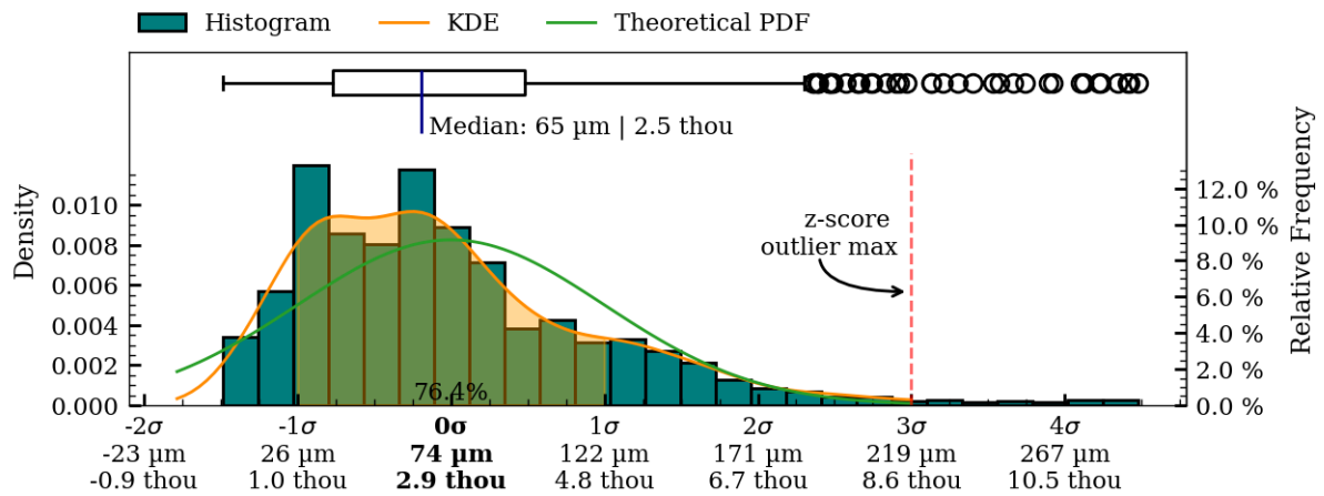
Figure 38: Coaxiality residual plots of exterior surface, MV020.
