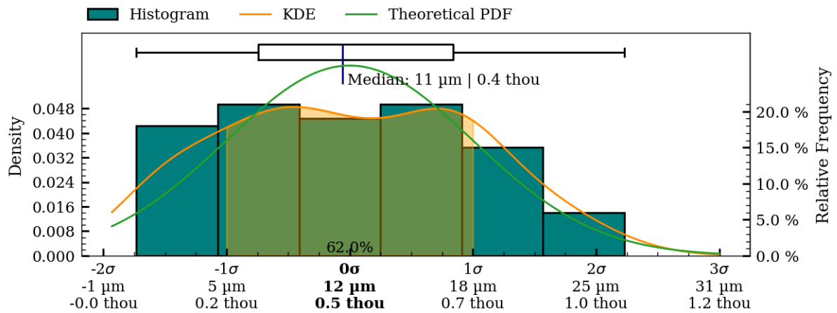
Figure 40: Coaxiality residual plots of interior_separate surface, MV020.
