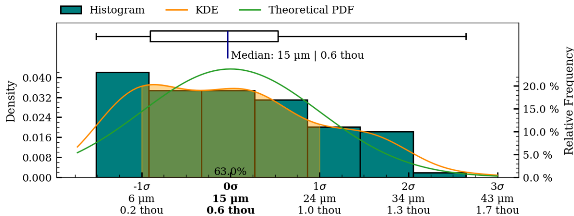
Figure 39: Coaxiality residual plots of interior surface, MV020.
