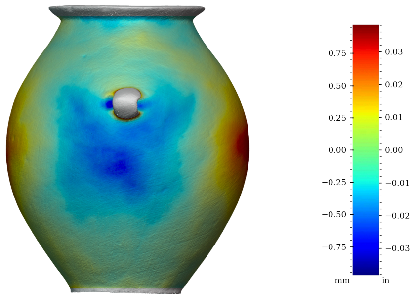
Figure 44: Surface variability heatmap of MV020, rotated 270°
