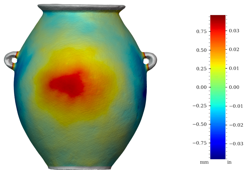
Figure 41: Surface variability heatmap of MV020, front view
