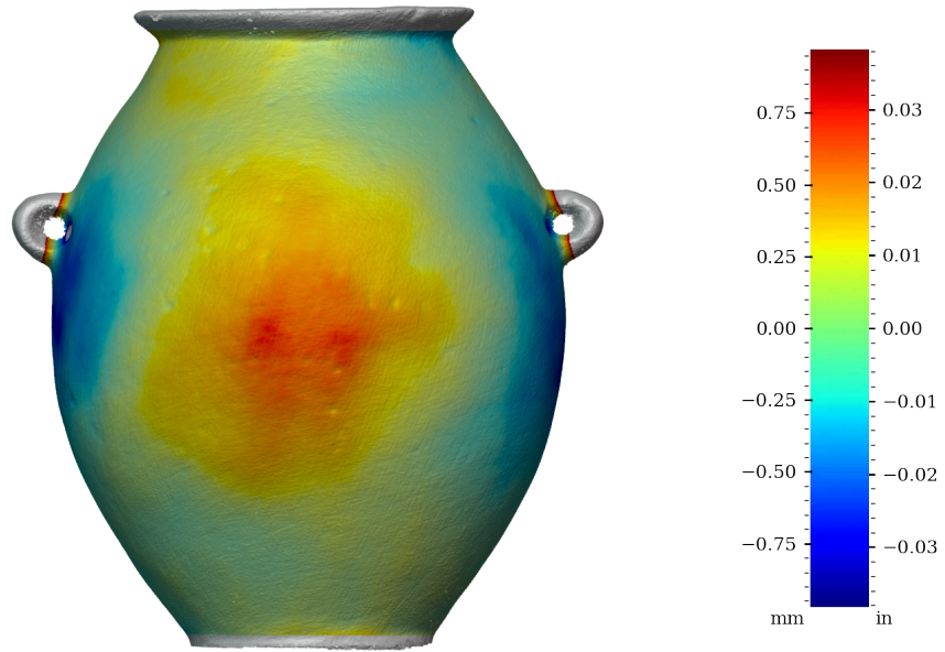
Figure 43: Surface variability heatmap of MV020, rotated 180°
