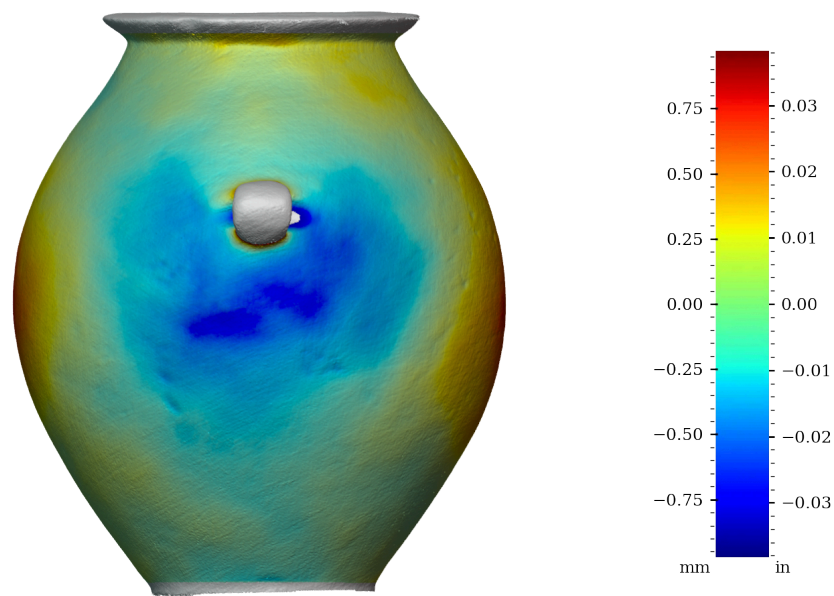
Figure 42: Surface variability heatmap of MV020, rotated 90°
