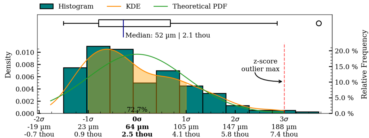
Figure 38: Coaxiality residual plots of exterior surface, MV020b.
