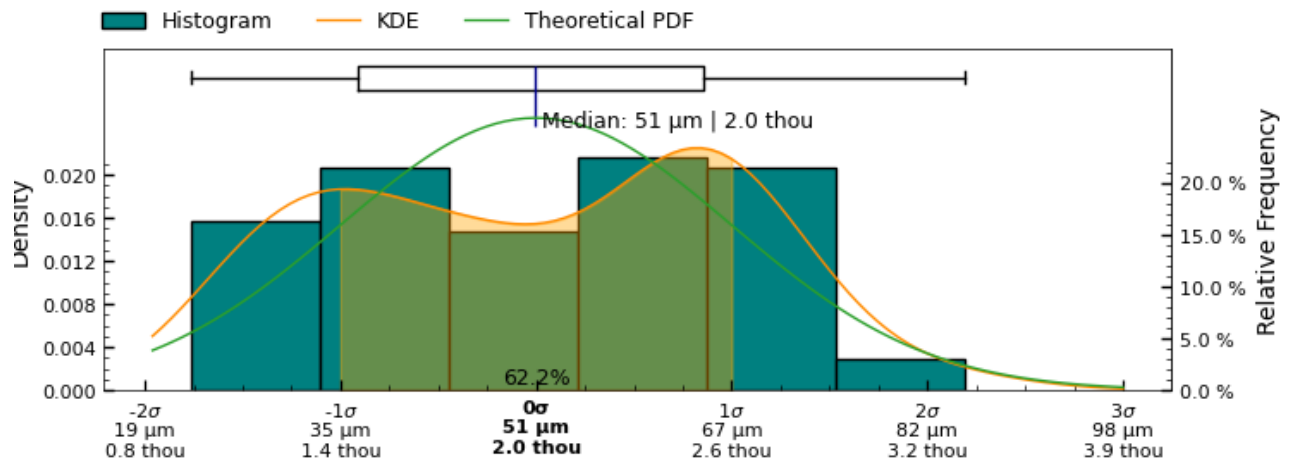
Figure 27: Standard Deviation measurement distribution across measured slices of '+' interior_separate '+' surface
