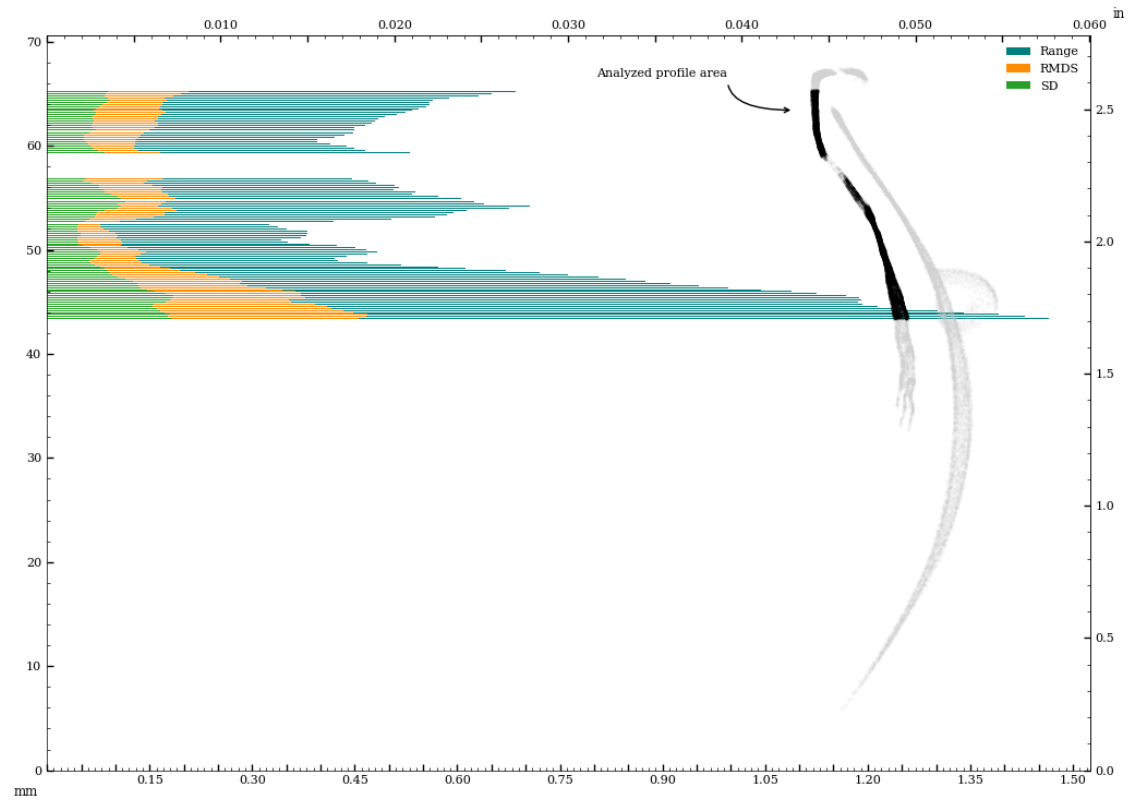
Figure 66: Circularity of interior surface - perpendicular to surface curvature.
