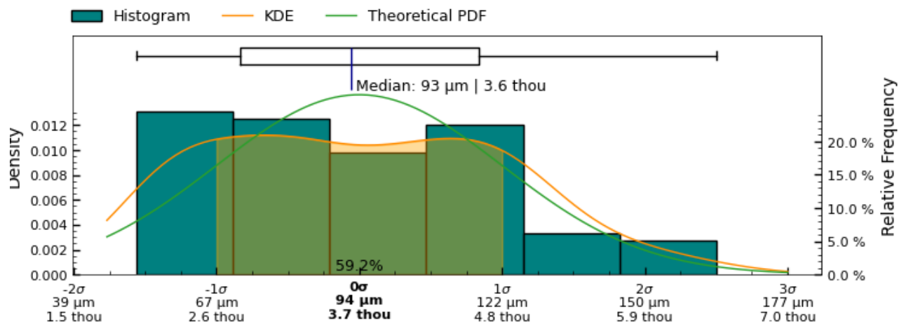
Figure 28: Root Mean Squared Deviation measurement distribution across measured slices of interior separately aligned surface
