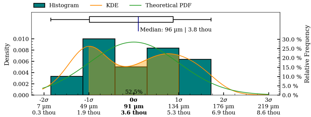
Figure 41: Coaxiality residual plots of interior surface, MV020c.
