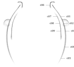
Figure 84: Circularity measurement sample locations, full mesh aligned to exterior surface
