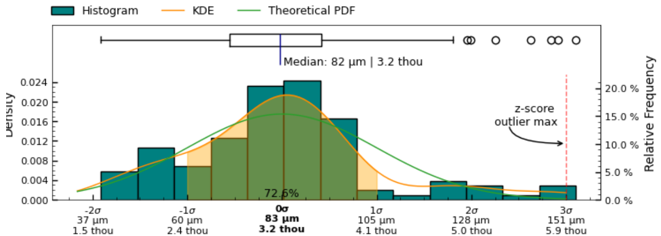
Figure 27: Standard Deviation measurement distribution across measured slices of "+ interior +" surface
