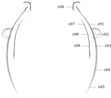
Figure 68: Circularity measurement sample locations, full mesh aligned to exterior surface
