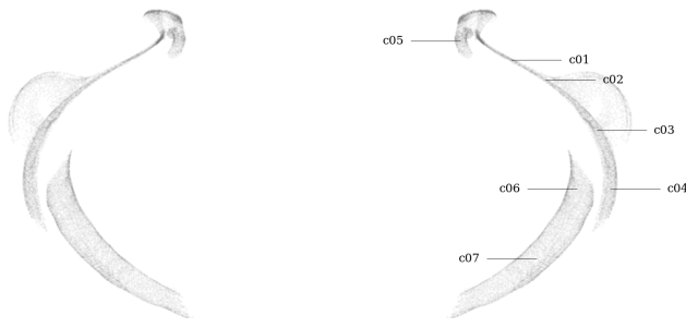
Figure 78: Circularity measurement sample locations, full mesh aligned to exterior surface
