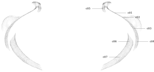
Figure 62: Circularity measurement sample locations, full mesh aligned to exterior surface
