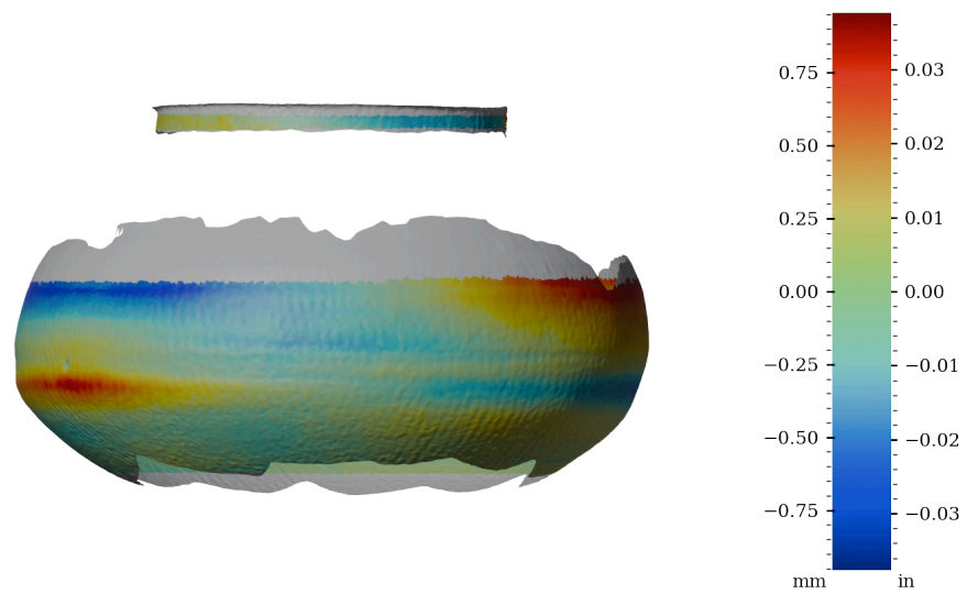
Figure 60: Surface variability heatmap of MV025b, rotated 270°
