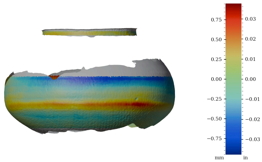
Figure 59: Surface variability heatmap of MV025b, rotated 180°
