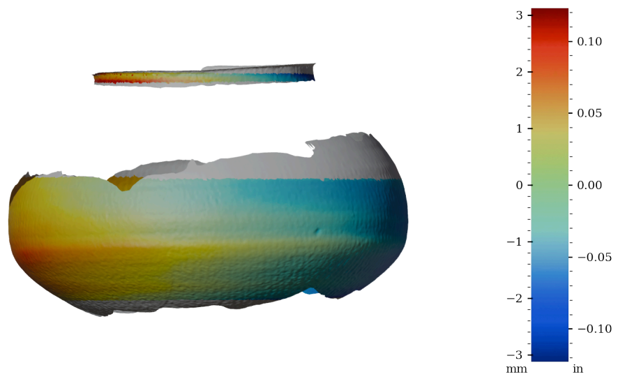
Figure 55: Surface variability heatmap of MV025b, rotated 180°
