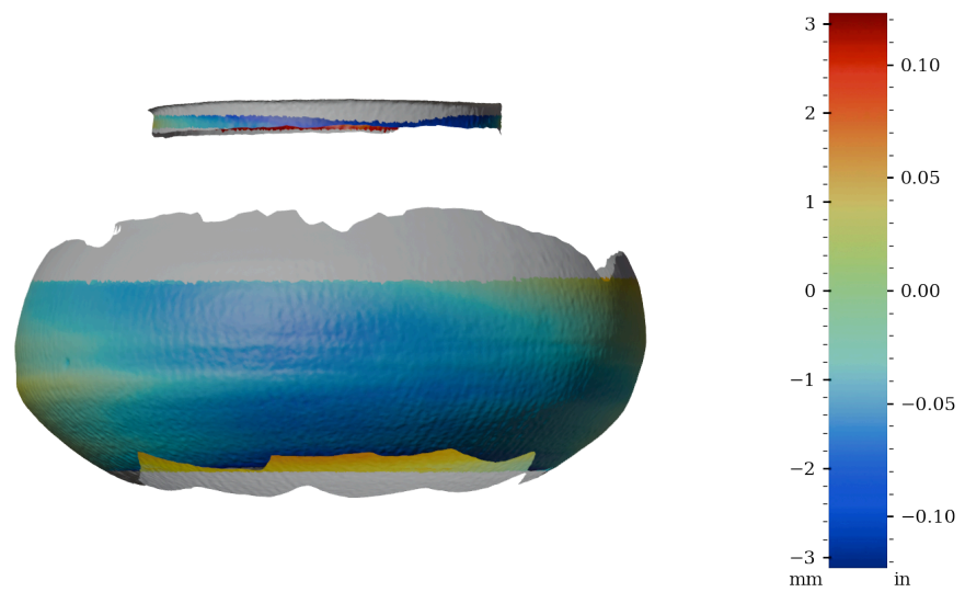
Figure 56: Surface variability heatmap of MV025b, rotated 270°
