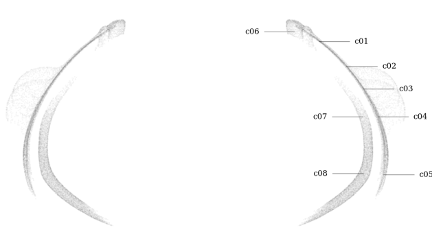
Figure 66: Circularity measurement sample locations, full mesh aligned to exterior surface
