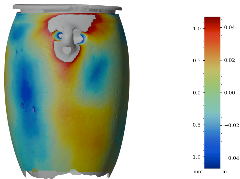
Figure 46: Surface variability heatmap of MV029, rotated 90°
