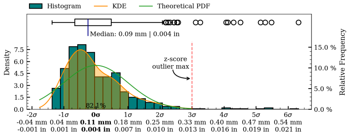
Figure 42: Coaxiality residual plots of exterior surface, MV029.
