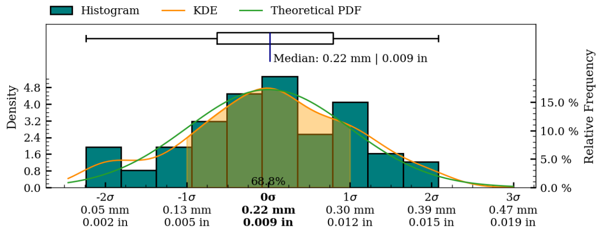
Figure 43: Coaxiality residual plots of interior surface, MV029.
