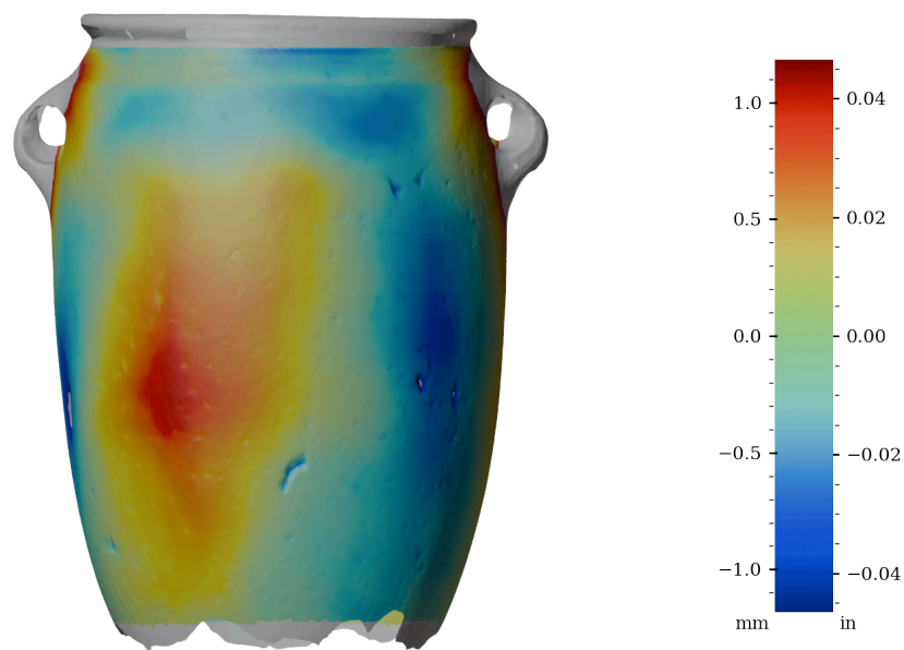
Figure 45: Surface variability heatmap of MV029, front view
