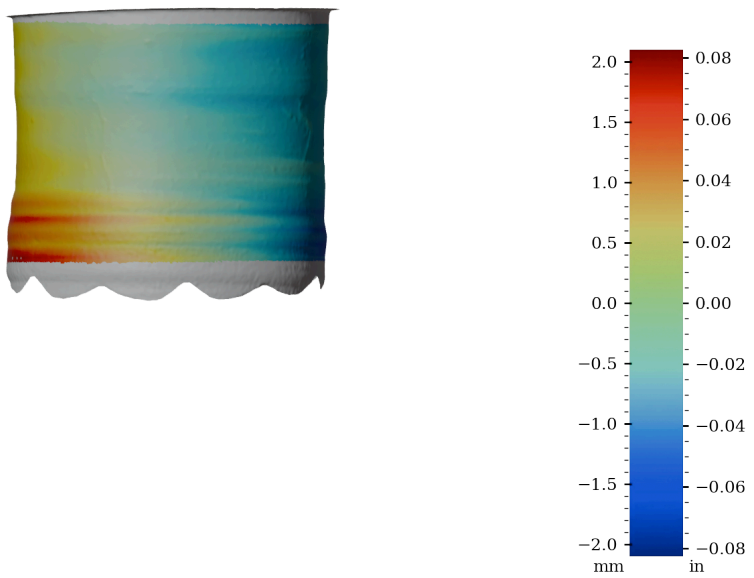
Figure 52: Surface variability heatmap of MV029, rotated 270°
