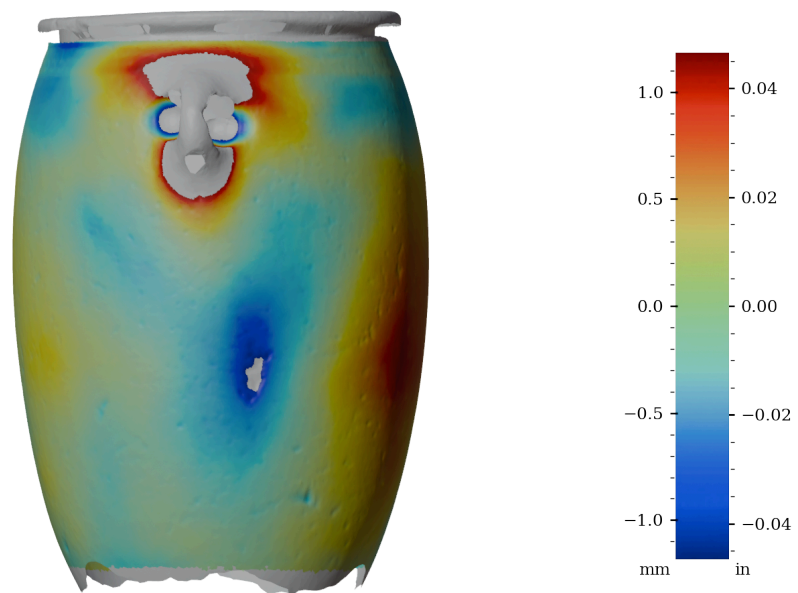
Figure 48: Surface variability heatmap of MV029, rotated 270°
