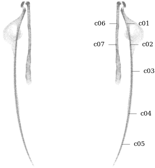
Figure 62: Circularity measurement sample locations, full mesh aligned to exterior surface
