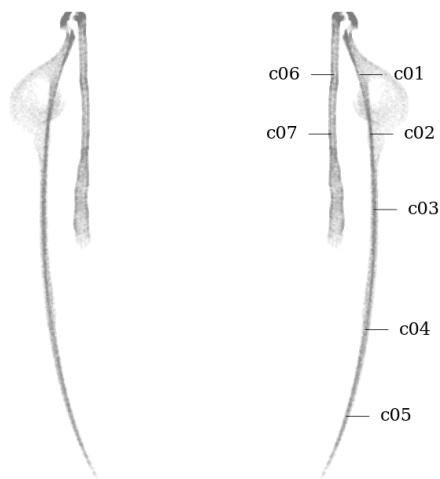
Figure 78: Circularity measurement sample locations, full mesh aligned to exterior surface
