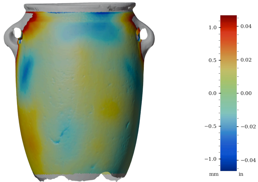
Figure 47: Surface variability heatmap of MV029, rotated 180°
