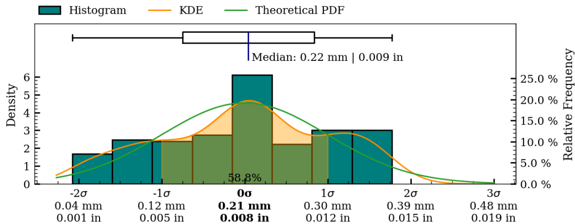
Figure 44: Coaxiality residual plots of interior_separate surface, MV029.
