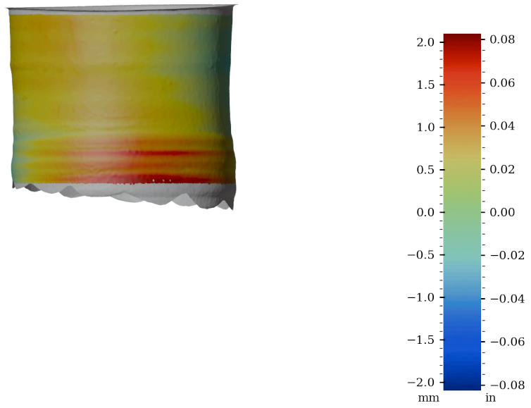
Figure 51: Surface variability heatmap of MV029, rotated 180°
