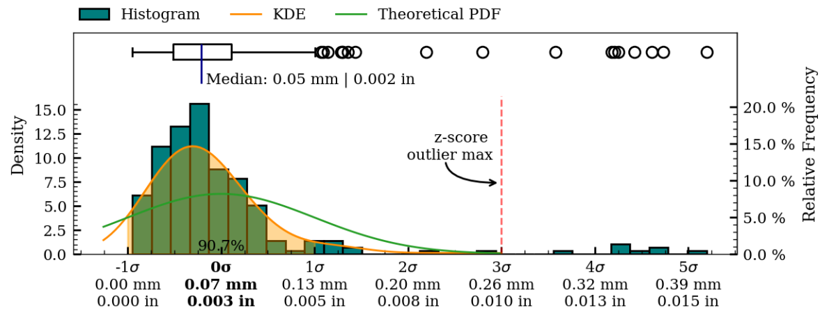
Figure 42: Coaxiality residual plots of exterior surface, MV032.
