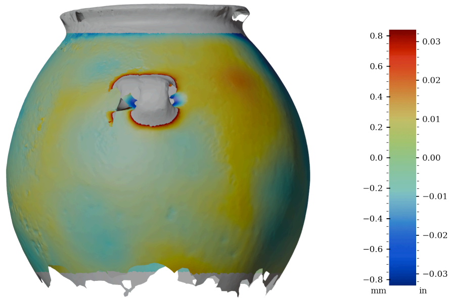
Figure 48: Surface variability heatmap of MV032, rotated 270°
