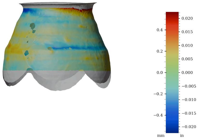
Figure 55: Surface variability heatmap of MV032, rotated 180°
