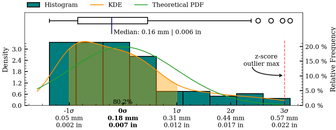
Figure 43: Coaxiality residual plots of interior surface, MV032.
