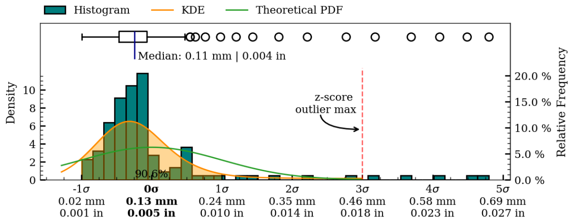
Figure 44: Coaxiality residual plots of interior_separate surface, MV032.
