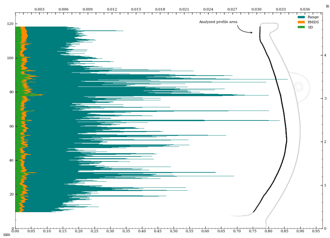
Figure 74: Circularity of interior_separate surface - perpendicular to surface curvature.
