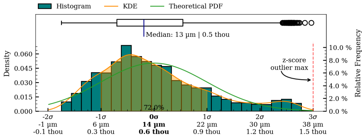
Figure 46: Coaxiality residual plots of interior_separate surface, PV001.
