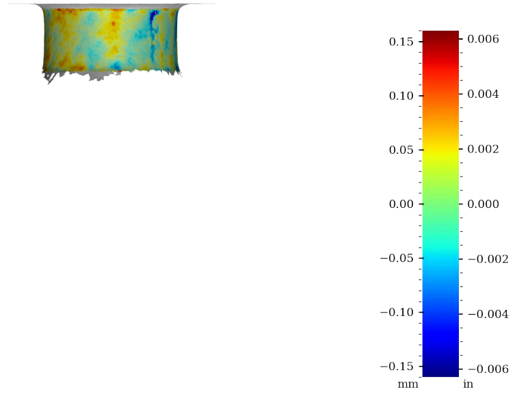
Figure 51: Surface variability heatmap of PV006, rotated 180°
