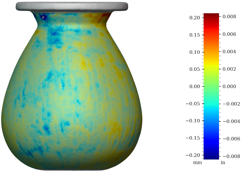
Figure 41: Surface variability heatmap of PV006, front view
