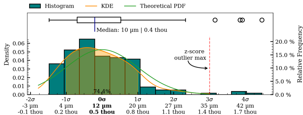
Figure 39: Coaxiality residual plots of interior surface, PV006.
