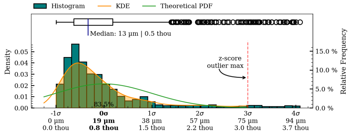
Figure 38: Coaxiality residual plots of exterior surface, PV006.
