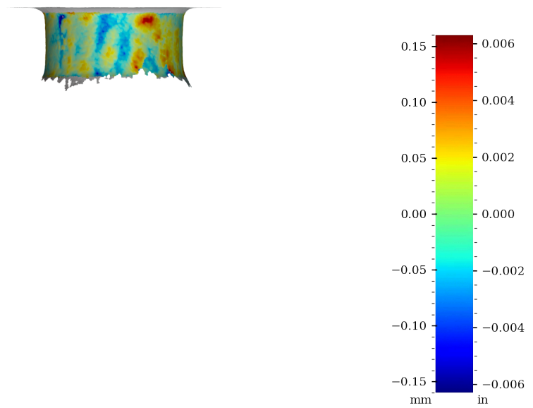
Figure 52: Surface variability heatmap of PV006, rotated 270°
