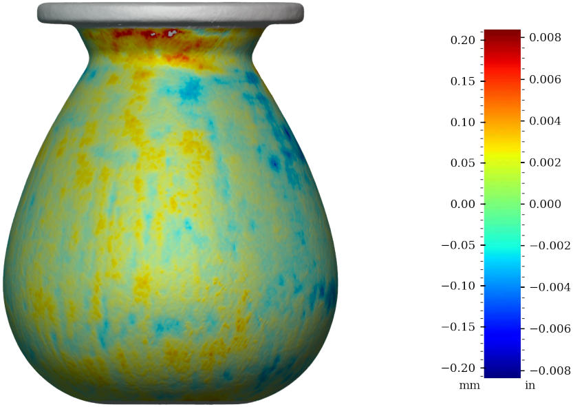
Figure 42: Surface variability heatmap of PV006, rotated 90°
