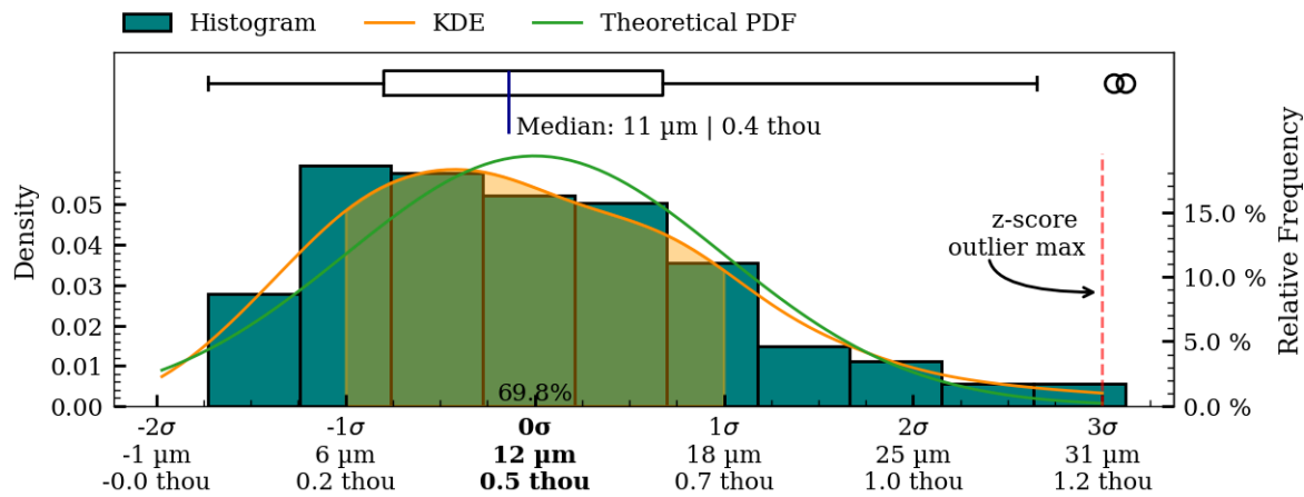
Figure 40: Coaxiality residual plots of interior_separate surface, PV006.
