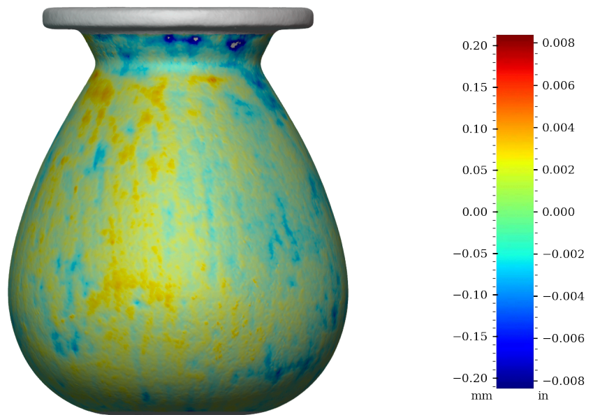
Figure 44: Surface variability heatmap of PV006, rotated 270°
