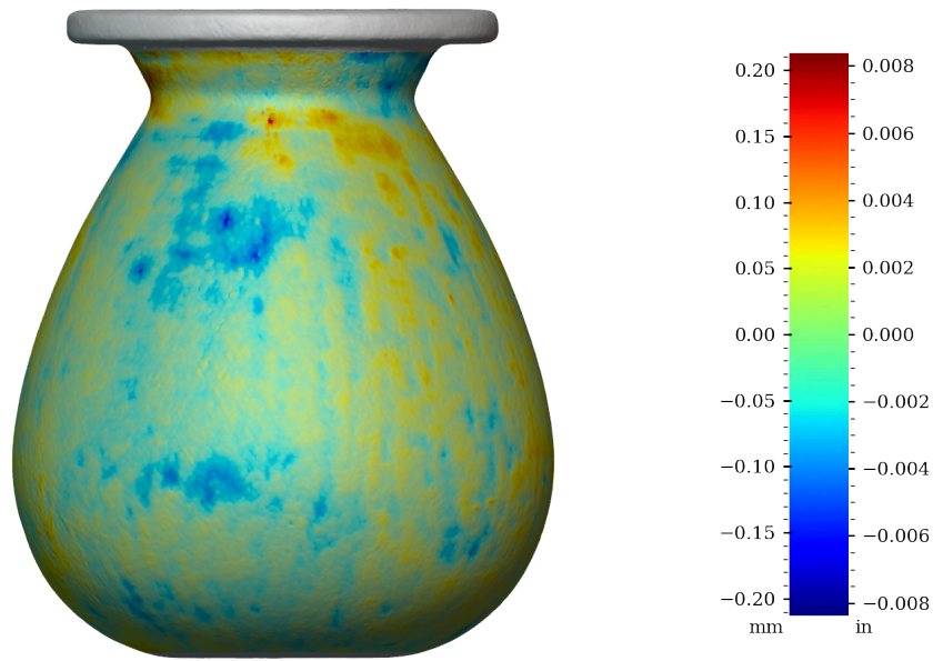
Figure 43: Surface variability heatmap of PV006, rotated 180°
