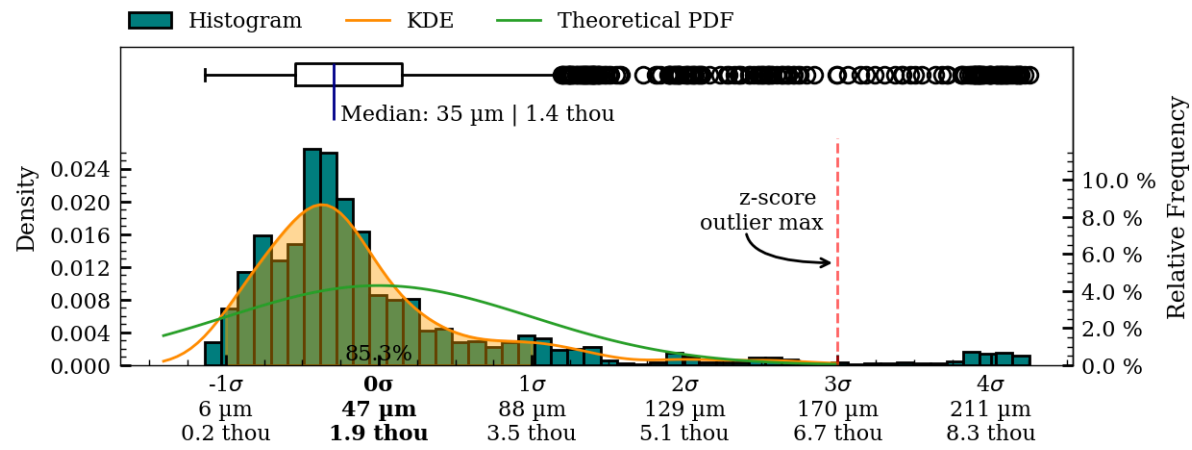
Figure 35: Coaxiality residual plots of exterior surface, RV001.
