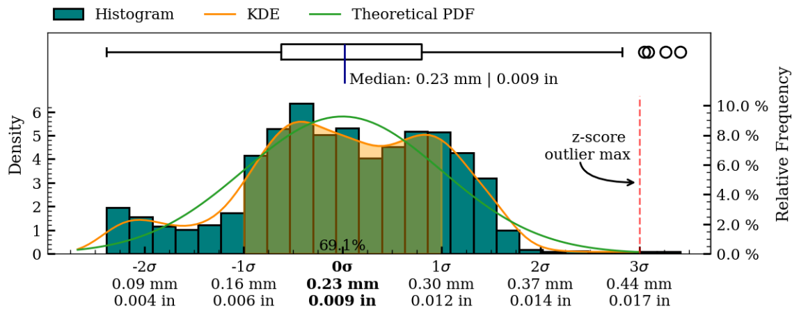
Figure 36: Coaxiality residual plots of interior surface, RV001.
