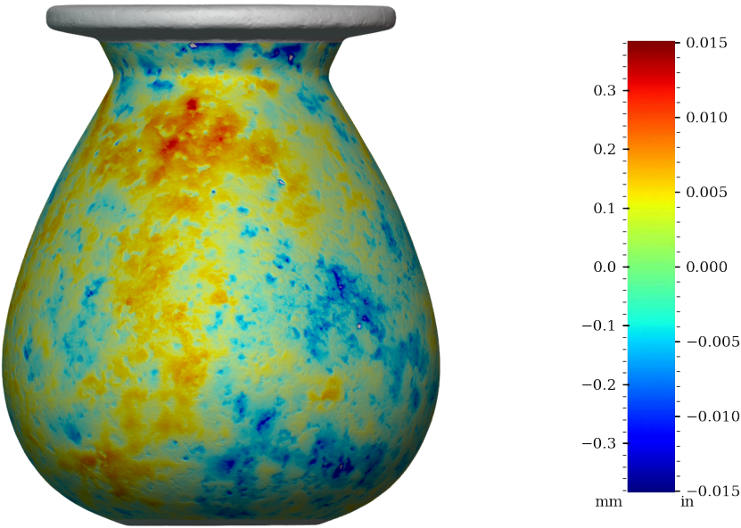
Figure 37: Surface variability heatmap of RV001, front view
