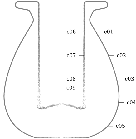
Figure 25: Concentricity measurement sample location on RV001.
