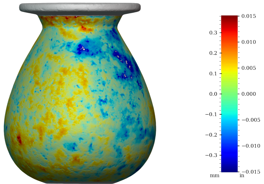
Figure 39: Surface variability heatmap of RV001, rotated 180°
