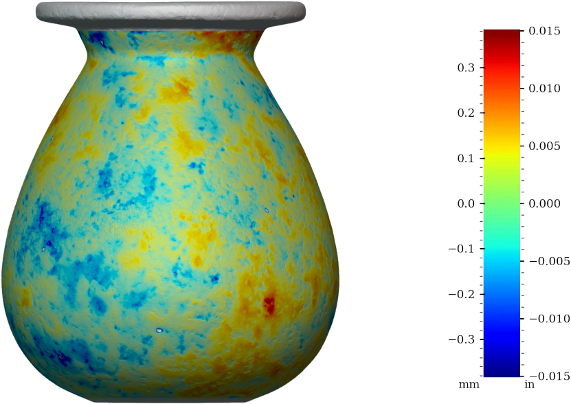
Figure 38: Surface variability heatmap of RV001, rotated 90°
