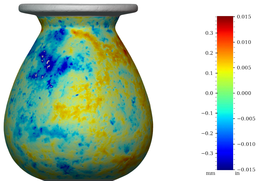
Figure 40: Surface variability heatmap of RV001, rotated 270°
