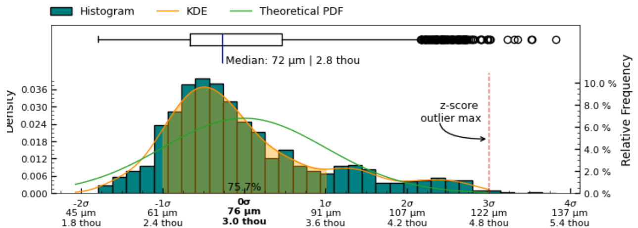
Figure 18: Median absolute deviation measurement distribution across measured slices of exterior surface
