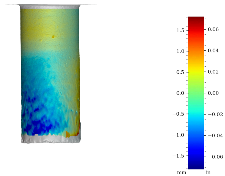
Figure 64: Surface variability heatmap of RV001, rotated 270°
