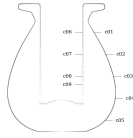
Figure 84: Circularity measurement sample locations, full mesh aligned to exterior surface
