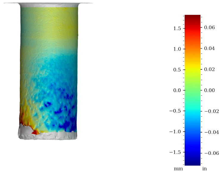
Figure 63: Surface variability heatmap of RV001, rotated 180°
