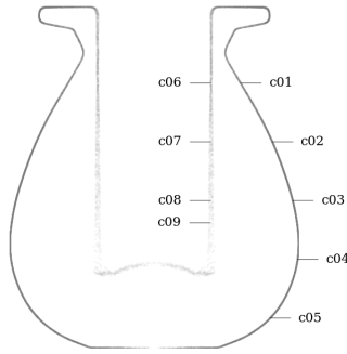
Figure 68: Circularity measurement sample locations, full mesh aligned to exterior surface
