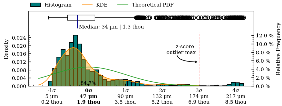
Figure 50: Coaxiality residual plots of exterior surface, RV001.
