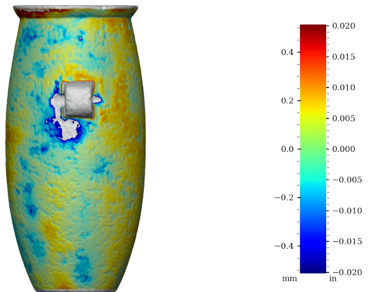
Figure 34: Surface variability heatmap of RV002, rotated 270°
