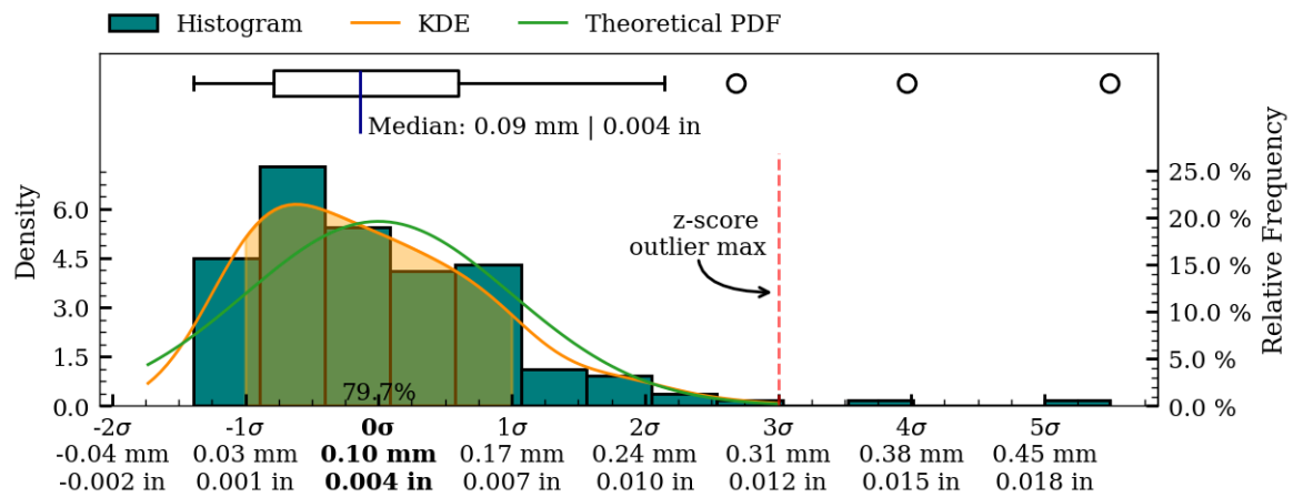
Figure 30: Coaxiality residual plots of interior surface, RV002.
