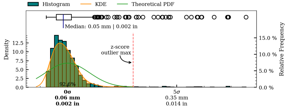
Figure 29: Coaxiality residual plots of exterior surface, RV002.
