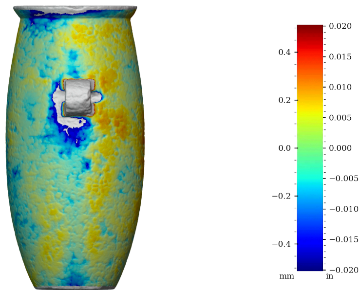
Figure 32: Surface variability heatmap of RV002, rotated 90°
